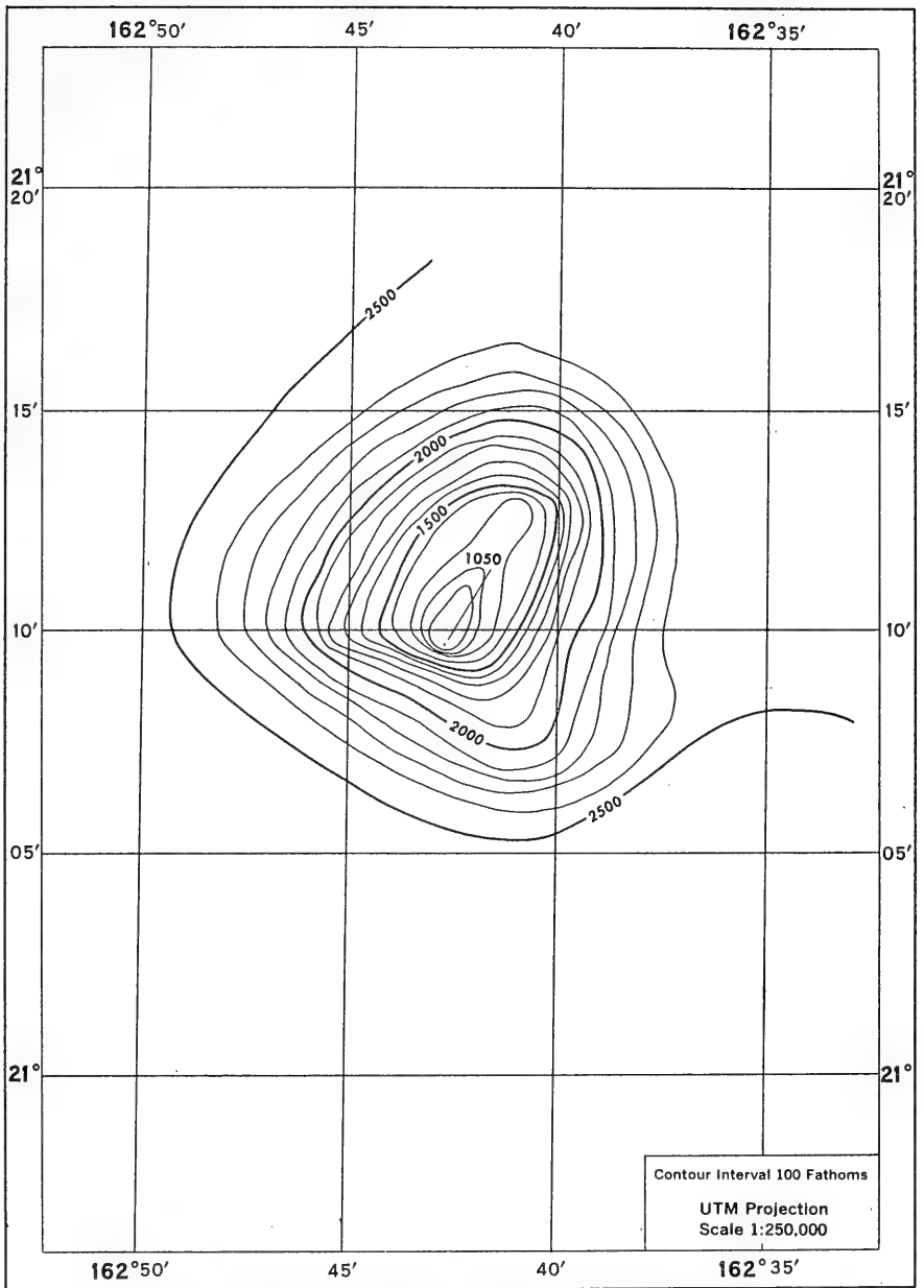
FIGURE 31 DEVELOPMENT AREA 6 BATHYMETRIC CONTOUR CHART
