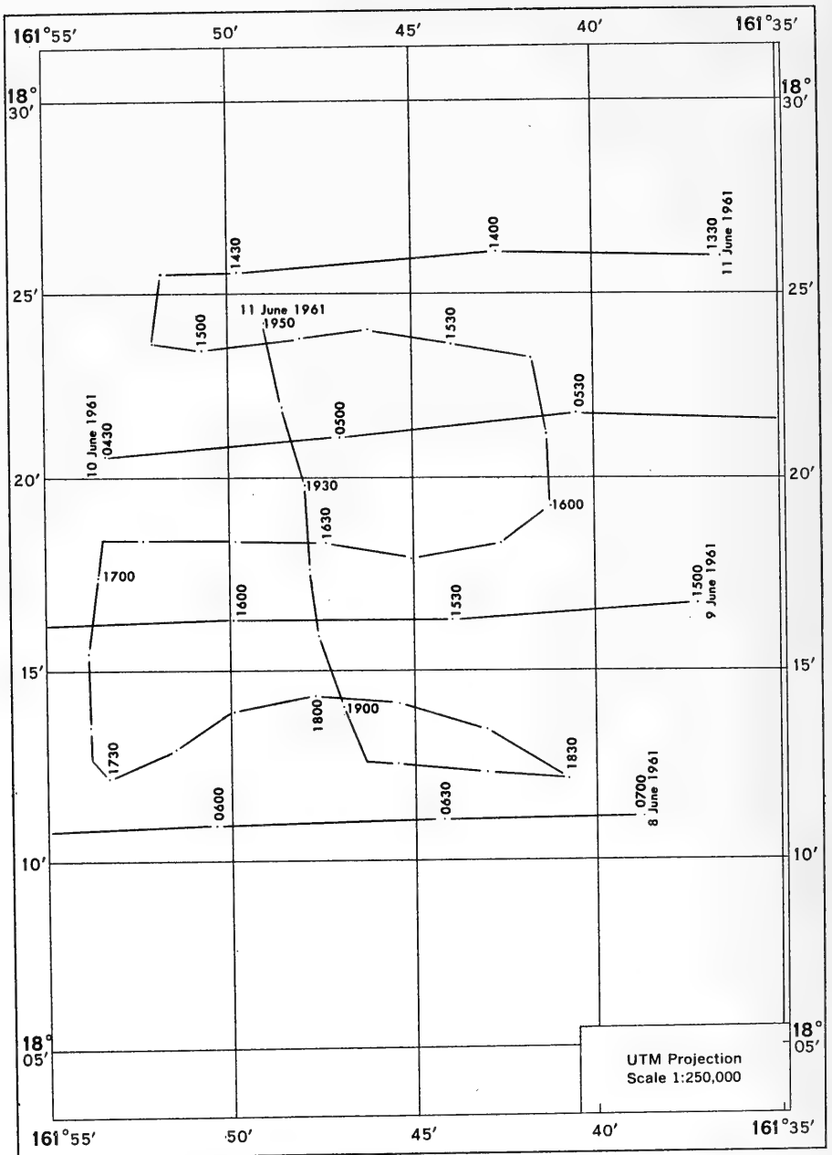
FIGURE 14 DEVELOPMENT AREA 1 TRACK CHART
