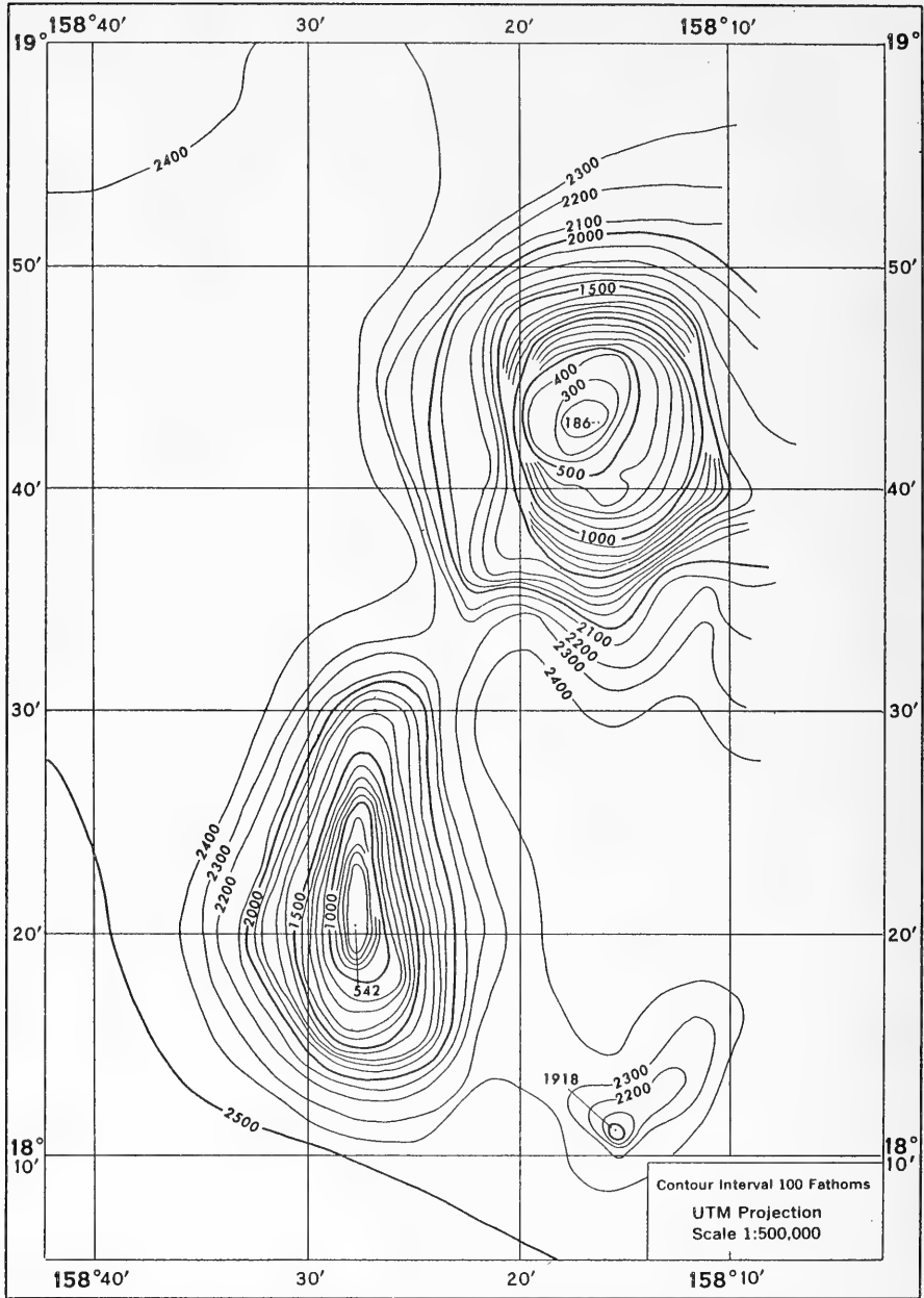
FIGURE 34 DEVELOPMENT AREA 7 BATHYMETRIC CONTOUR CHART
