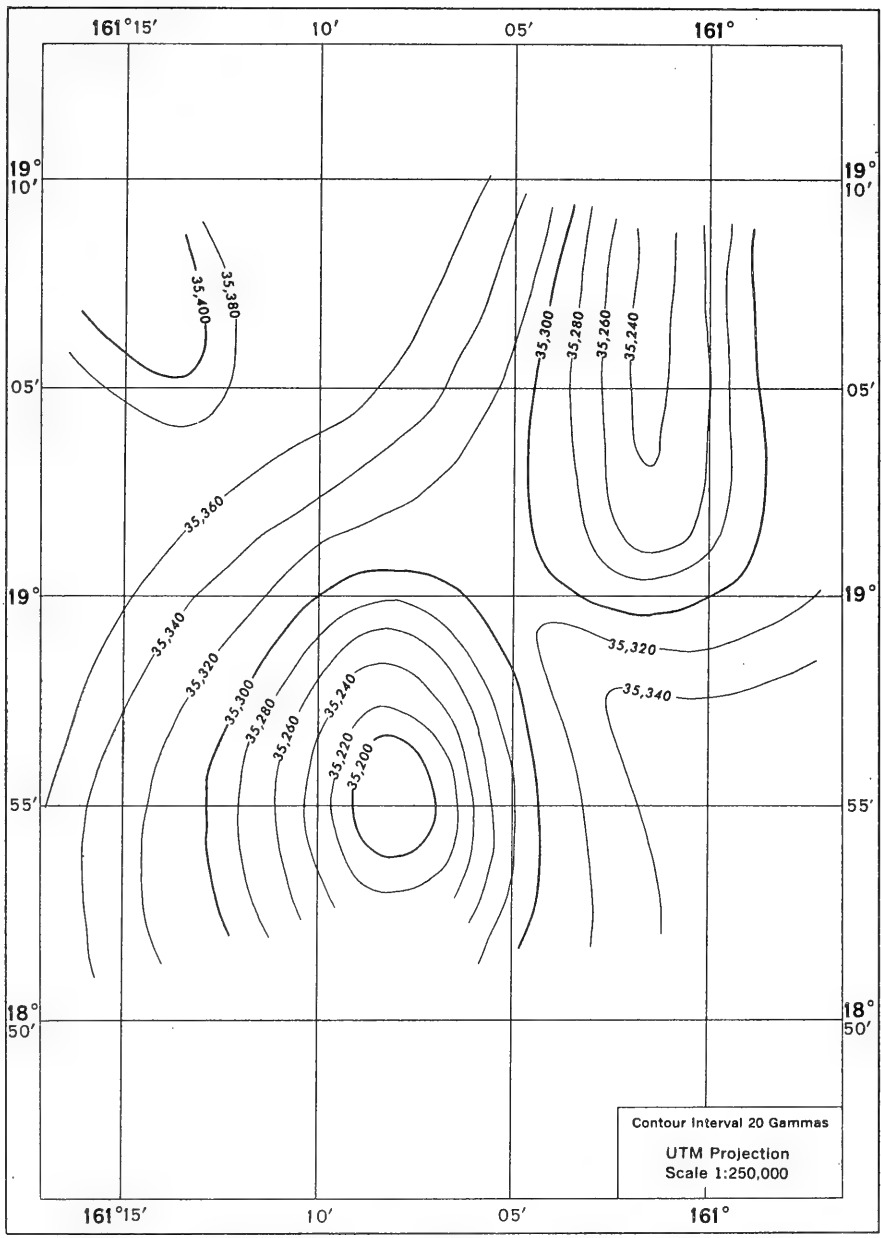
FIGURE 21 DEVELOPMENT AREA 3 MAGNETIC TOTAL INTENSITY CONTOUR CHART
