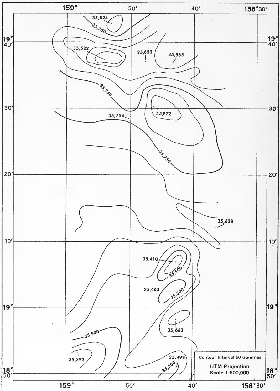
FIGURE 36 DEVELOPMENT AREA 8 MAGNETIC TOTAL INTENSITY CONTOUR CHART
