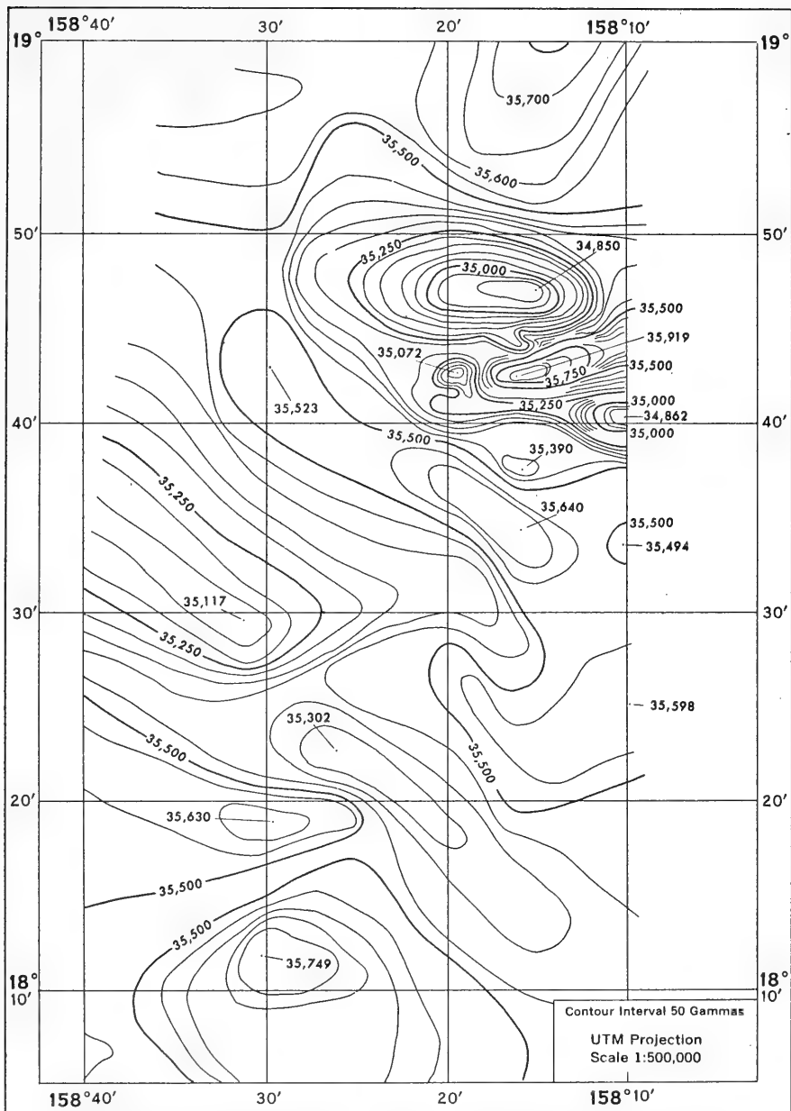
FIGURE 33 DEVELOPMENT AREA 7 MAGNETIC TOTAL INTENSITY CONTOUR CHART
