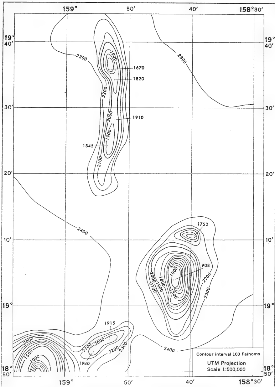
FIGURE 37 DEVELOPMENT AREA 8 BATHYMETRIC CONTOUR CHART
