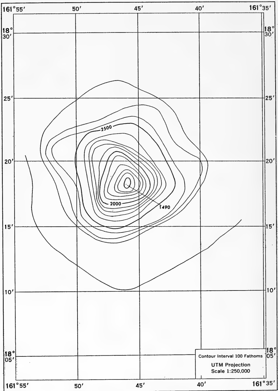
FIGURE 16 DEVELOPMENT AREA 1 BATHYMETRIC CONTOUR CHART
