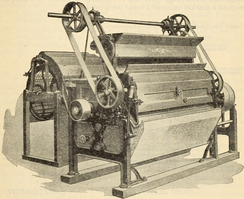
FIG. 2.—A type of machine used in delinting cottonseed
