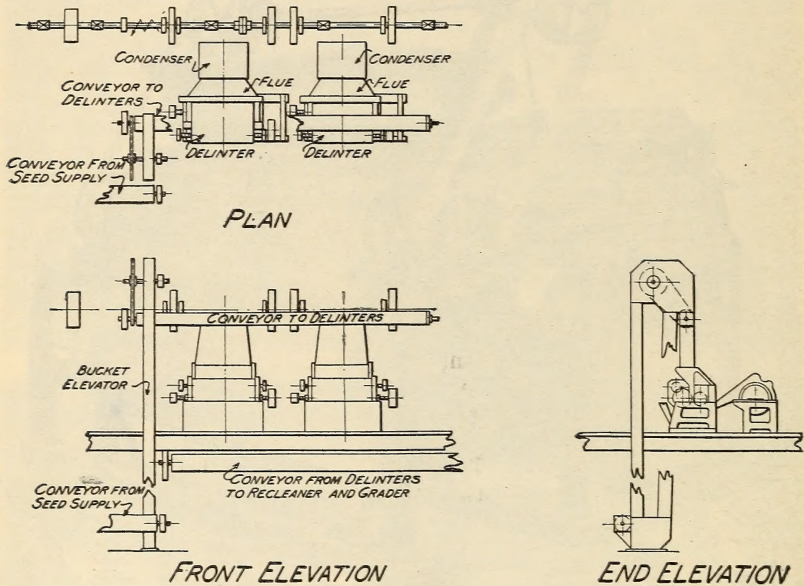
FIG. 3.—General layout or plan of two-unit delinting plant. Note: No attempt is made here to show the details or to suggest a fixed plan of installation. Manufacturers no doubt will be glad to cooperate with prospective buyers in working out the most economical and efficient plan of installing and operating such machinery under varied conditions and for any special requirements
