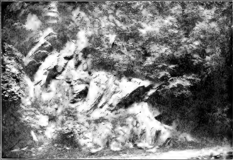
FIG. 2.—VIEW SHOWING THE LOWER PART OF THE CATSKILL FORMATION ON JENNINGS RUN.
