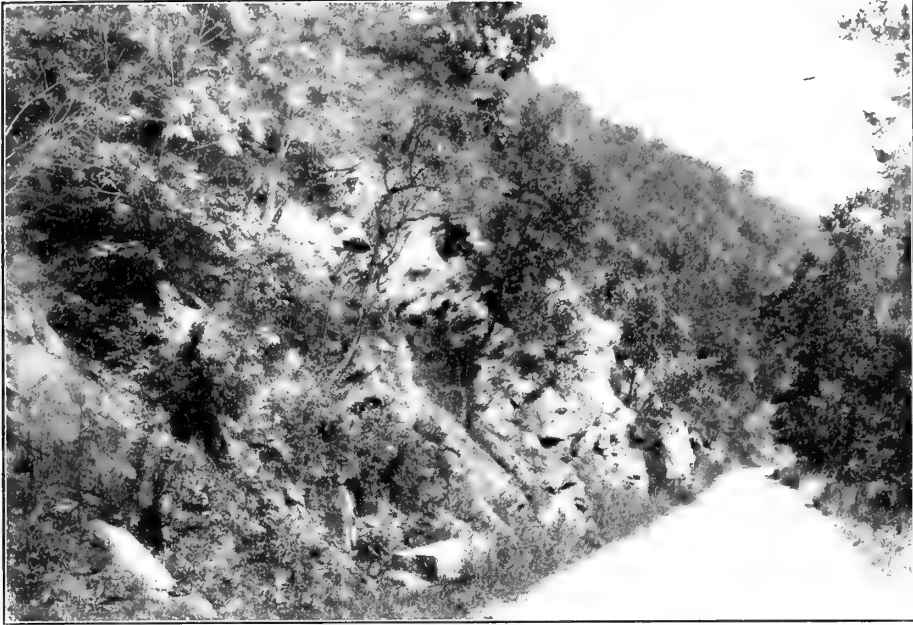
FIG. 1.—VIEW SHOWING THE CATSKILL FORMATION ON JENNINGS RUN ROAD 1 MILE EAST OF BARRELVILLE.
