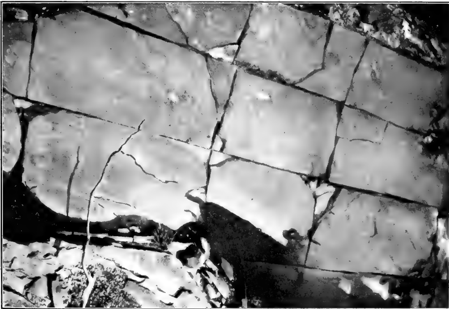
FIG. 2.—VIEW SHOWING RECTILINEAR JOINTING IN THE SANDY SHALE OF THE JENNINGS FORMATION NEAR STOTTLERS CROSSROADS.
