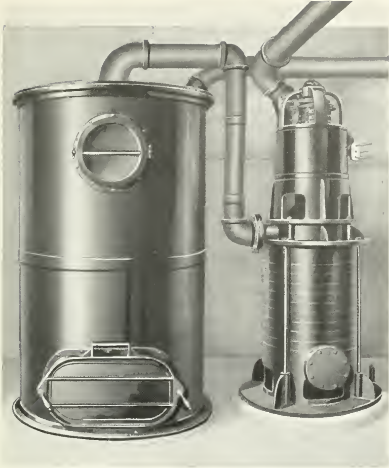
VACUUM CLEANER SYSTEM—SPENCER TURBINE CLEANER CO.
