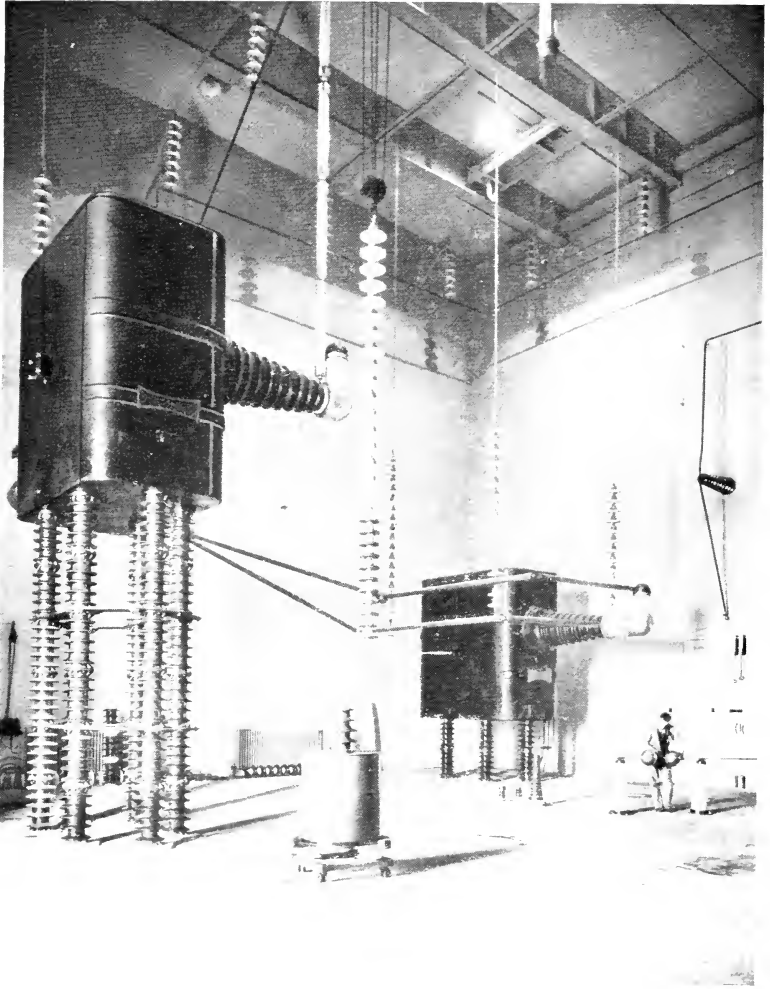
THE 1,000,000-VOLT TESTING TRANSFORMER IN THE RESEARCH LABORATORY AT STOURPORT
