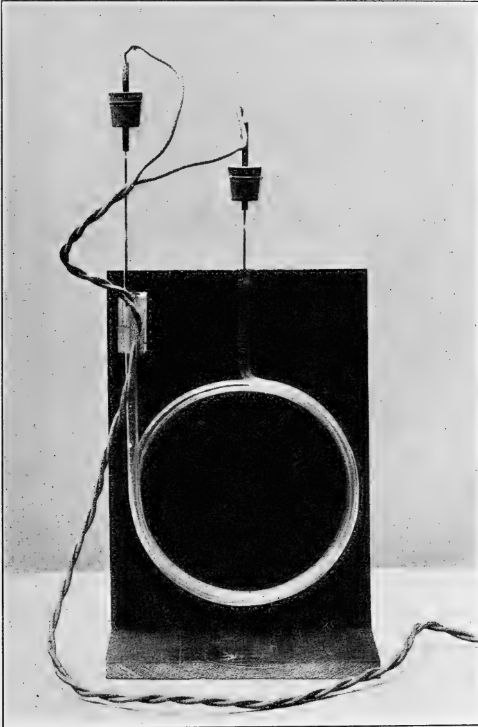
FIG. 7.—Electrolytic cell used for preliminary measurements of resistance of sea-water samples of various salinities
