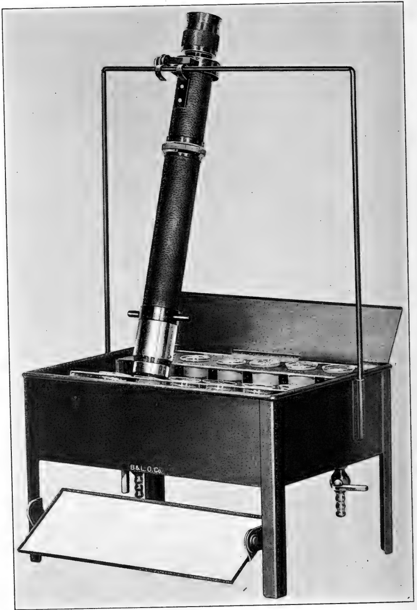
FIG. 4.—Dipping refractometer
