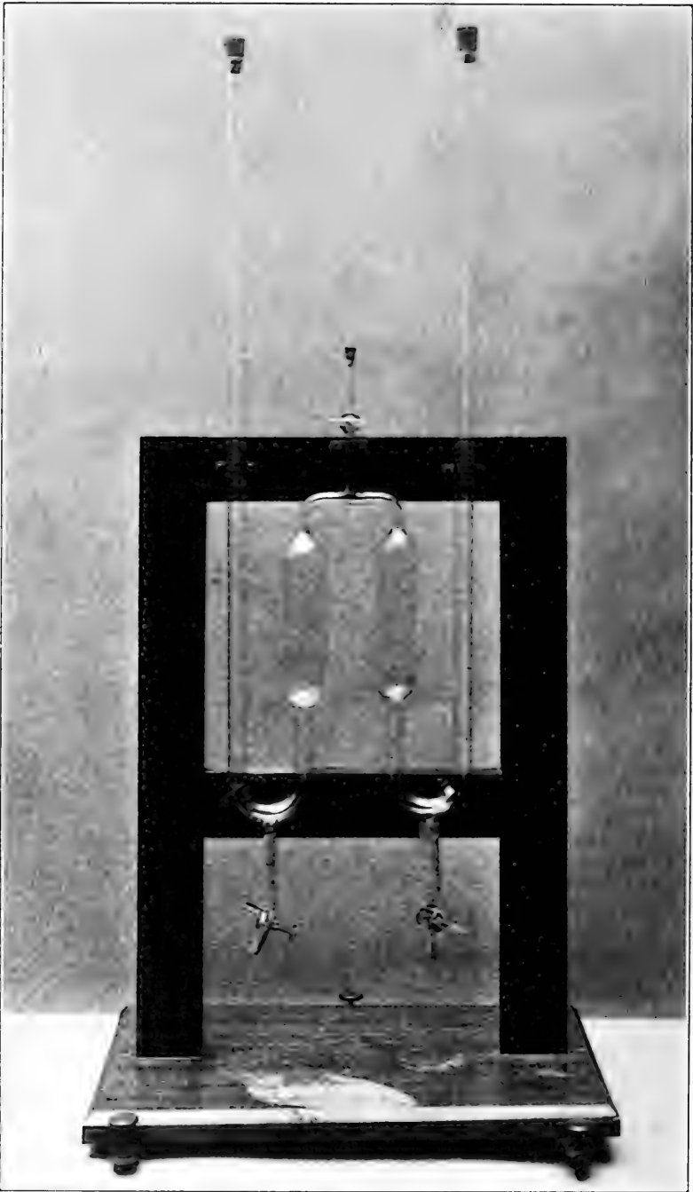
FIG. 8.—Apparatus for measuring salinity by the method of balancing columns of liquids
