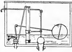
FIG. 84. Diagram of flushing tank.
