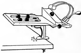
FIG. 108. Cherry stoner.
