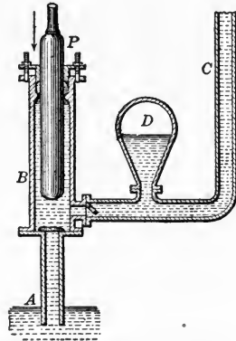
FIG. 69. Force pump.
