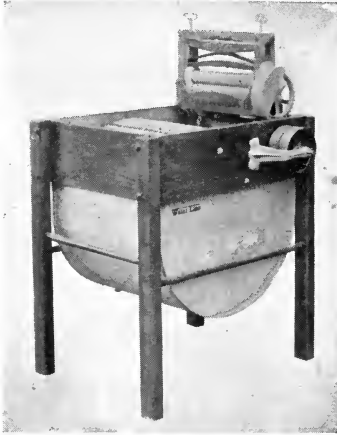
FIG. 88. Cylinder washer.
