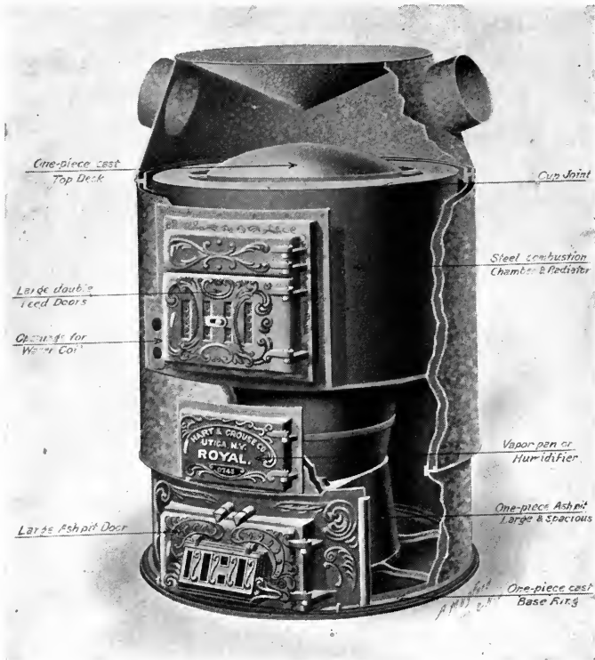
FIG. 26. Warm-air furnace.
