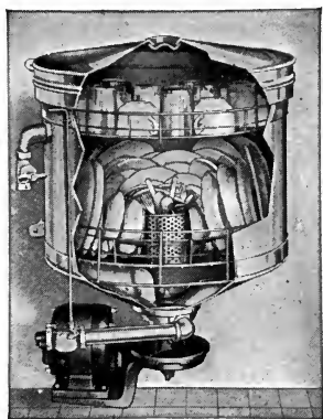
FIG. 119-b. Walker dish-washer.
