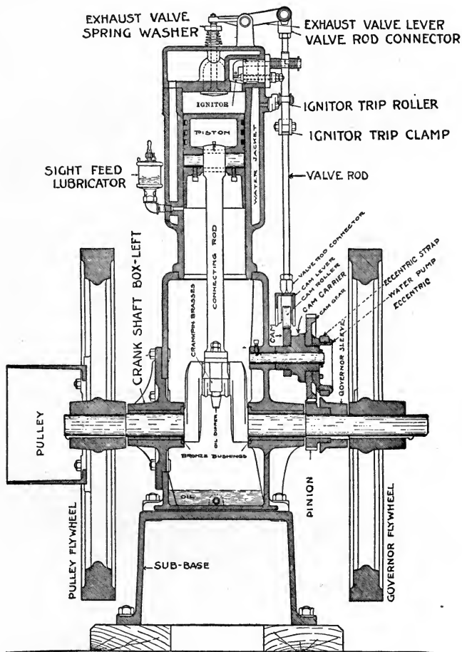
FIG. 151. Sectional view of gasoline engine.
