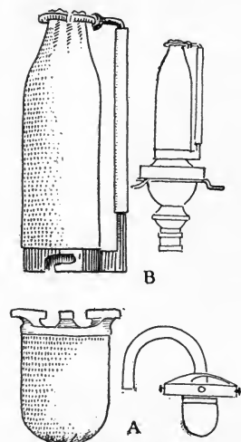
FIG. 48. Mantles.
