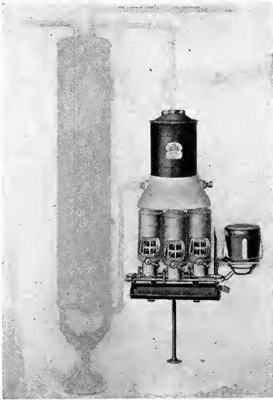
FIG. 74. Water heater and tank. FIG. 75. Booster for hot water.
