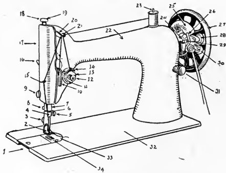
FIG. 132. Lock-stitch machine.
