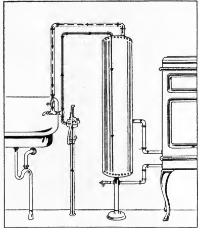
FIG. 73. Force pump and boiler.
