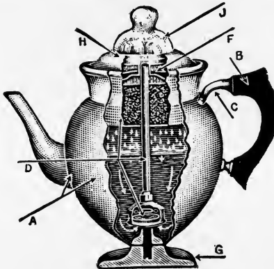
FIG. 118. Percolator.
