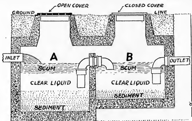
FIG. 82. Details of septic tank.
