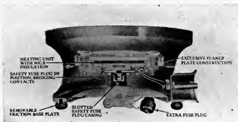
FIG. 20. Heating unit of electric stove.
