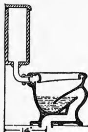
FIG. 83. Section of water closet.
