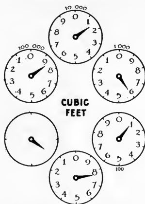
FIG. 159. Water meter.
