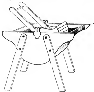
FIG. 90. Oscillating washing machine.
