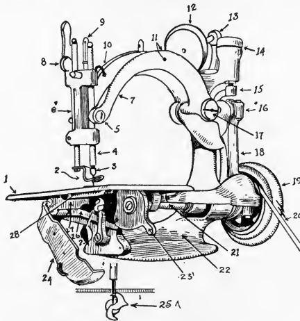
FIG. 138. Chain-stitch machine.
