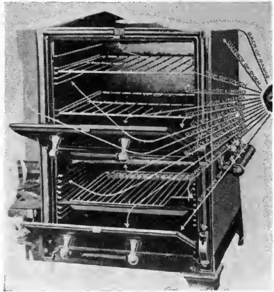
FIG. 7. Gas ovens.
