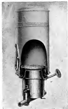
FIG. 13. Burner for oil stove.
