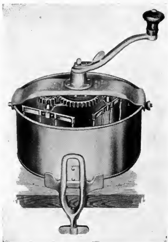
FIG. 116. View showing internal arrangement of cake mixer.
