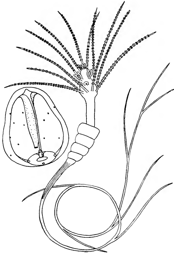
FIG. 3.— Trichorhiza brunnea , after Russell, Proc. Zool. Soc., London, 1906. Hydroid, and enlarged view of recently liberated medusa.
