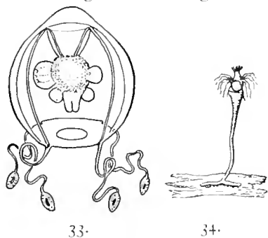
FIG. 33.— Eucodonium brownei , after Browne, in Proc. Zool. Soc. London .
