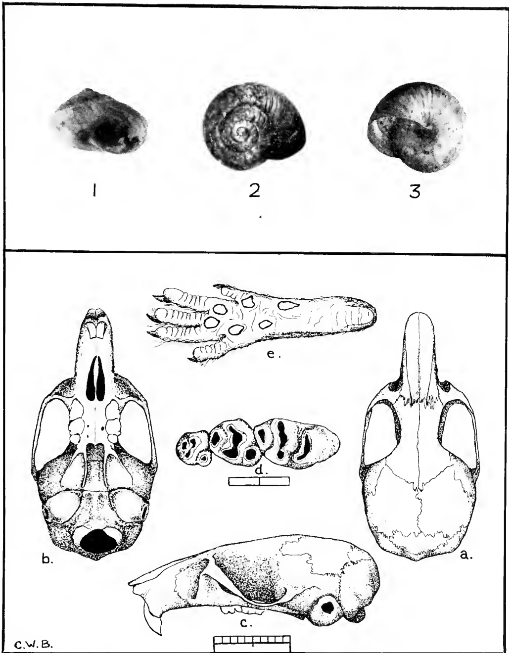
Thalassohelix translucens , sp.n., Figs. 1-3. ? Pseudomys (Gyomys) funceus sp.n., figs. a-e.
