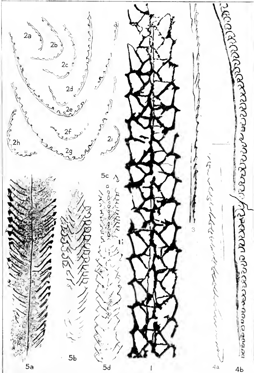
Graptolites
