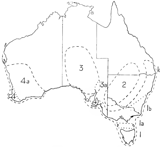
FIG. 1—DISTRIBUTION.
