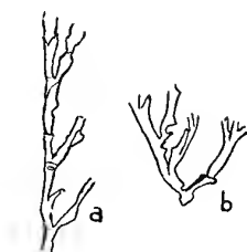
Fig. 4. Pterograptus lyricus , sp. nov. Polyparies bilaterally compressed. a. Proximal portion showing inner branches arising serially (No. 13755 Nat. Mus.). b. Proximal portion (No. 13756 Nat. Mus.). \times 4 . Paratypes, Turner's Quarry, 5 miles W. of Hastings.
