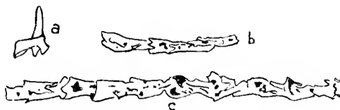
Fig. 2. Tetragraptus decipiens T. S. Hall var. bipatens nov. a. Sicula and theca 1 (No. 25094). b. (?) serrated or irregular apertural margins on branch of second order (No. 25058). c. Proximal portion of branch of second order showing peculiar arrangement of thecae (holotype No. 25094). \times 4 .
