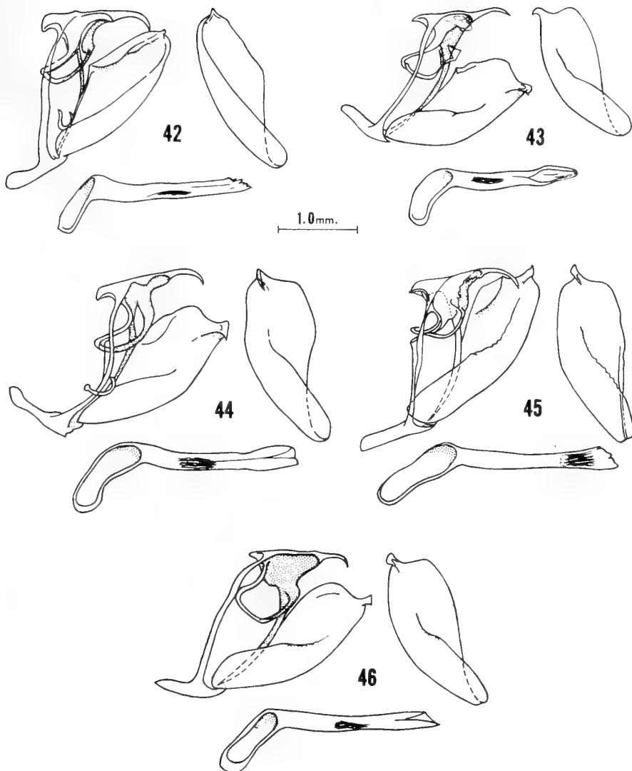
Figs. 42-46, male genitalia of Forbestra species, the penis and dissected left valve shown separately, all drawn to the same scale. Fig. 42, F. e. equicoloides (Godman & Salvin) from Caucayá, Amazonas, Colombia; slide 777, CM. Fig. 43, F. proceris (Weymer) from "Upper Amazon"; slide 780, CM. Fig. 44, F. aeneola new species, holotype from Lago Yarina-Cocha, Loreto, Peru; slide 1198, CM. Fig. 45, F. olivencia (Bates) from Rio Putumayo, Colombia; slide 813, AMNH. Fig. 46, F. t. truncata (Butler) from "Upper Amazon"; slide 774, CM.
