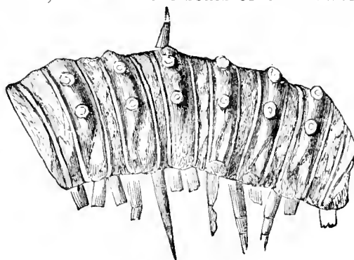
Fig. 5. Acautherpestes major .
