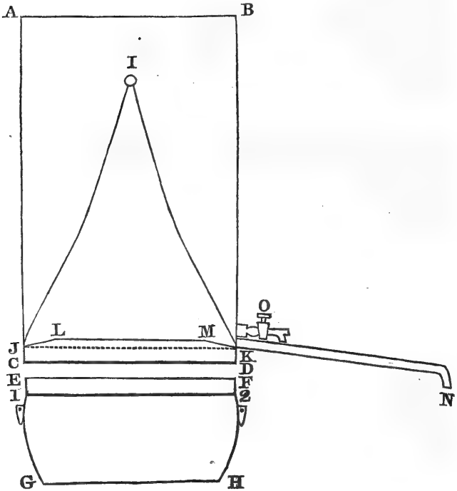
A, B, C, D, Tin iron-stand for the cold water, and fitting closely on E, F, G, H, the copper or boiling-pan, I, J, K, condenser, L, M, J, K, receiver of condensed spirits, K, N, rod for conducting off the spirits, O, cock for shifting water in the stand.
