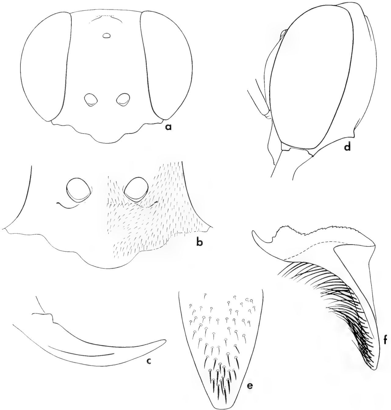
FIGURE 65 Gastrosericus lepidus : a, female head ( \times 32 ), b, female clypeus ( \times 42 ), c, female mandible ( \times 54 ), d, female head laterally ( \times 38 ), e, female pygidial plate ( \times 52 ), f, volsella ( \times 220 )
