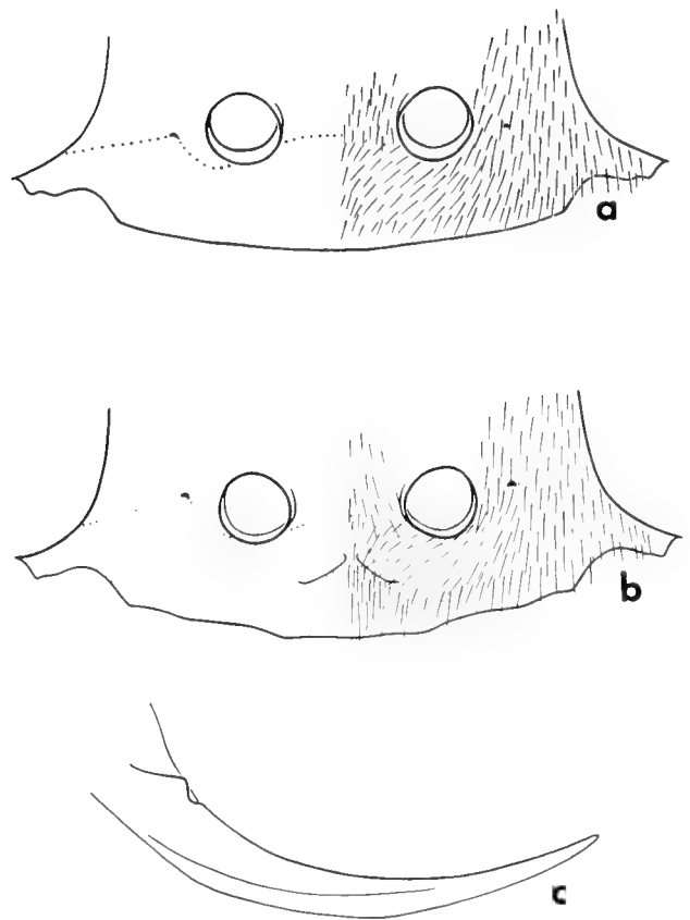
FIGURE 12. Gastrosericus attenuatus , female: a, noncarnate clypeus ( \times 44 ), b, carnate clypeus ( \times 44 ); c, mandible ( \times 41 ).
