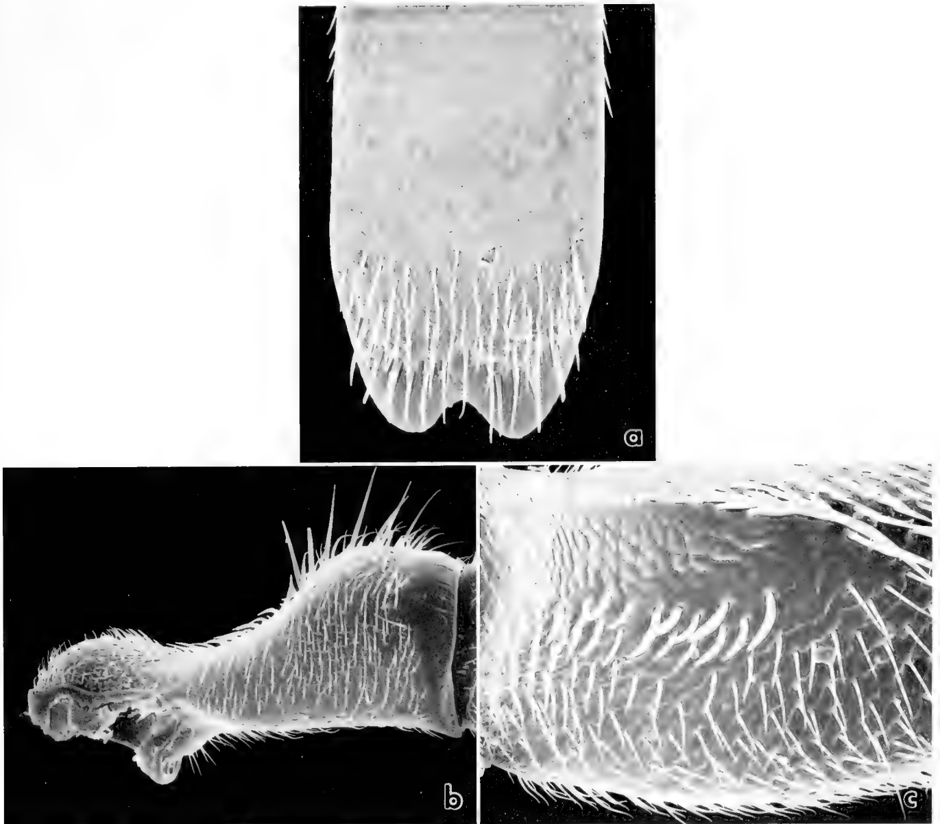
FIGURE 132. Gastrosericus tuberculatus : a, male sternum VIII, ventral view ( \times 31 ); b, male foretrochanter ( \times 103 ); c, bottom of foretrochanteral notch ( \times 205 ).
