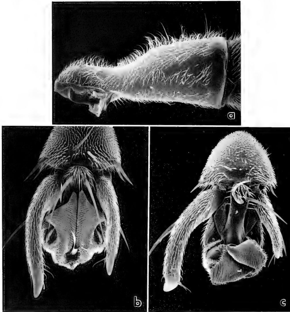
FIGURE 98. Gastrosericus rothneyi : a, male foretrochanter ( \times 199 ); b, claws of female hindtarsomere V ( \times 167 ); c, claws of male hindtarsomere V ( \times 210 ).
