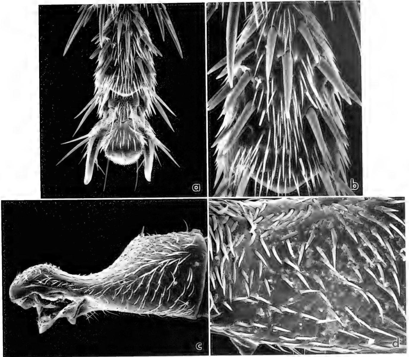
FIGURE 55. Gastrosericus hombori : a, female hindtarsomere V ventrally ( \times 237 ); b, same ( \times 474 ); c, foretrochanteral notch of male ( \times 356 ); d, bottom of trochanteral notch ( \times 798 )
