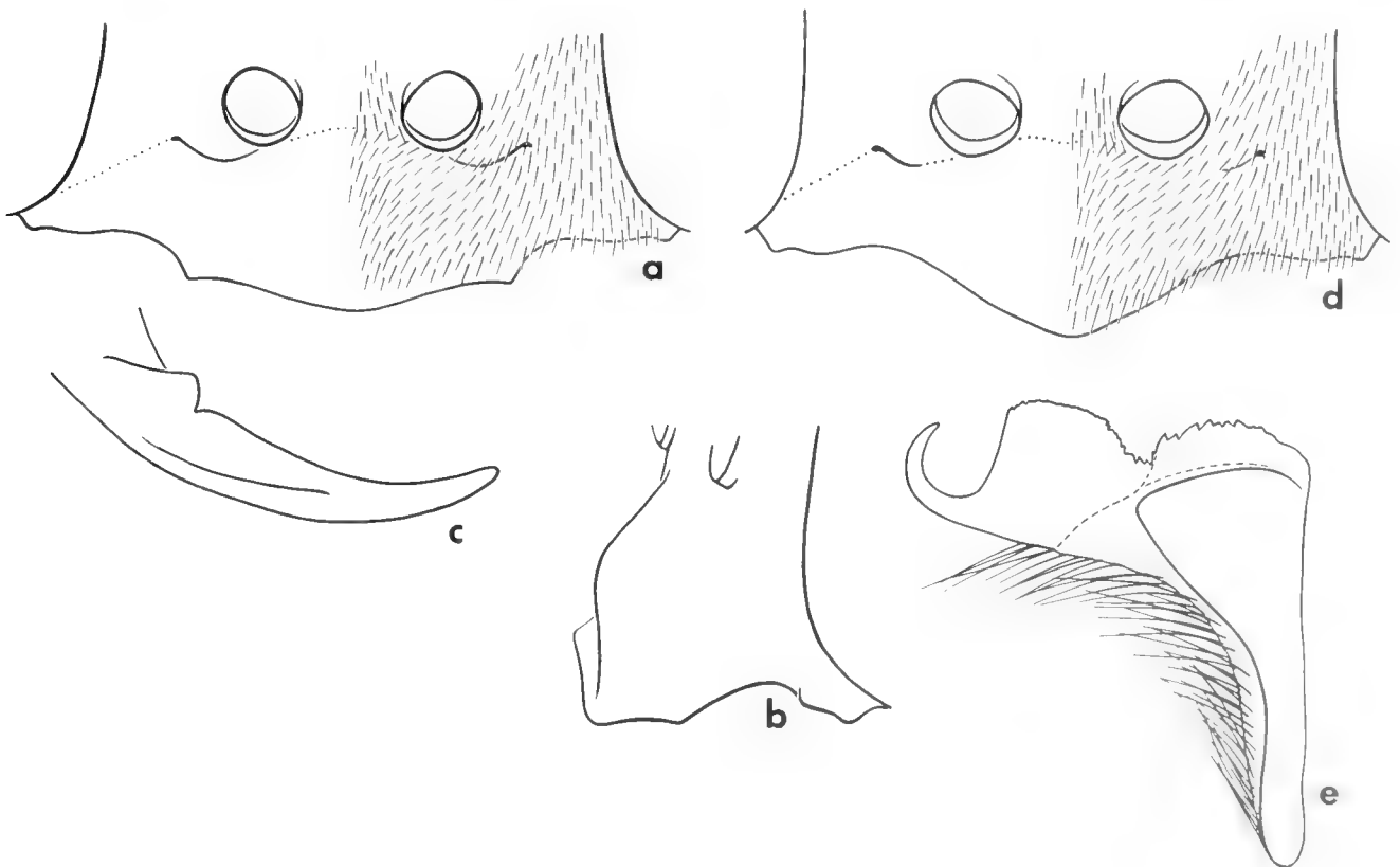
FIGURE 27. Gastrosericus chalcithorax : a, female clypeus frontally ( \times 66 ); b, female clypeus obliquely from the side showing median swelling ( \times 99 ); c, female mandible ( \times 69 ); d, male clypeus ( \times 82 ); e, volsella ( \times 314 ).
