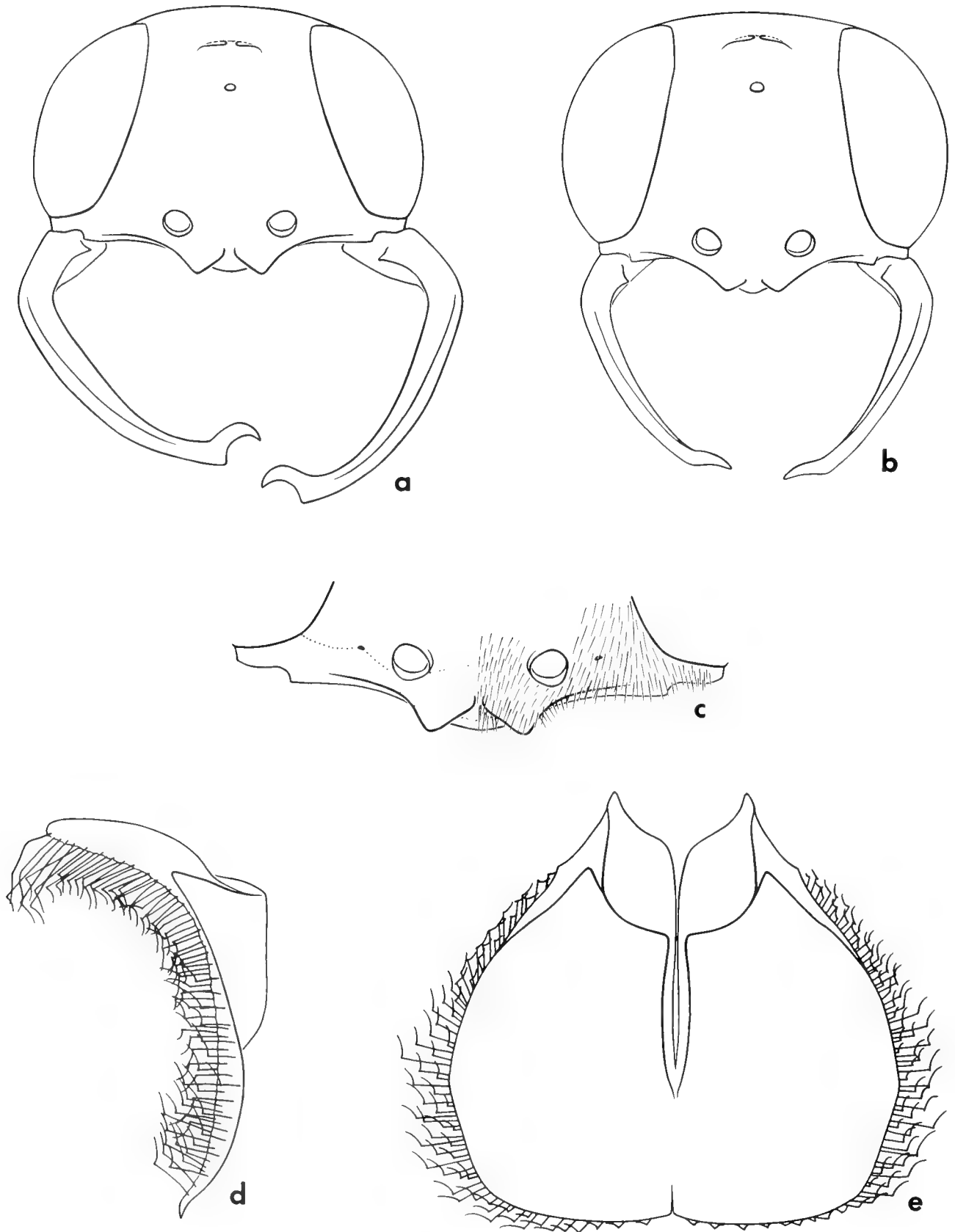
FIGURE 13 Gastrosericus attenuatus , male. a, head of a large specimen ( \times 26 ), b, head of a small specimen ( \times 32 ); c, clypeus ( \times 49 ); d, volsella laterally ( \times 204 ), e, volsella dorsally ( \times 204 )
