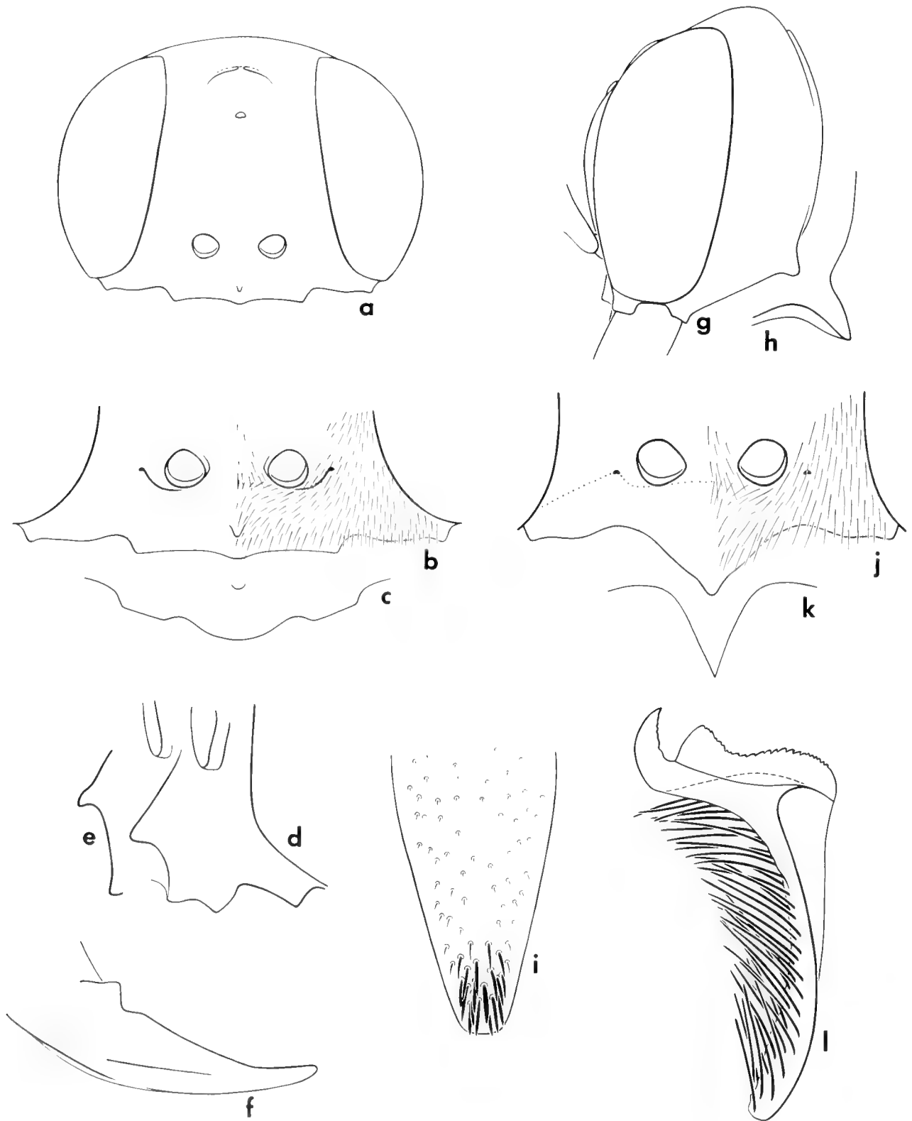
FIGURE 131. Gastroseius tuberculatus . a, female head frontally ( \times 25 ); b, female clypeus ( \times 39 ); c, outline of female clypeus showing individual variation ( \times 55 ); d, female clypeus obliquely ( \times 110 ); e, outline of a female clypeus obliquely showing individual variation ( \times 55 ); f, female mandible ( \times 54 ); g, female head laterally ( \times 29 ); h, genal tooth of female showing individual variation ( \times 23 ); i, female pygidial plate ( \times 49 ); j, male clypeus ( \times 54 ); k, outline of male clypeal lobe showing individual variation ( \times 48 ); l, volsella ( \times 207 ).
