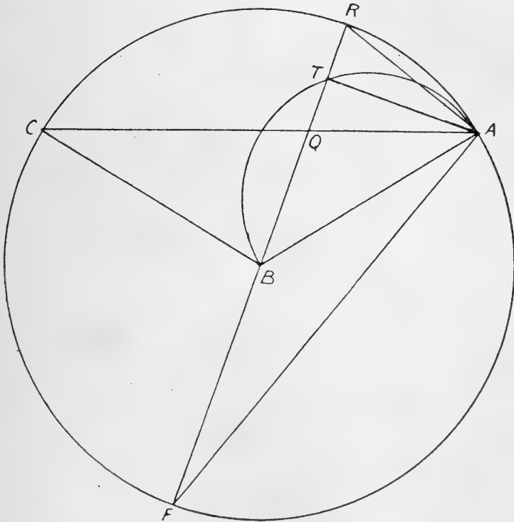
Fig. 16. Löwenturn's Method (No. 1).
