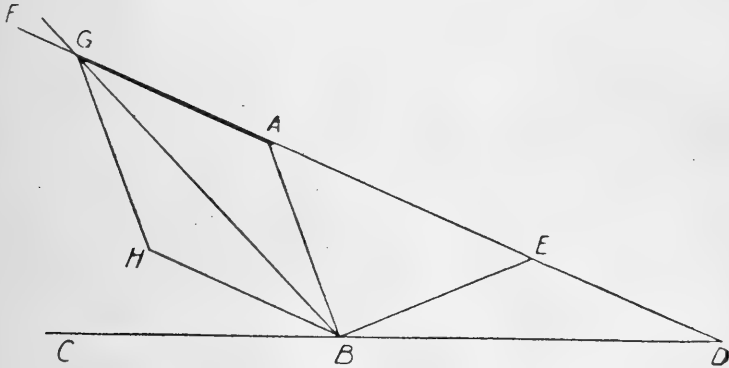
Fig. 21. Adamson's Linkwork (No. 2).
