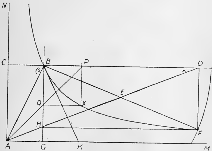
Fig. 6. Method of Pappus (Use of Hyperbola).
