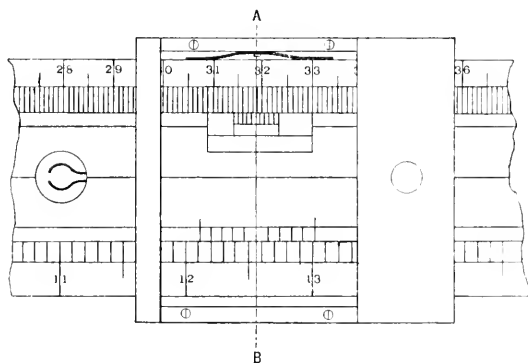
Fig. 1. Plan (lens removed).
