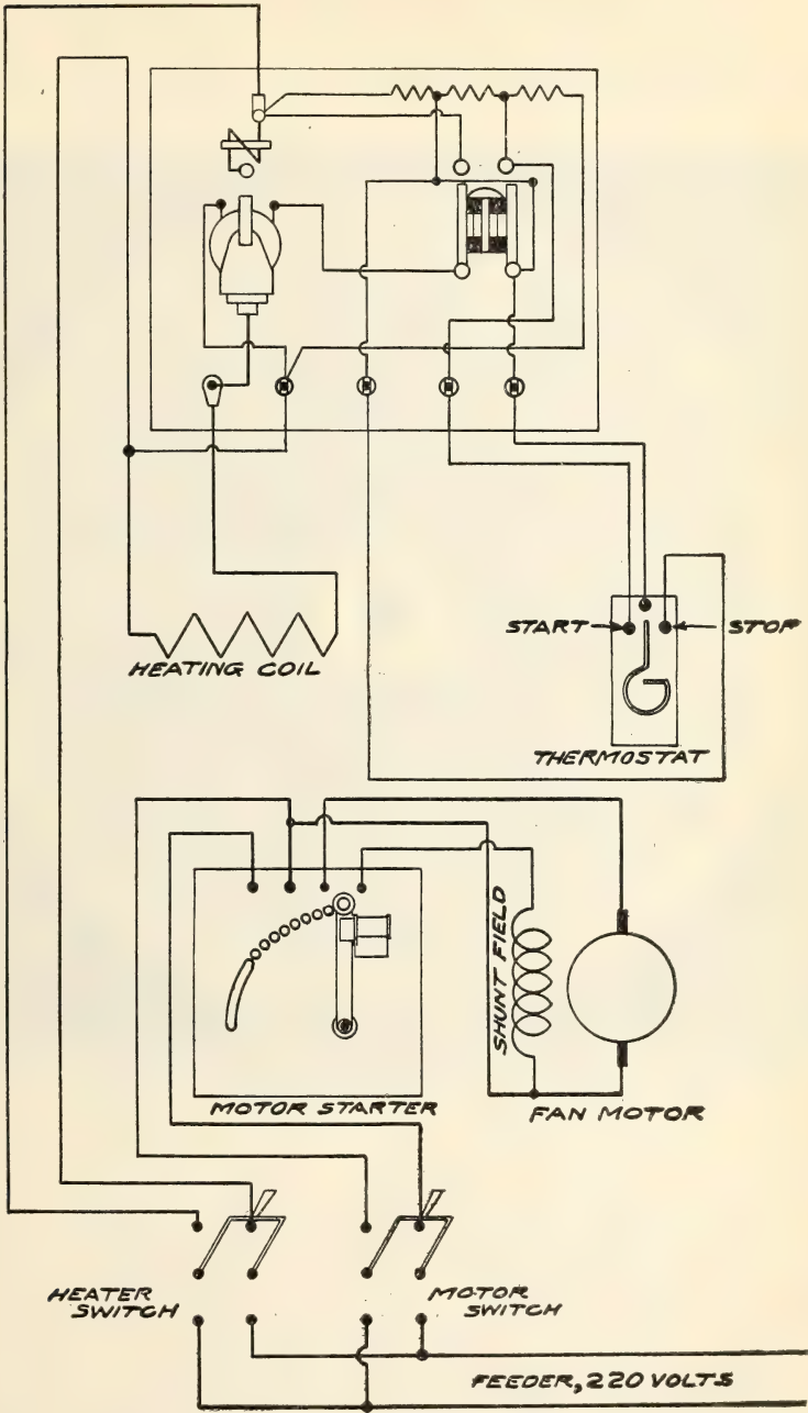
FIG. 10.—Wiring diagram of temperature-control system in Biochemic Division.
