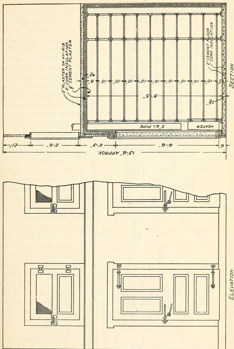
Fig. 3.—Vertical transverse section through incubating compartment and a partial exterior elevation.
