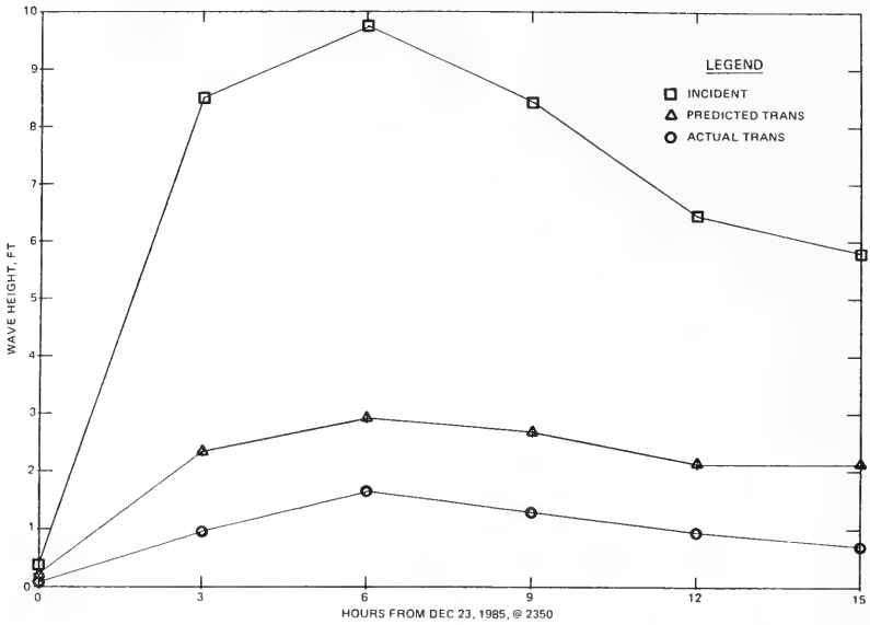
Figure 7. Incident and transmitted wave heights Burns Harbor, Indiana
