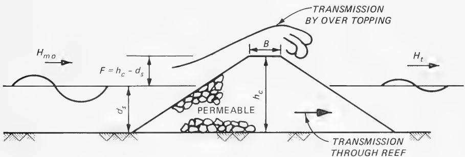
Figure 1. Definition sketch for wave transmission over and through a reef breakwater
