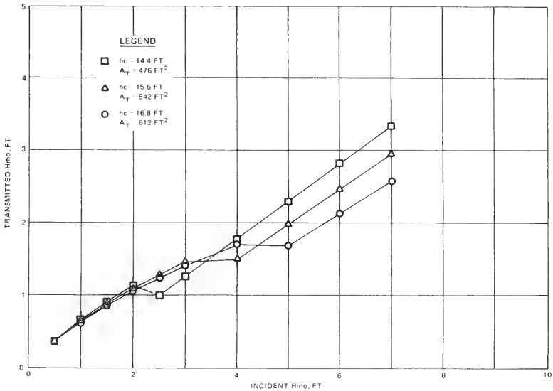
Figure 5. Transmitted wave height versus incident wave height for reef breakwaters, in water depth of 12.0 ft, exposed to incident wave spectrum with period of peak energy density of 8.0 sec
