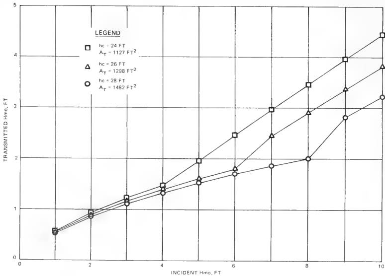
Figure 4. Transmitted wave heights versus incident wave height for reef breakwaters, in water depth of 20 ft, exposed to incident wave spectrum with period of peak energy density of 8.0 sec
