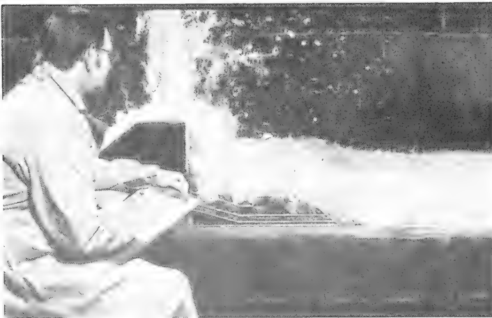
Figure 16. Laboratory tests of wave action against a Cape Hatteras seawall, vertical configuration
