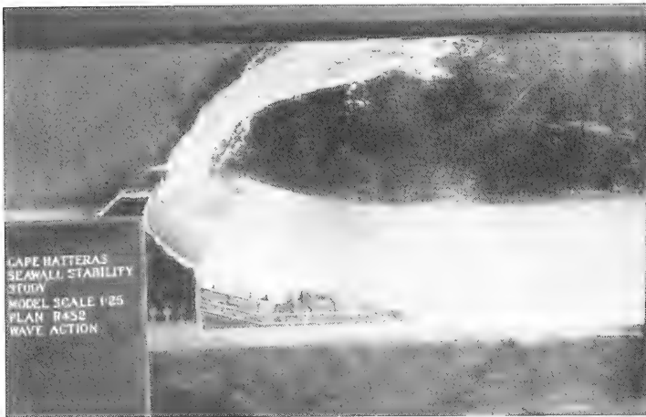
Figure 15. Laboratory tests of wave action against a Cape Hatteras seawall with a moderate recurve
