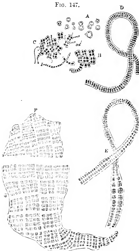
Successive stages of development of Ulea .
