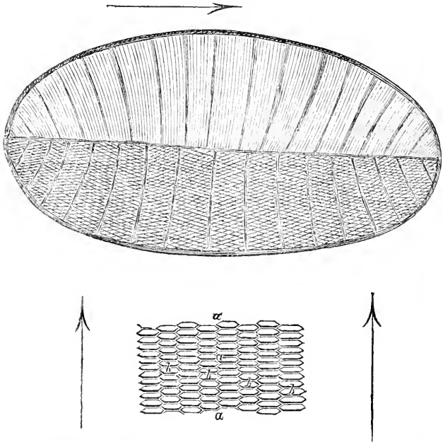
Valve of Sarrella gemma , with portion more highly magnified, showing two systems of markings a and b .
