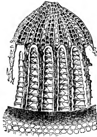
Double Peristome of Cinclidium arcticum .
