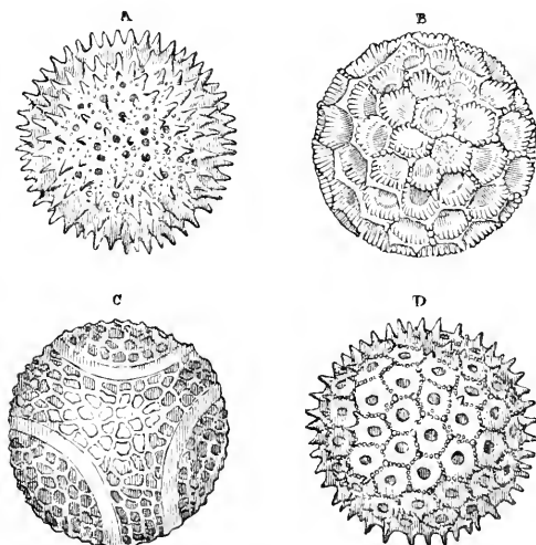
Pollen-grains of,—A, Althaea rosea ; B, Cobaea scandens ; C, Passiflora carulea ; D, Ipomoea purpurea .
