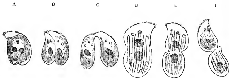
Fissiparous multiplication of Chilodon cucullulus :—A, B, C, successive stages of longitudinal fission (?); D, E, F, successive stages of transverse fission.
