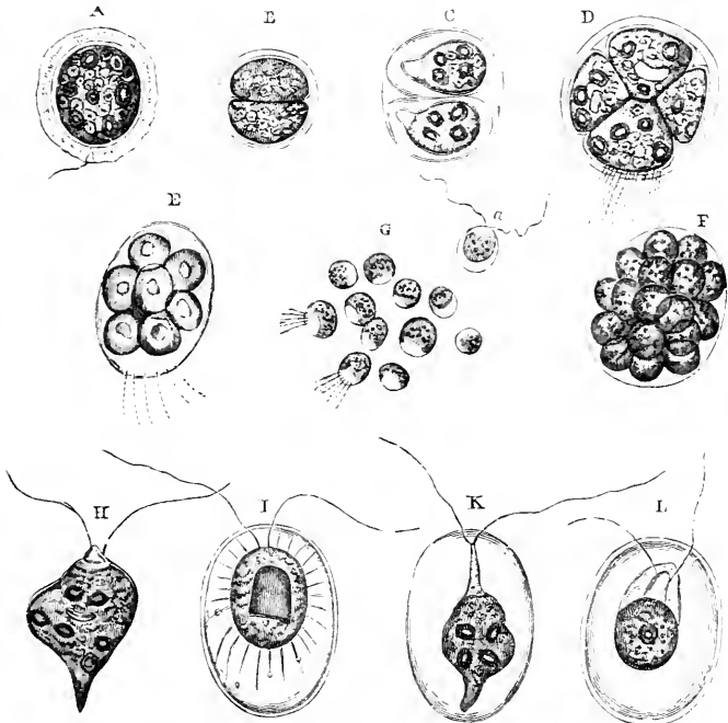
DEVELOPMENT OF PALMOGLEA AND PROTOCOCCUS.
