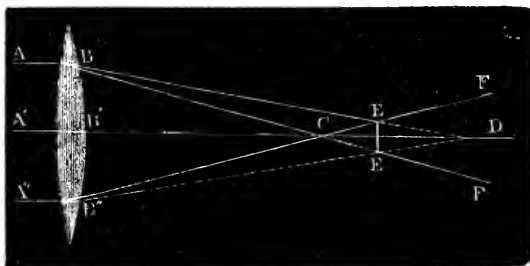
Diagram illustrating Chromatic Aberration .
