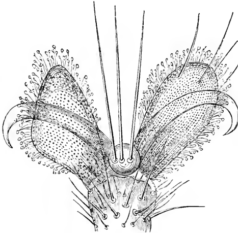
Foot of Fly .
