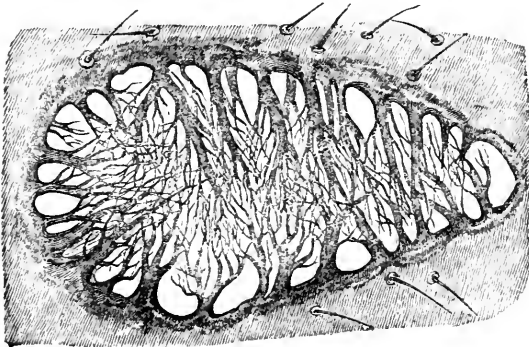
Spiracle of Common Fly .
