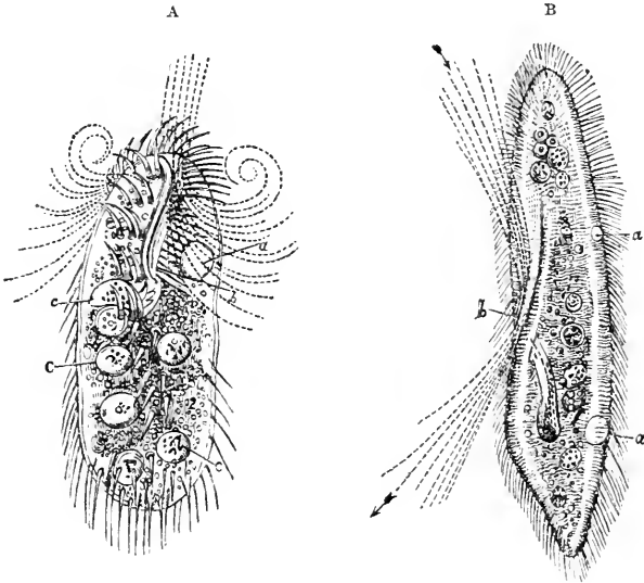
A, Kerona silurus :— a , contractile vesicle ; b , mouth ; c , c , Animalcules swallowed by the Kerona , after having themselves ingested particles of indigo. B, Paramecium caudatum :— a , a , contractile vesicles ; b , mouth.
