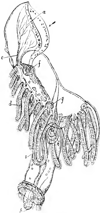
Actinotrocha branchiata :— a , Episotome or hood; b , Anus; c , Stomach; d , Ciliated Tentacula; e , Mouth.
