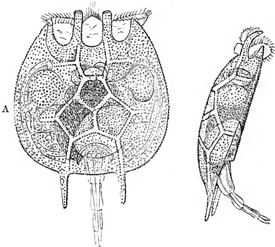
Notozoum quadricornis ; A, dorsal view ; B, side view.
