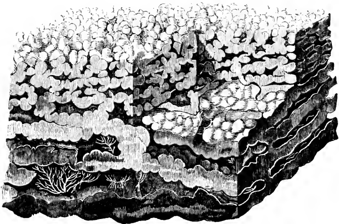
STRUCTURE OF EOZOON CANADENSIS.
