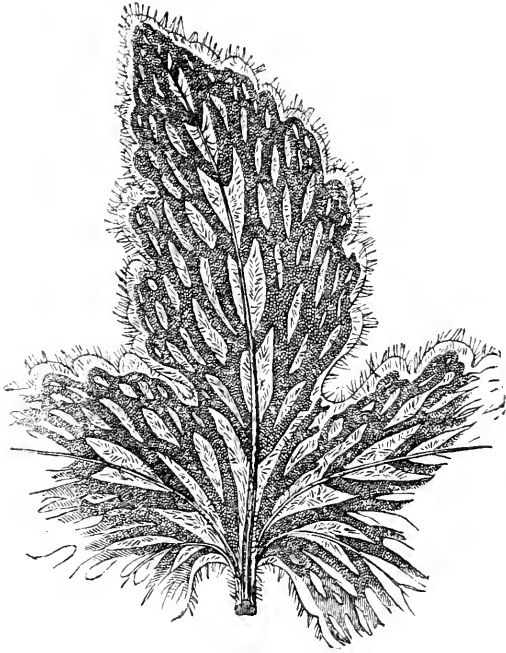
Portion of Frond of Hemionitis , with Sori.
