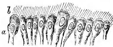
Ciliated Epithelium ; a, nucleated cells, resting on their smaller extremities; b, cilia.
