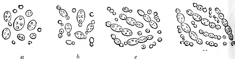
Torula cerevisia , or Yeast-Plant, as developed during the process of fermentation:— a , b , c , d , successive stages of Cell-multiplication.
