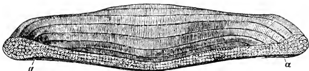
Alveolina Quoiï .— a, a , septal plane, showing multiple pores.
