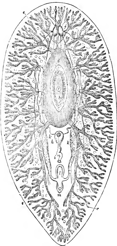
Structure of Polycelis levigatus (a Planarian worm):—a, Mouth, surrounded by its circular sucker; b, Buccal cavity; c, Oesophageal orifice; d, Stomach; e, ramifications of Gastric Canals; f, Cephalic Ganglia and their Nervous filaments; g, g, Testes; h, Vesicula seminalis; i, male genital canal; k, k, Oviducts; l, dilatation at their point of junction; m, Female genital orifice.
