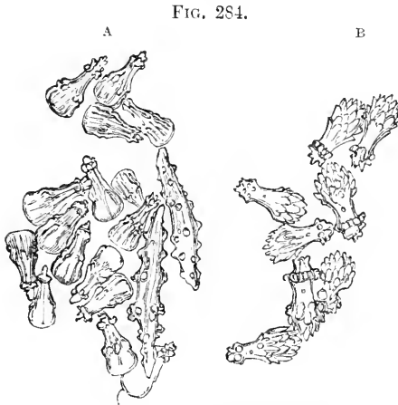
A, Spicules of Gorgonia guttata . B, Spicules of Muricea elongata .
