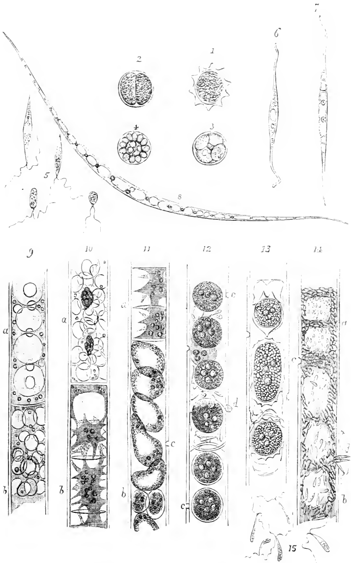
DEVELOPMENT AND REPRODUCTION OF SPHEROPLEA.
