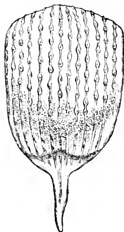
Battledoor Scale of Polyommatus argus (Azure-blue).
