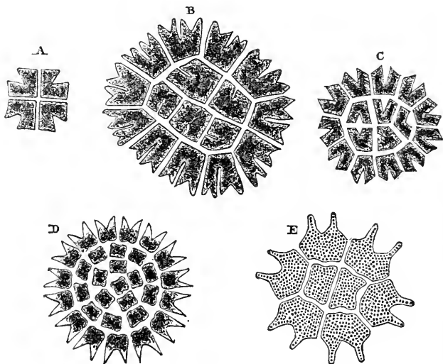
Various species(?) of Pediastrum :—A, P. tetras ; B, C, P. bivadiatum ; D, P. pertusum ; E, empty frond of P. granulatum .
