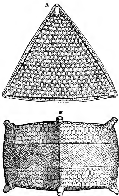
Triceratium farus .—A, side view ; B, front view.
