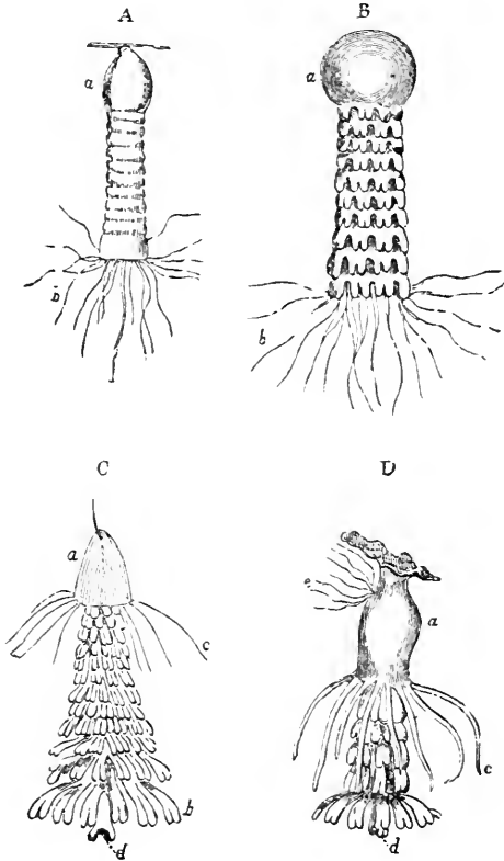
Successive Stages of Development of Medusa-buds from Strobila-larva :— a , Polype-body ; b , its original circle of Tentacles ; c , its secondary circle of Tentacles ; d , proboscis of most advanced Medusa-disk ; e , Polype-bud from side of Polype body.
