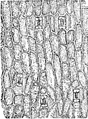
Cuticle of Leaf of Yucca .
