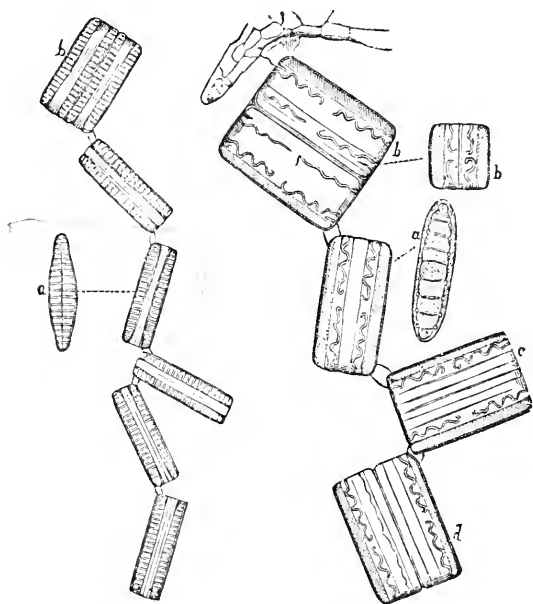
Fig. 127.— Diatoma vulgare :— a , side view of frustule; b , frustule undergoing self-division.
