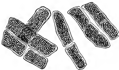
Cells of Paony , filled with Starch.
