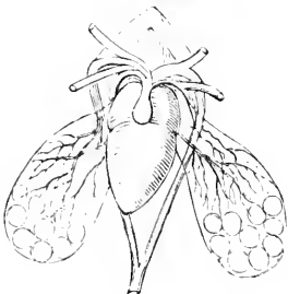
CIRCULATION IN TADPOLE.
