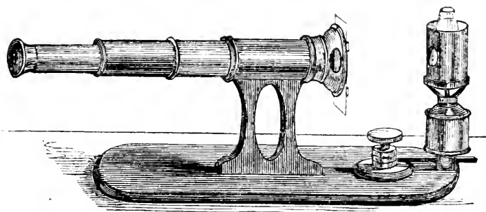
Prof. Beale's Demonstrating Microscope.
