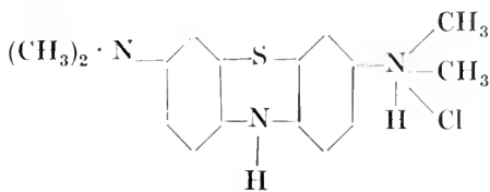
Leuco-methylene blue (colourless)
