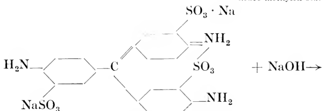
Disodium pararosanilin trisulphonate (red)—one of the primary constituents of acid fuchsin
