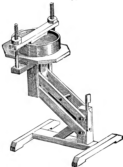
Fig. 82. Cheese-press.
