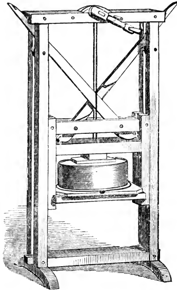
Fig. 83. Self-acting cheese-press.
