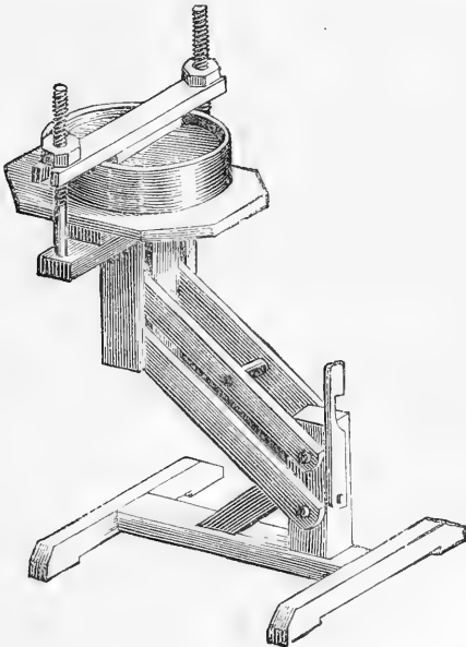
Fig. 82. Cheese-press.
