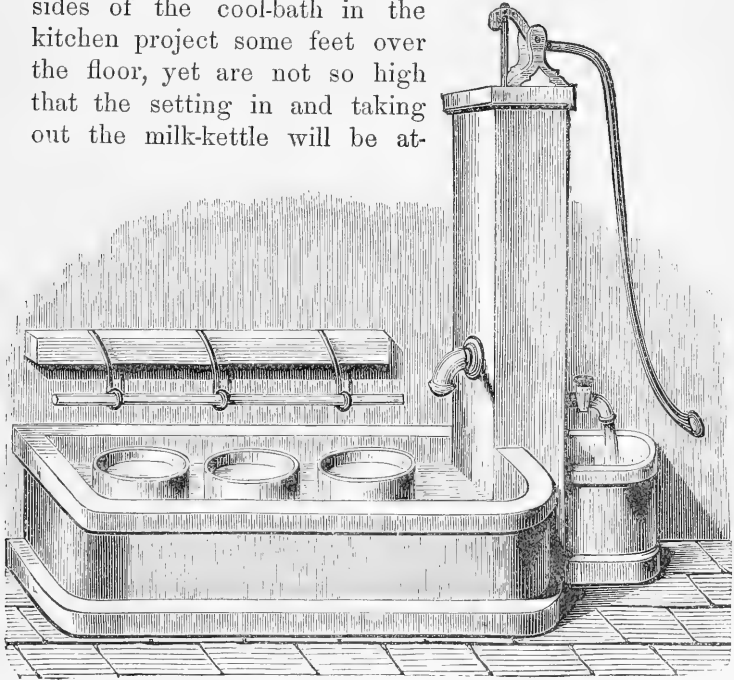
Fig. 96. Cool-bath.
