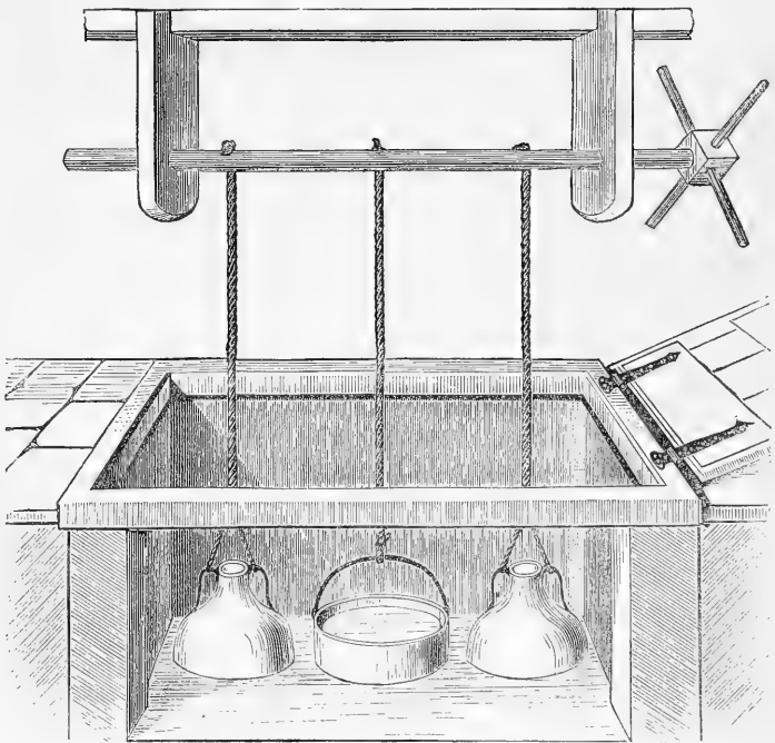
Fig. 97. Cool-bath
