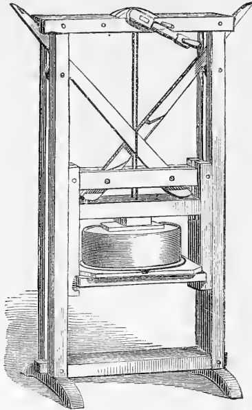
Fig. 83. Self-acting cheese-press.
