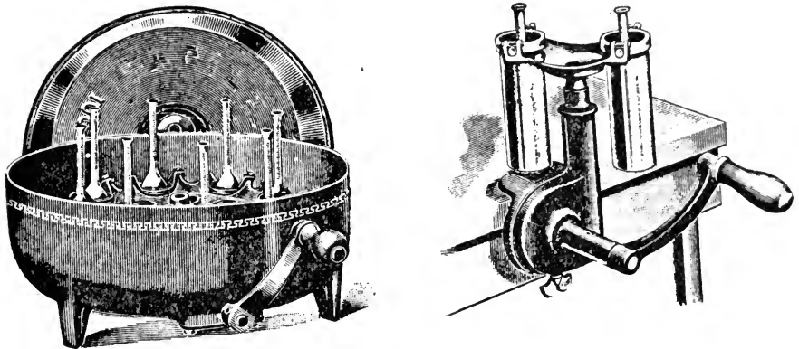
Fig. 4. Types of Babcock testers, in which the test-bottles are whirled.
