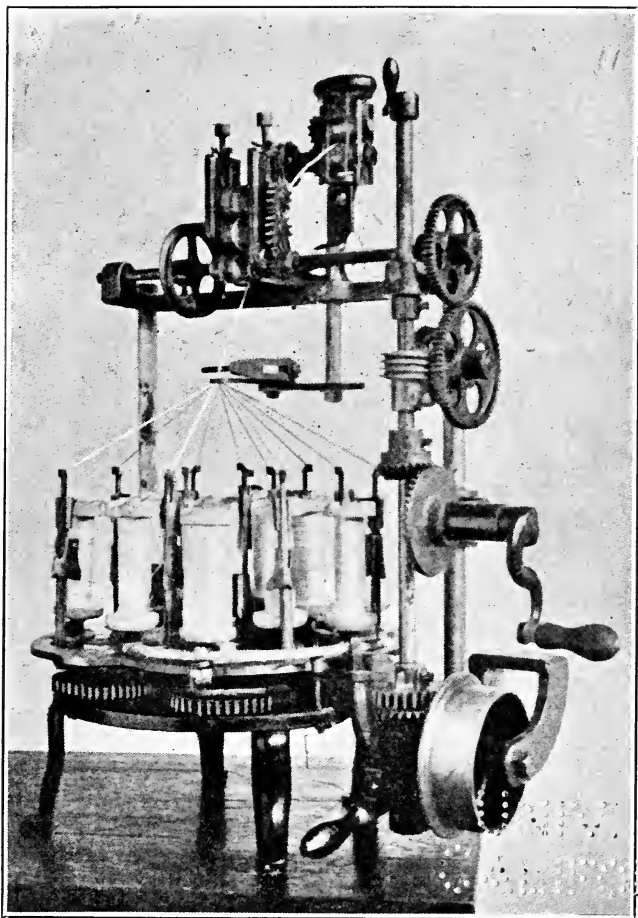
Courtesy of "The Philippine Craftsman" Figure 3. Thirteen-Spool Braiding Machine
