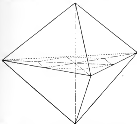
FIG. 204.—The Positive Trigonal Pyramid of the Second Order, (\overline{hh\bar{2}hl}) .
