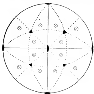
FIG. 107.—The Plus Right Tetartohedral Pentagonal Dodecahedron. Tetartohedron.
