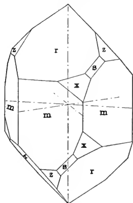
FIG. 210.—Right-handed Quartz: Combination of m(10\bar{1}0) , r(10\bar{1}1) , z(01\bar{1}1) , s(11\bar{2}1) , x(51\bar{6}1) .
