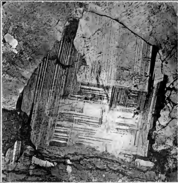
FIG. 459. — Section of a Complexly Twinned Feldspar between Crossed Nicols.
