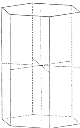
FIG. 157. — Hexagonal Prism of the First Order, a : \infty a : a : \infty c , (h0h0) .
