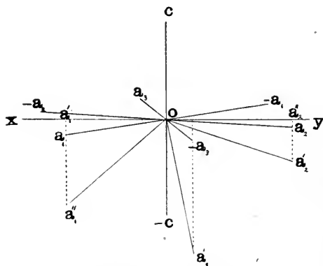
FIG. 53.—Axial Cross of Apatite; \dot{c} = 0.734+ .
