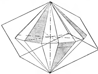
FIG. 184.—The Plus Left Rhombohedron of the Third Order, (\overline{ikh\bar{l}}) .
