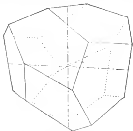
FIG. 109.—The Plus Right Tetartohedral Pentagonal Dodecahedron, \kappa\pi(hkl) .
