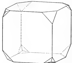
FIG. 98. — Combination of (100), \kappa(111) , \kappa(211) on Boracite.
