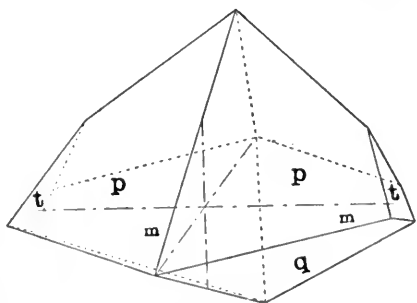
FIG. 257. — Combination of p(111) , q(111) , m(\bar{1}10) , t(771) , z(161) on Clinohedrite.
