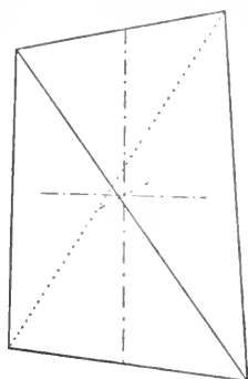
FIG. 142 a.—The Plus Right Tetragonal Sphenoid of the Third Order.
