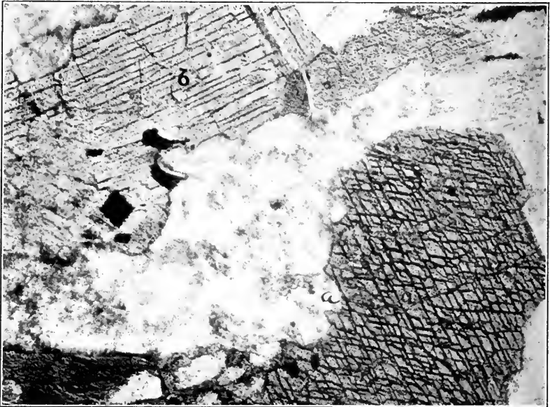
FIG. 478.—Section of Diorite, showing the Relief and Cleavage Angle, 124^{\circ} , of Hornblende a , and also the Parallel Cleavage b , when cut Parallel to the Vertical Axis.
