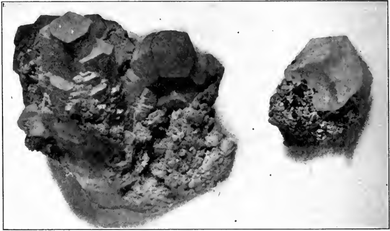
FIG. 438. — Prismatic Habit of Calcite, Wanlockhead, Scotland. The Small Specimen is the Rhombohedron e , Freiberg, Saxony.
