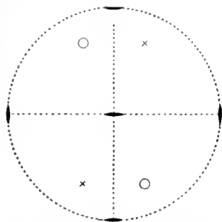
FIG. 232. — Type 6, Digonal Holoaxial.
