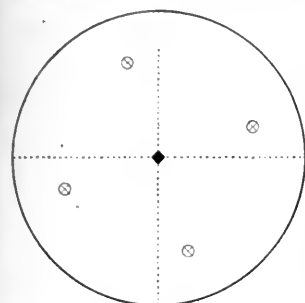
FIG. 131.—Type 24: Tetragonal Equatorial.
