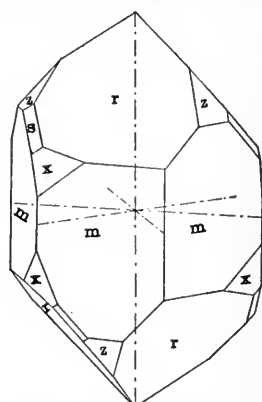
FIG. 211.—Left-handed Quartz, m(10\bar{1}0) , r(10\bar{1}1) , z(01\bar{1}1) , s(2\bar{1}\bar{1}1) , x(6\bar{5}\bar{1}1) .
