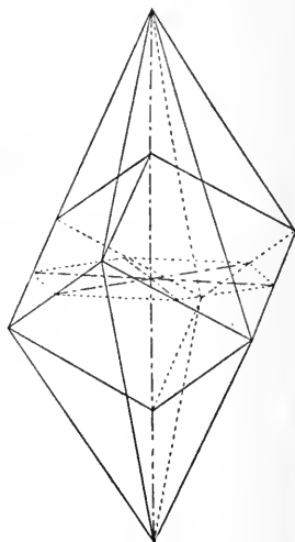
FIG. 164 a.—The Rhombohedron of the Middle Edge and Scalenohedron.
