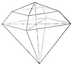
FIG. 130.—Silver Fluoride, AgF, H 2 O; Combination of (111), (11 \bar{1} ) (113).
