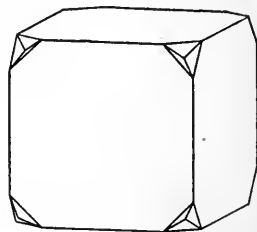
FIG. 29. — The Cube with the Corners replaced by the Tetragonal Trisectahedron.
