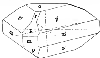
FIG. 196. — Benitoite, Combination of p(10\bar{1}1) , p'(0\bar{1}11) , m(10\bar{1}0) , r(10\bar{1}2) , c(0001) .
