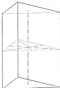
FIG. 206.—The Plus Trigonal Prism of the Second Order, (\overline{hh\bar{2}ho}) .
