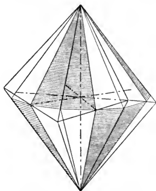
FIG. 162. — The Positive Scalenohedron, k(hh\bar{1}l) .
