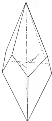
FIG. 139 a . — The Left Tetragonal Trapezohedron, \tau(212) .
