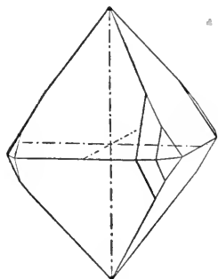
FIG. 136. — Combination of (101) (111) and (313) of Scheelite.
