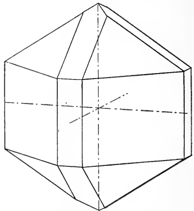
FIG. 119.—Combination of (111) (101) (110) (100) of Cassiterite.
