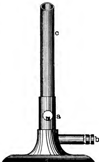
FIG. 525. — The Bunsen Burner.
