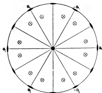
FIG. 152. — Type 20, Dihexagonal Equatorial.
