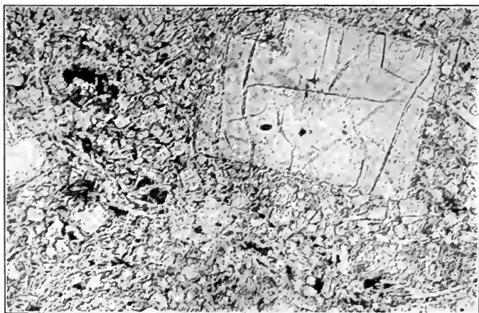
FIG. 482. — Nepheline in a Section of Phonolite. The Small Square Crystals are also Nepheline. The Elongated Crystals are Feldspar.
