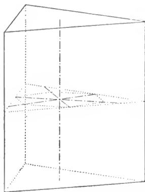
FIG. 205.—The Negative Left Trigonal Prism of the Third Order, (i\overline{kh}l) .
