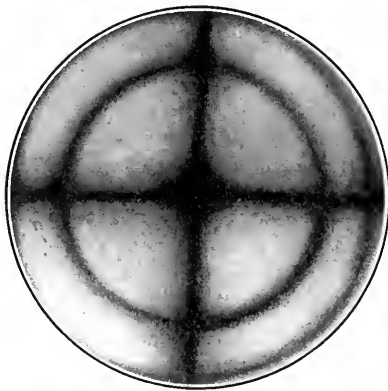
FIG. 342. — Interference Figure of Brucite.
