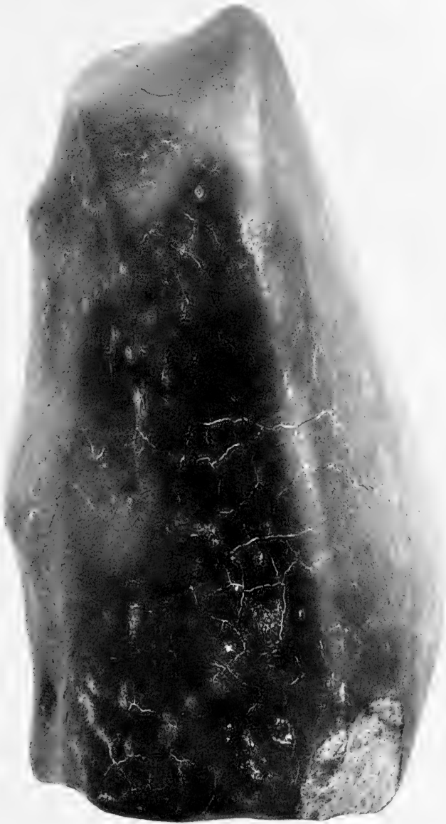
Meteoric Stone. One of the larger individuals of the fall at Modoc, Kansas, on September 2, 1905. Weight 2,268 grams
