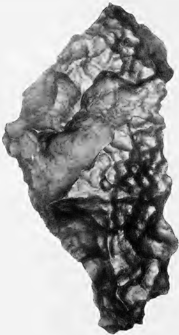
Iron Meteorite: Owens Valley, Inyo Co., California. Found by shepherd in 1913, and presented to the National Museum by Mr. Lincoln Ellsworth. Length 65 centimeters; weight 193.17 kilograms (425 lbs.). The iron shows to excellent advantage the so-called "piezoglyphs," or "thumb markings"
