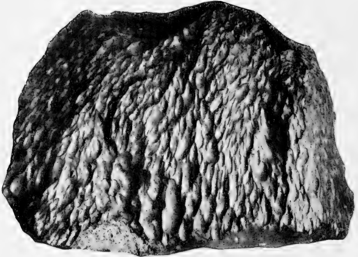
Meteoric Stone, Bath Furnace, Kentucky.
