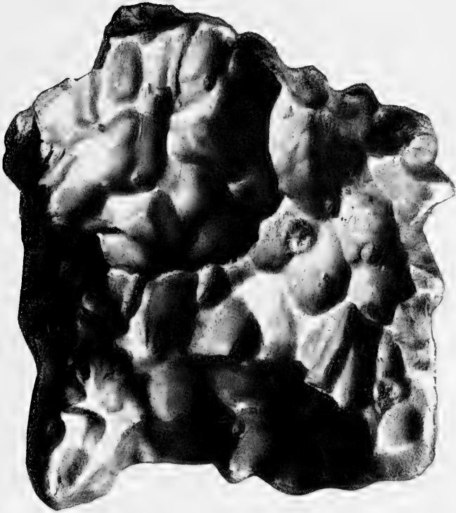
Meteoric Iron. Fell at Mazapil, Mexico, Nov. 27, 1885. Weight about 4 kilograms or 8.8 lbs. Note the beautiful sculpturing or piezoglyphs. For description of fall see p. 21
