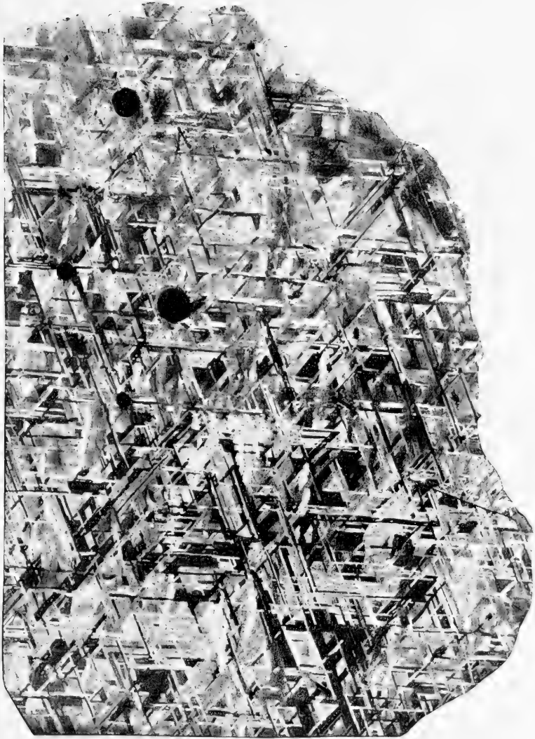
Etched surface of a slice from the Casas Grandes Meteoric Iron
