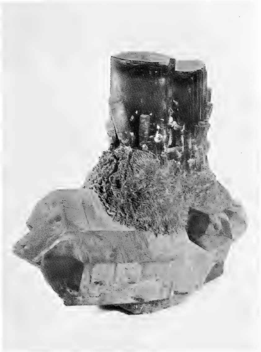
Group of tourmaline crystals, Mesa Grande, California. Roebling Collection, National Museum
