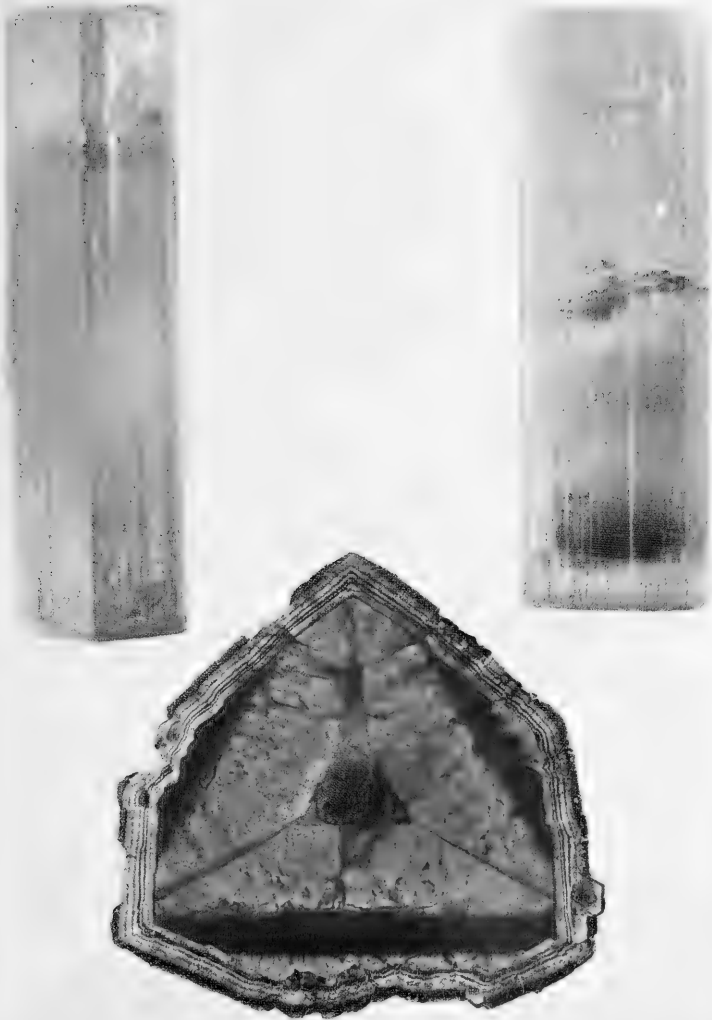
Tourmaline. Crystals from Mesa Grande, California; Cross-section from Tsilaizina, Madagascar
