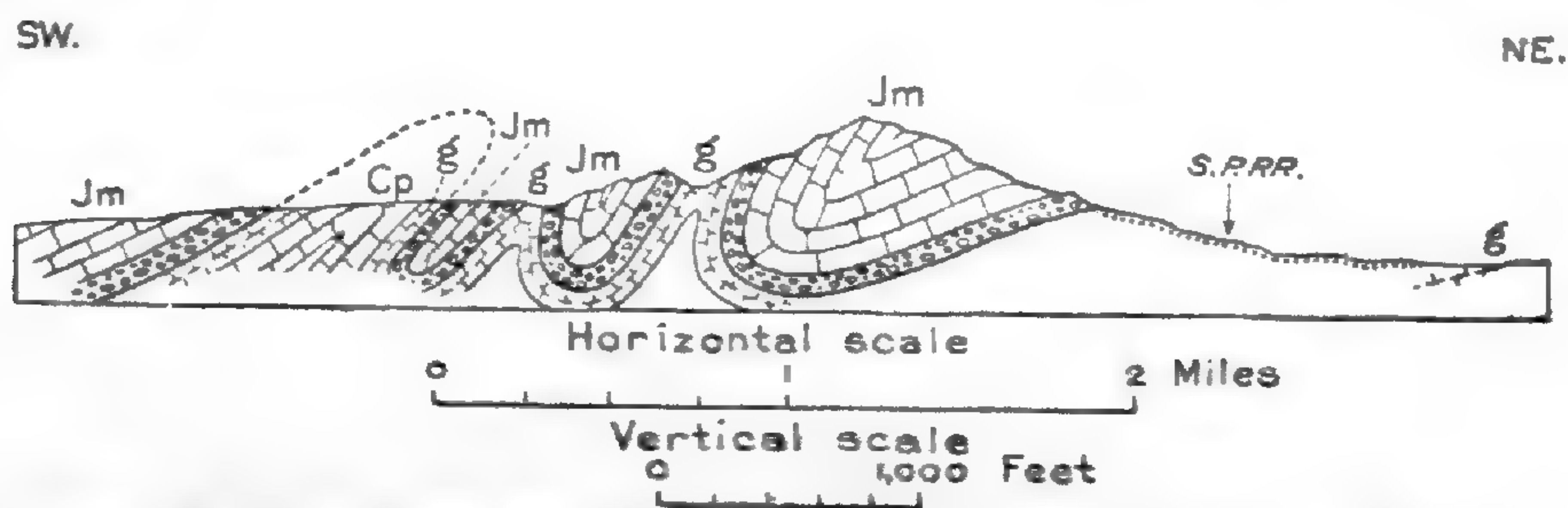
FIGURE 24.—Section across the Malone Mountains, Tex. After C. L. Baker (personal communication). Jm, Malone limestone (Jurassic). Cp, Limestone, etc.; g, gypsum (both Permian)
