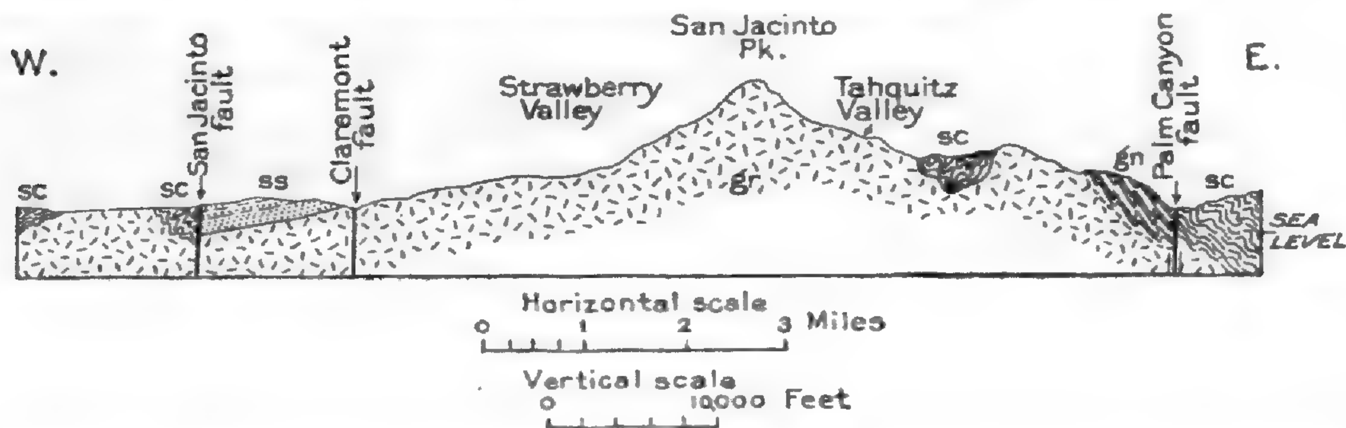
FIGURE 63.—Section through the San Jacinto Mountains, Calif. After Frazer. ss, Sandstone; sc, schist; gn, gneiss; gr, granite
