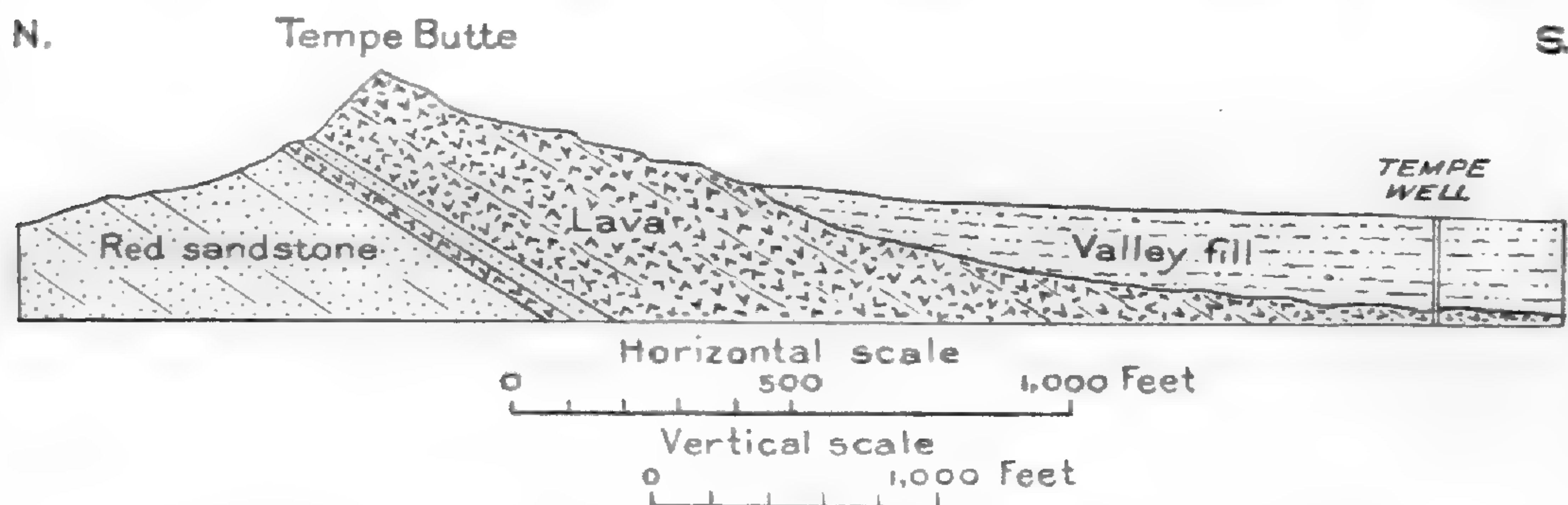
FIGURE 50.—Section through Tempe Butte and Tempe Well, Ariz. After Lee
