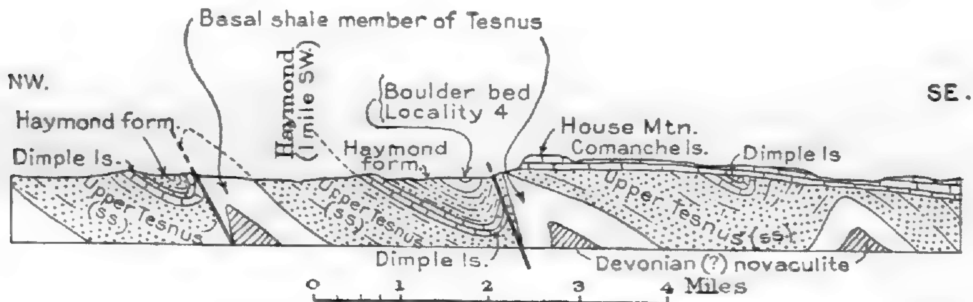
FIGURE 10.—Section through House Mountain, about 1 mile north of the railroad northwest of Tesnus, Tex.
