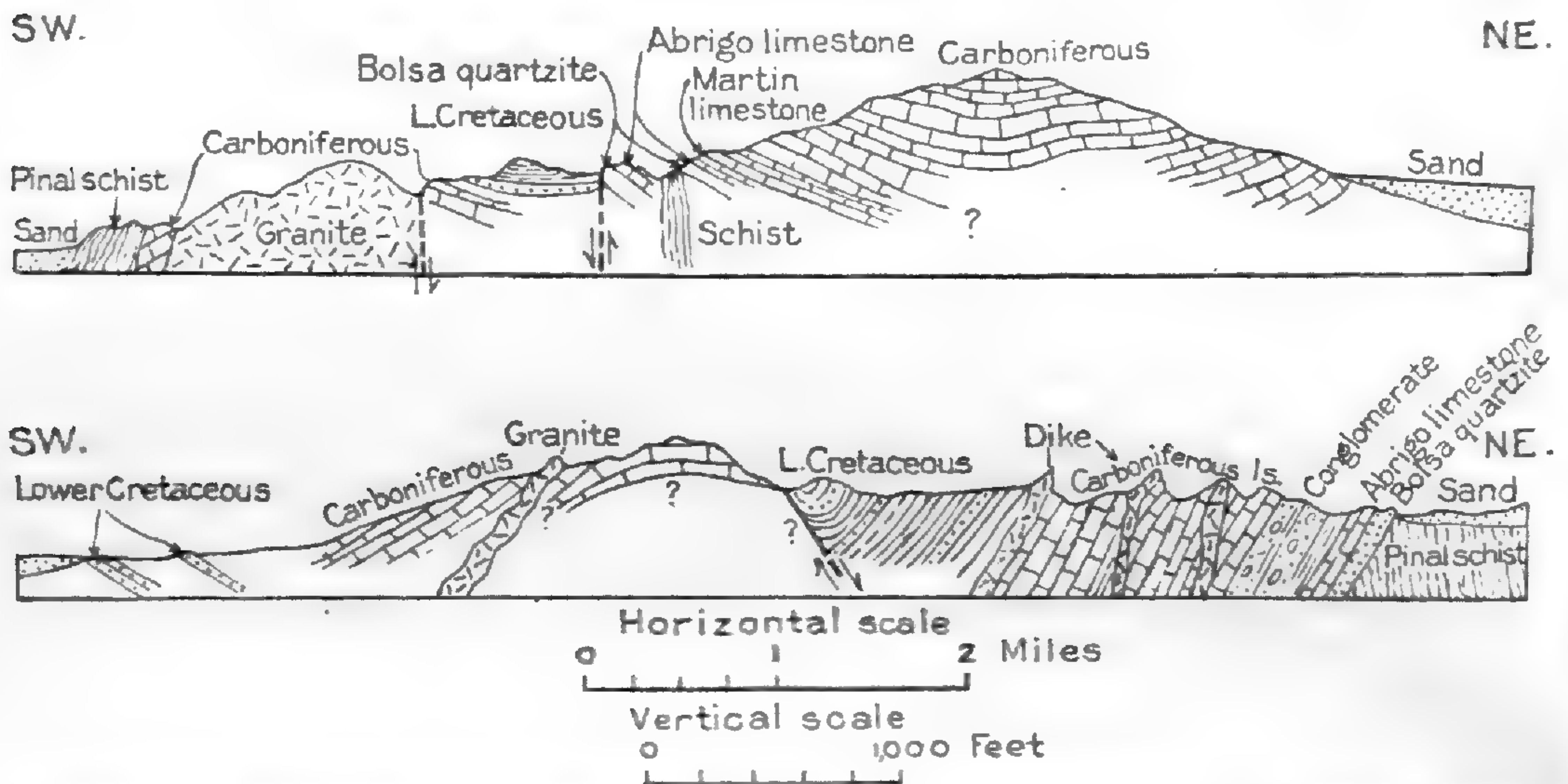
FIGURE 37.—Sections across the Dragoon Mountains, Ariz. Upper section, 3 to 6 miles southwest of the railroad; lower, 12 miles southwest of the railroad
