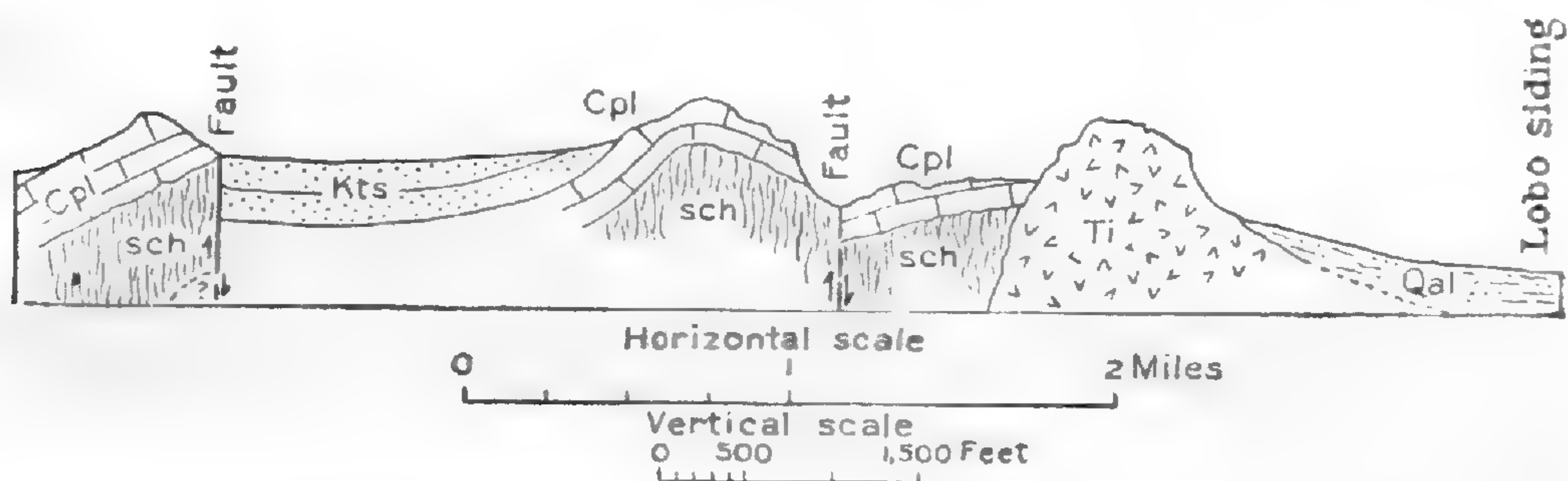
FIGURE 16.—Section across the Van Horn Mountains near their north end. Kts, sandstone (Cox); Cpl, Permian limestone; sch, Carrizo Mountain schist; Qal, alluvium; Ti, igneous rock
