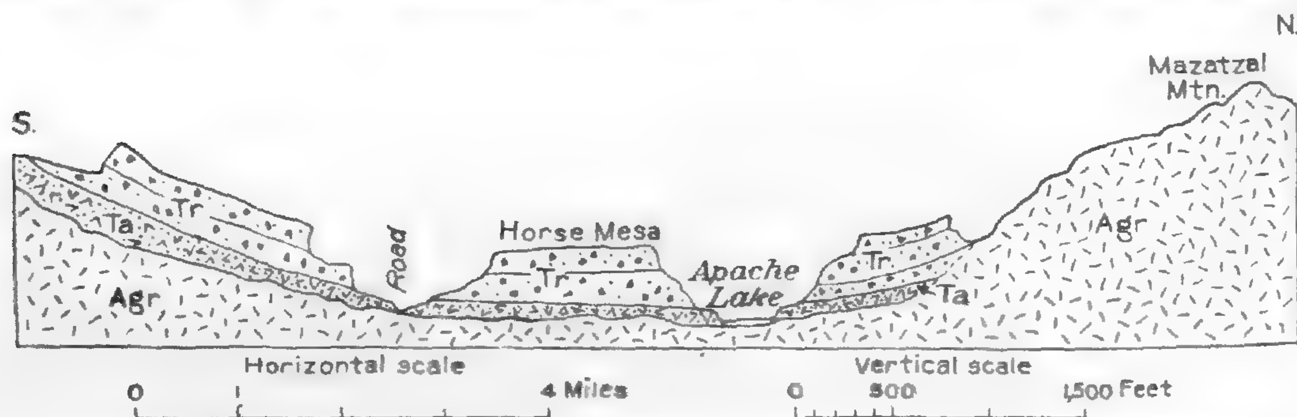
FIGURE 58.—Section showing relations of Tertiary volcanic succession 15 miles southwest of Roosevelt Dam, Ariz. Tr, Rhyolite tuff; Ta, andesite; Agr, granite
