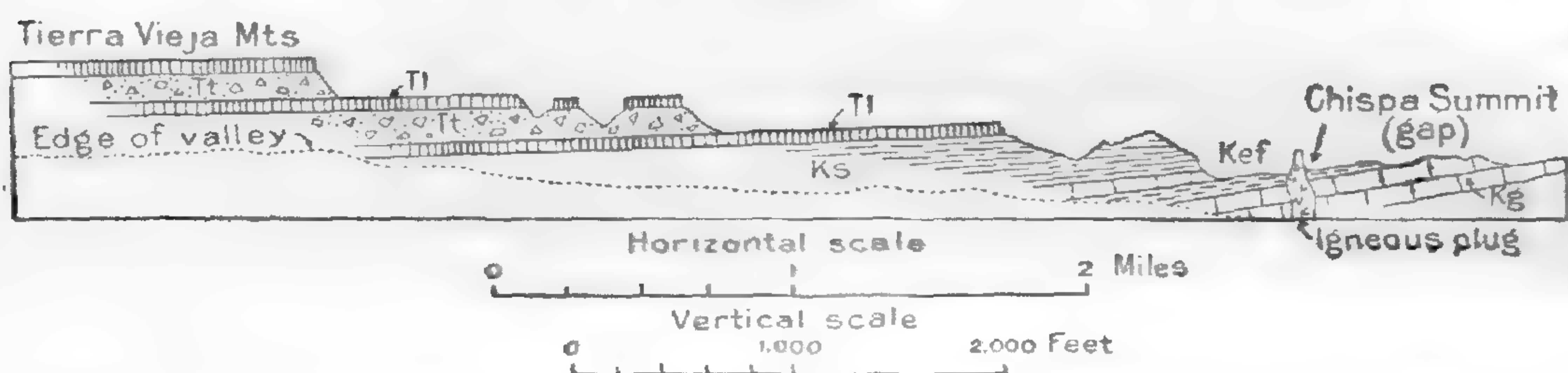
FIGURE 15.—Profile of the northern part of the Tierra Vieja Mountains south of Chispa siding, Tex. Tl, Tertiary lava; Tt, Tertiary tuff; Ks, Upper Cretaceous shale; Kef, Eagle Ford formation (Upper Cretaceous); Kg, Georgetown limestone (Lower Cretaceous)
