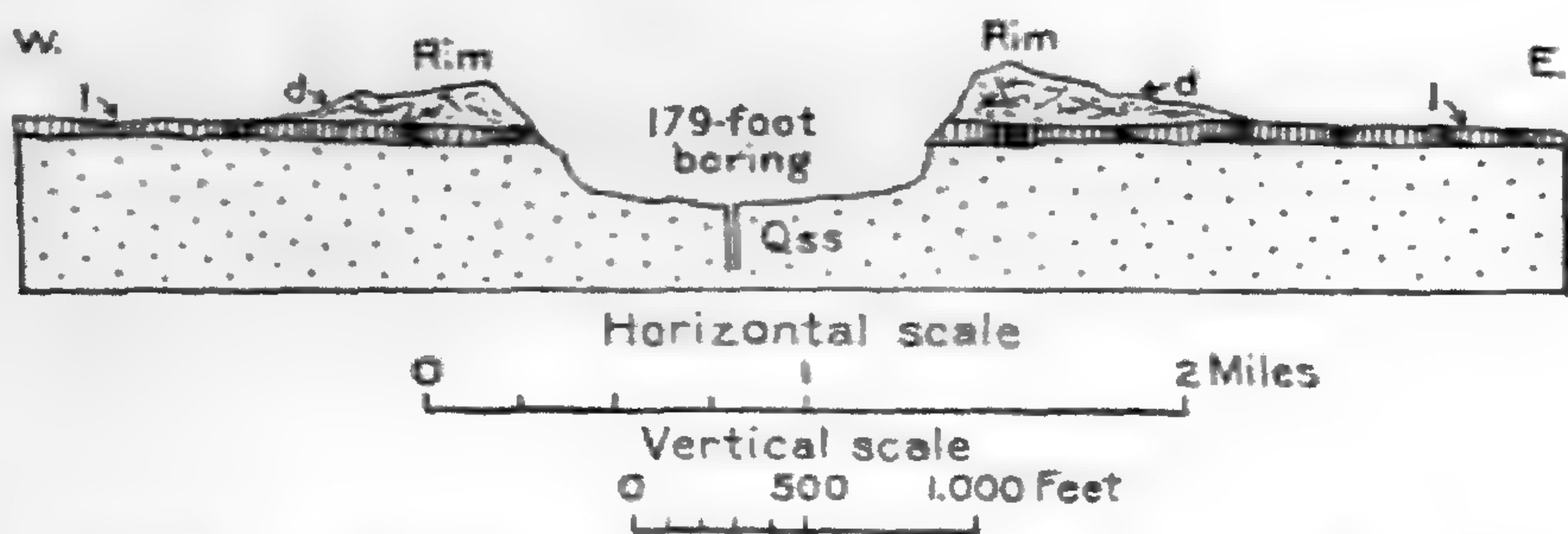
FIGURE 28.—Cross section of Kilbourne Hole, 8 miles west of Lanark, N. Mex. By W. T. Lee. l, Lava; d, ejected material; Qss, sand
