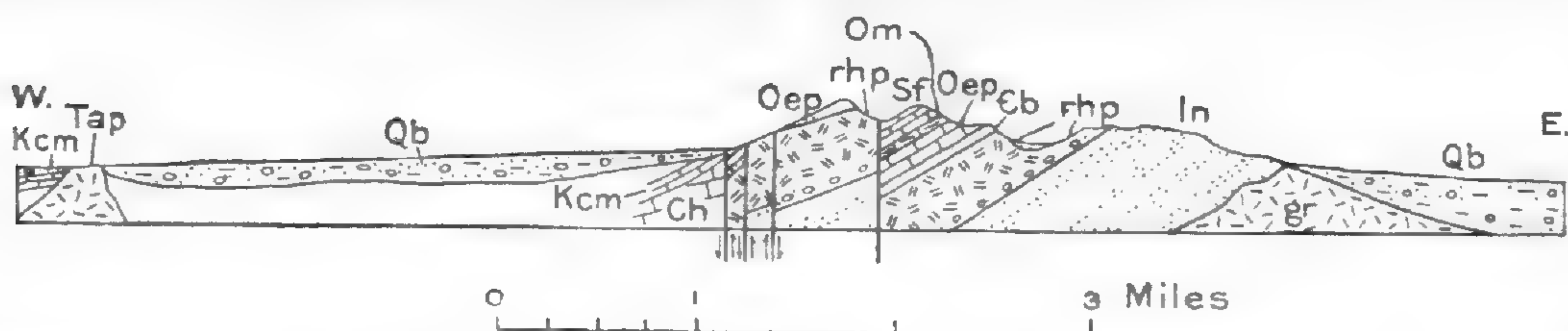
FIGURE 26.—Section across the Franklin Mountains north of El Paso, Tex. After Richardson. In, Lanoria quartzite; rhp, rhyolite porphyry; Eb, Bliss sandstone; Oep, El Paso limestone; Om, Montoya limestone; Sf, Fusselman limestone; Ch, limestone, mostly Permian, underlain by Devonian and Pennsylvanian to the north; Kcm, Comanche series; gr, granite; Tap, andesite porphyry; Qb, bolson deposits
