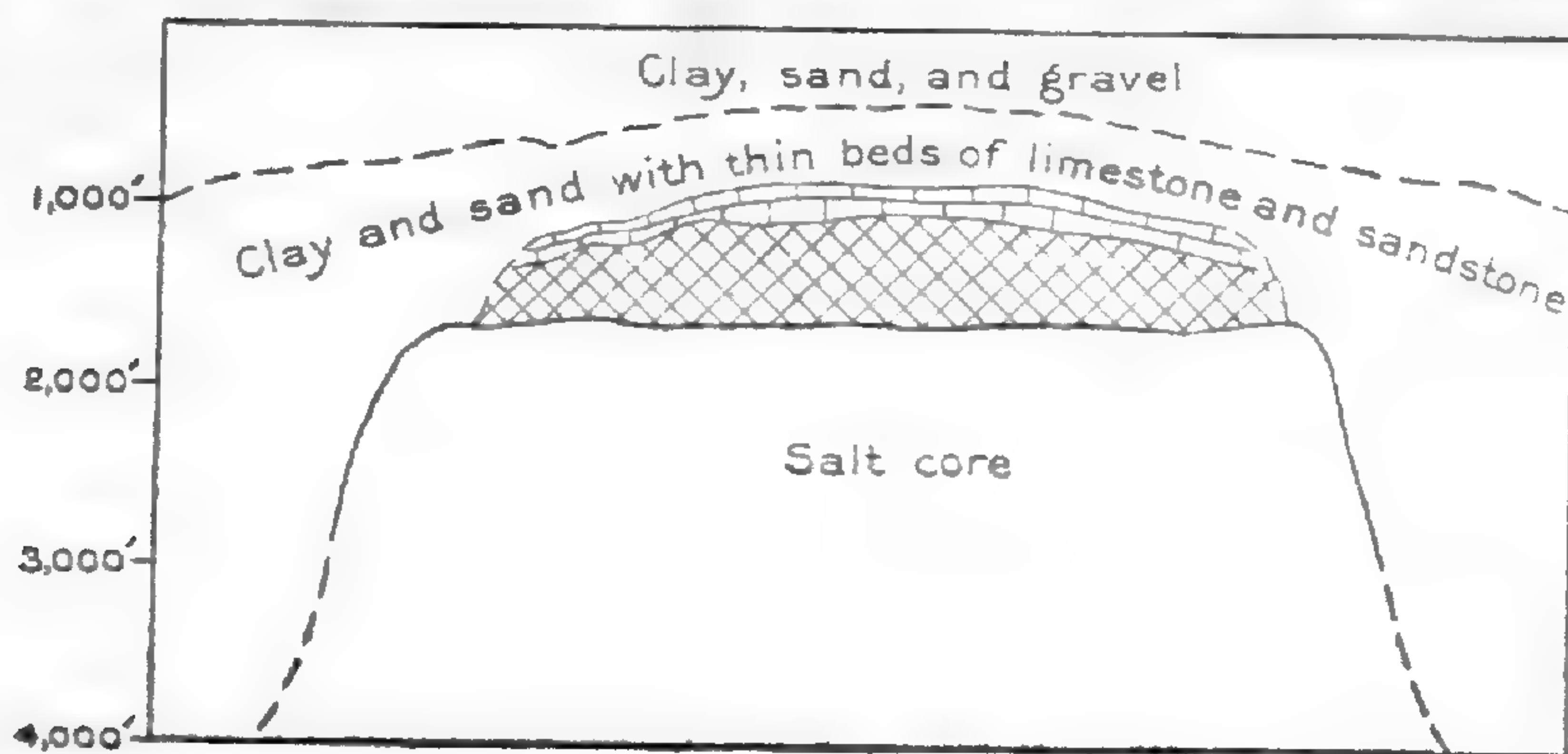
FIGURE 3.—Section through Spindletop salt dome, Texas. Partly after Fenneman
