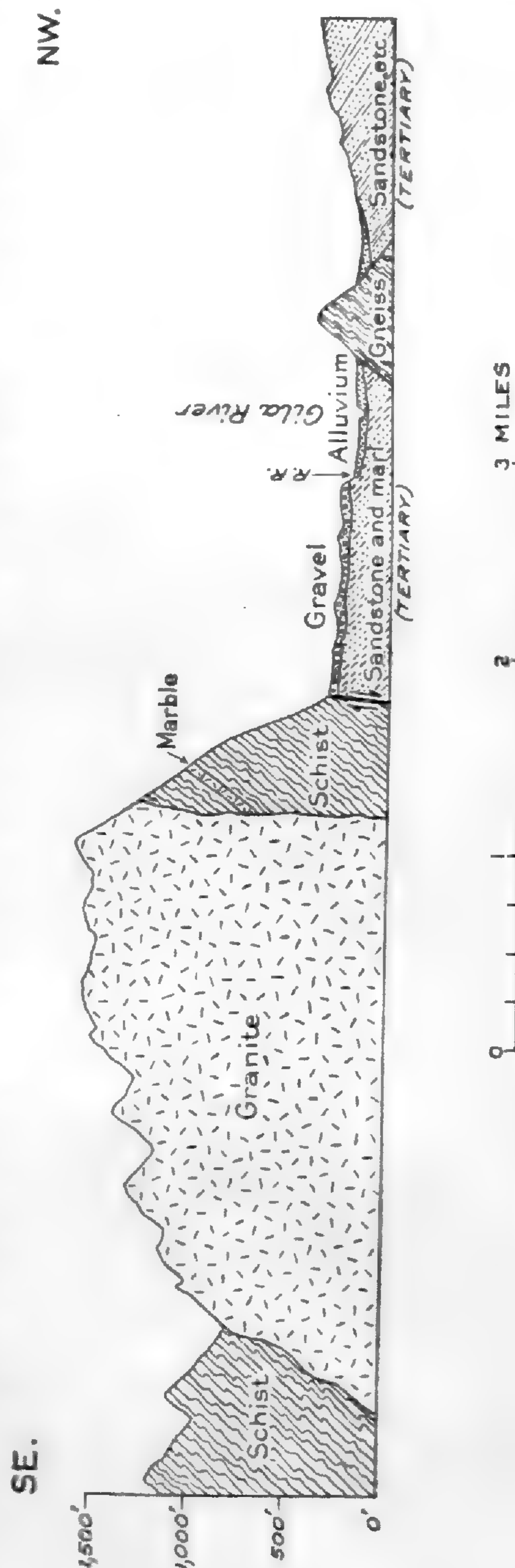
FIGURE 61.—Section of north end of Gila Mountains, Ariz. By E. D. Wilson
