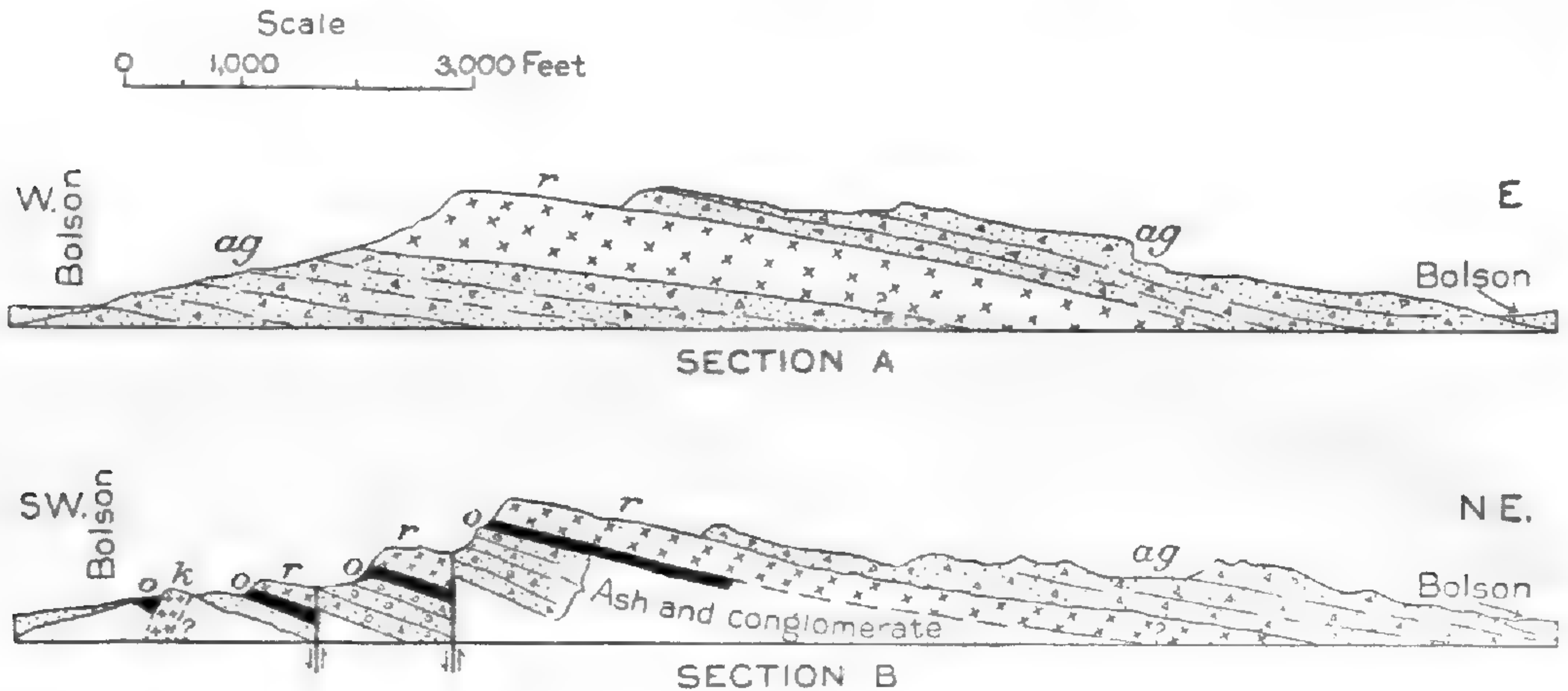
FIGURE 31.—Sections across the Little Florida Mountains, N. Mex. A, Across center of range; B, 1\frac{1}{2} miles farther south. ag , Agglomerate; r , felsitic rhyolite; o , obsidian; k , keratophyre
