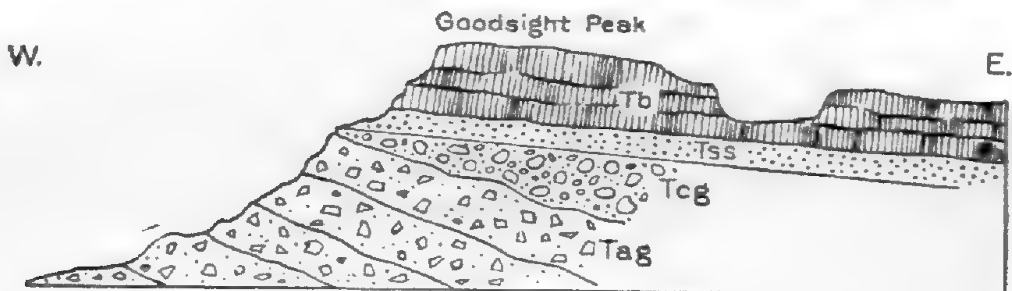
FIGURE 29.—Section through Goodsight Peak, 15 miles northwest of Cambray, N. Mex. Tb, lava (basalt); Tss, gray sandstone; Tcg, conglomerate; Tag, agglomerate
