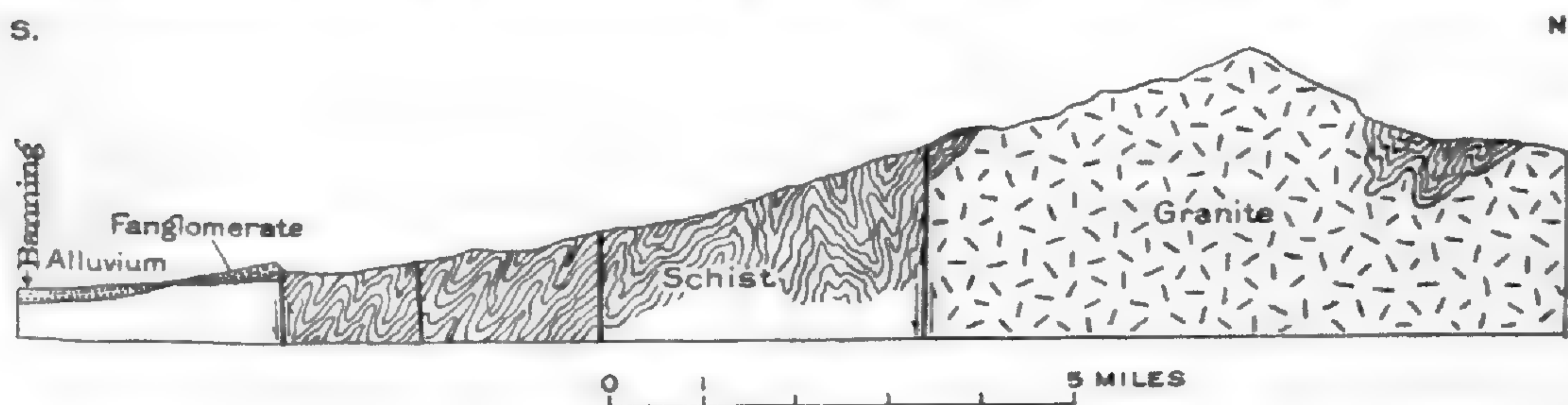
FIGURE 65.—Section from Banning, Calif., north to San Bernardino Mountain. After Vaughan
