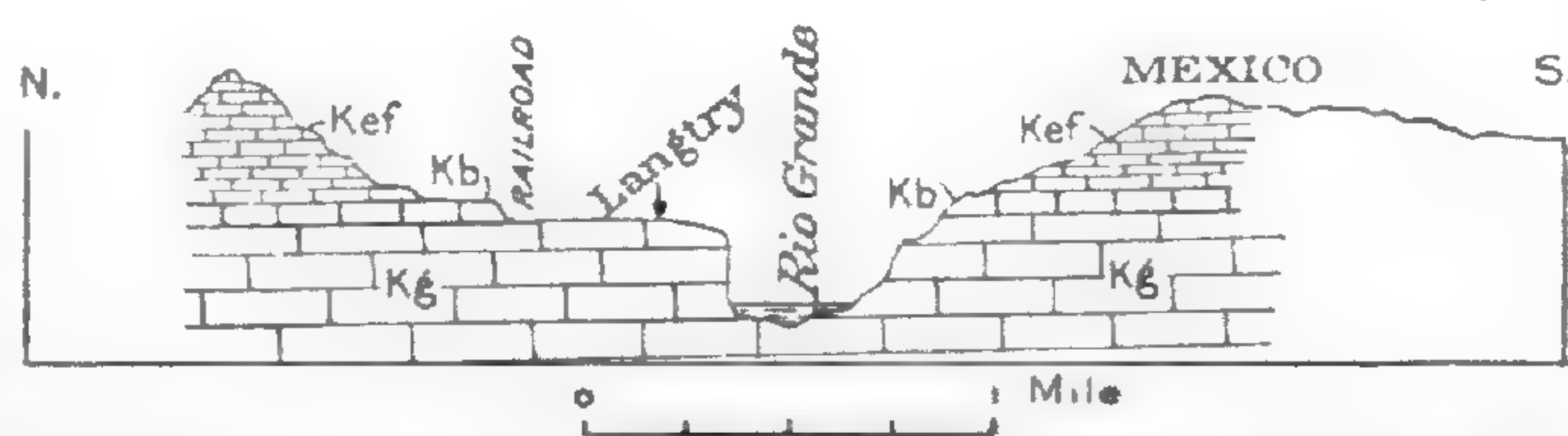
FIGURE 8.—Section at Langtry, Tex. Kef, Eagle Ford limestone; Kb, Buda limestone; Kg, Georgetown limestone (all Cretaceous)
