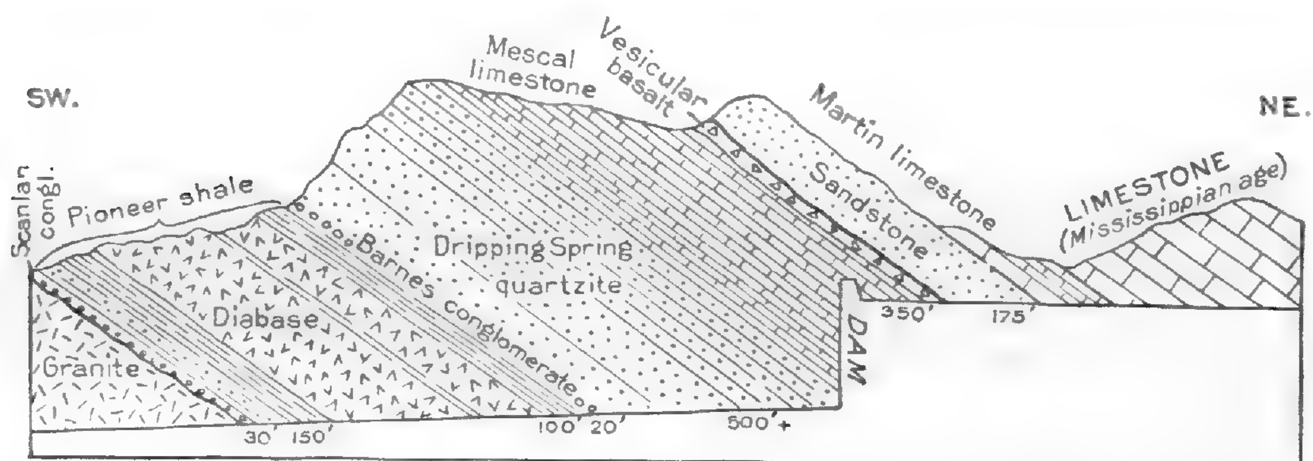
FIGURE 57.—Section at Roosevelt Dam, Ariz.
