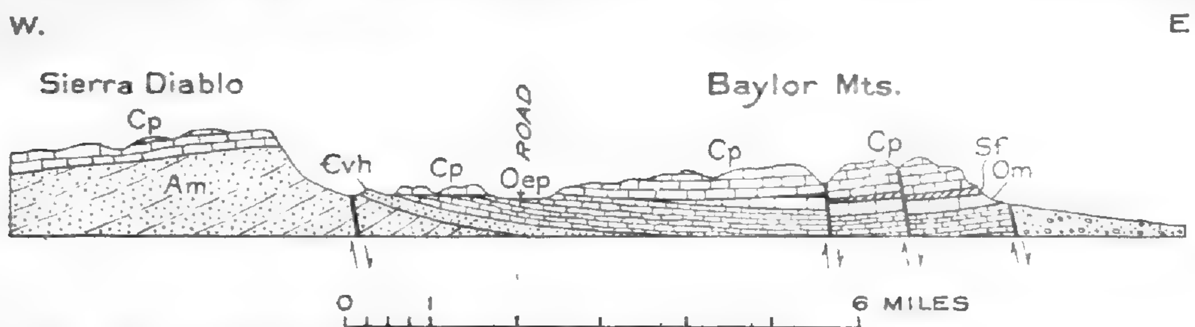
FIGURE 19.—Section across the escarpment of the Sierra Diablo and Baylor Mountains, 15 miles north of Van Horn, Tex. By P. B. King. Am, Millican formation; Cvh, Van Horn sandstone; Oep, El Paso limestone; Om, Montoya limestone; Sf, Fusselman limestone; Cp, limestones of Permian age
