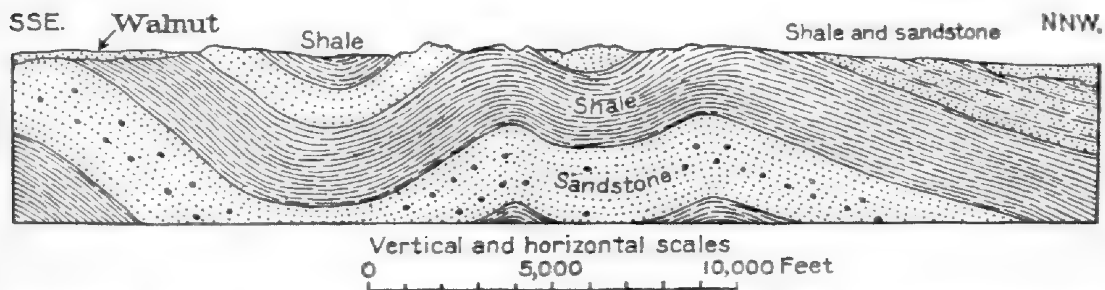
FIGURE 67.—Section of San Jose Hills about 7 miles west of Pomona, Calif. After English and Kew. All Puente formation
