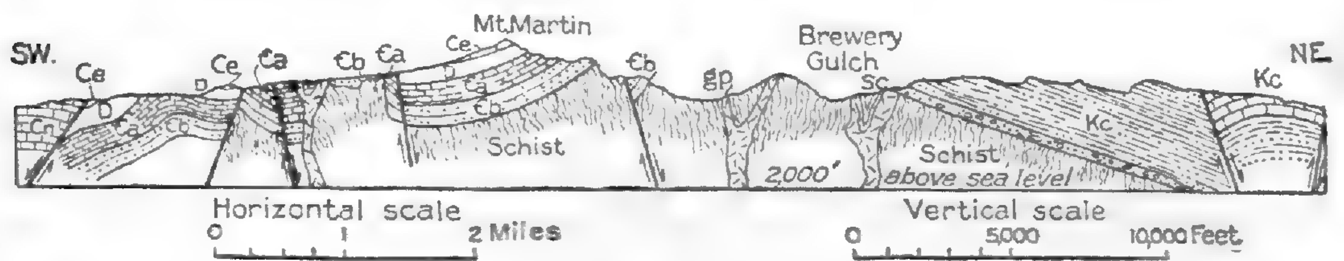
FIGURE 45.—Section across the Bisbee region, Ariz. Kc, Limestones, sandstones, shales, and conglomerate of Lower Cretaceous age (Comanche); Cn, Naco limestone; Ce, Escabrosa limestone; D, Martin limestone (Devonian); Ca, Abrigo limestone; Cb, Bolsa quartzite (Cambrian); sc, schist; gp, granite porphyry. After Ransome
