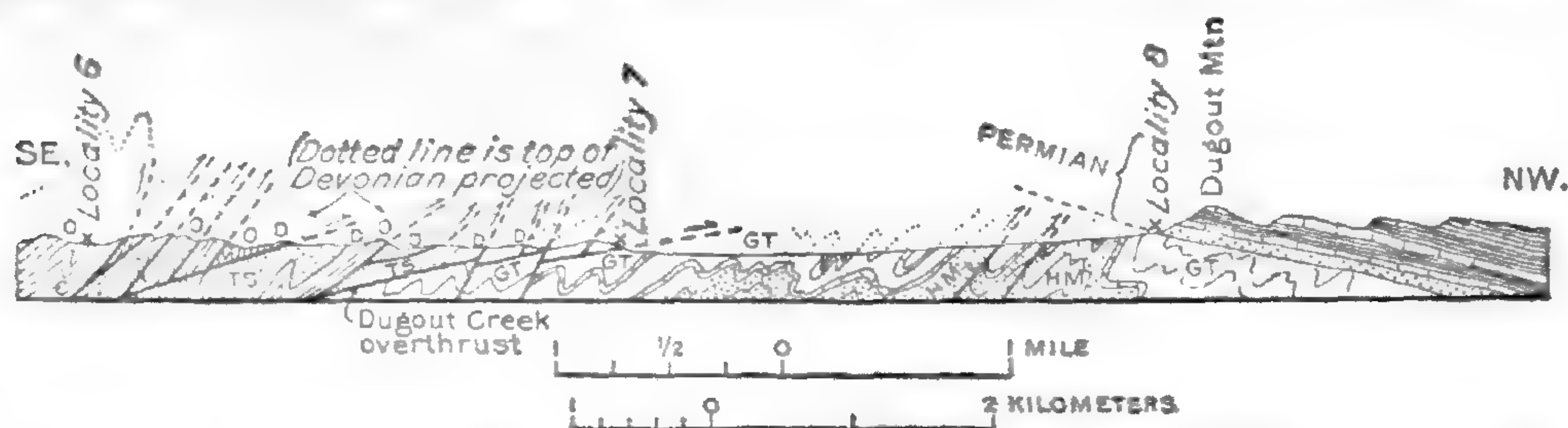
FIGURE 12.—Section southeast of Dugout Mountain, Tex., showing relations of the Dugout Creek overthrust. By P. B. King. C, Cambrian; O, Ordovician; D, Devonian; TS, Tesnus formation; HM, Haymond formation; GT, Gaptank formation
