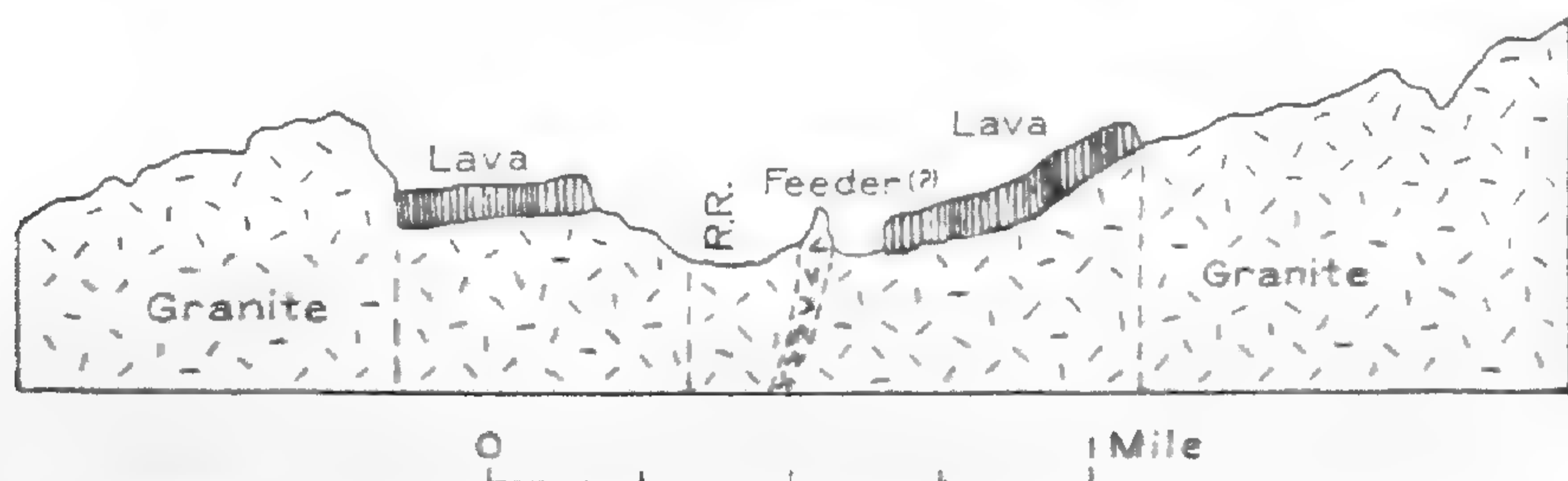
FIGURE 71.—Section about 2 miles north of Jacumba Springs, Calif.
