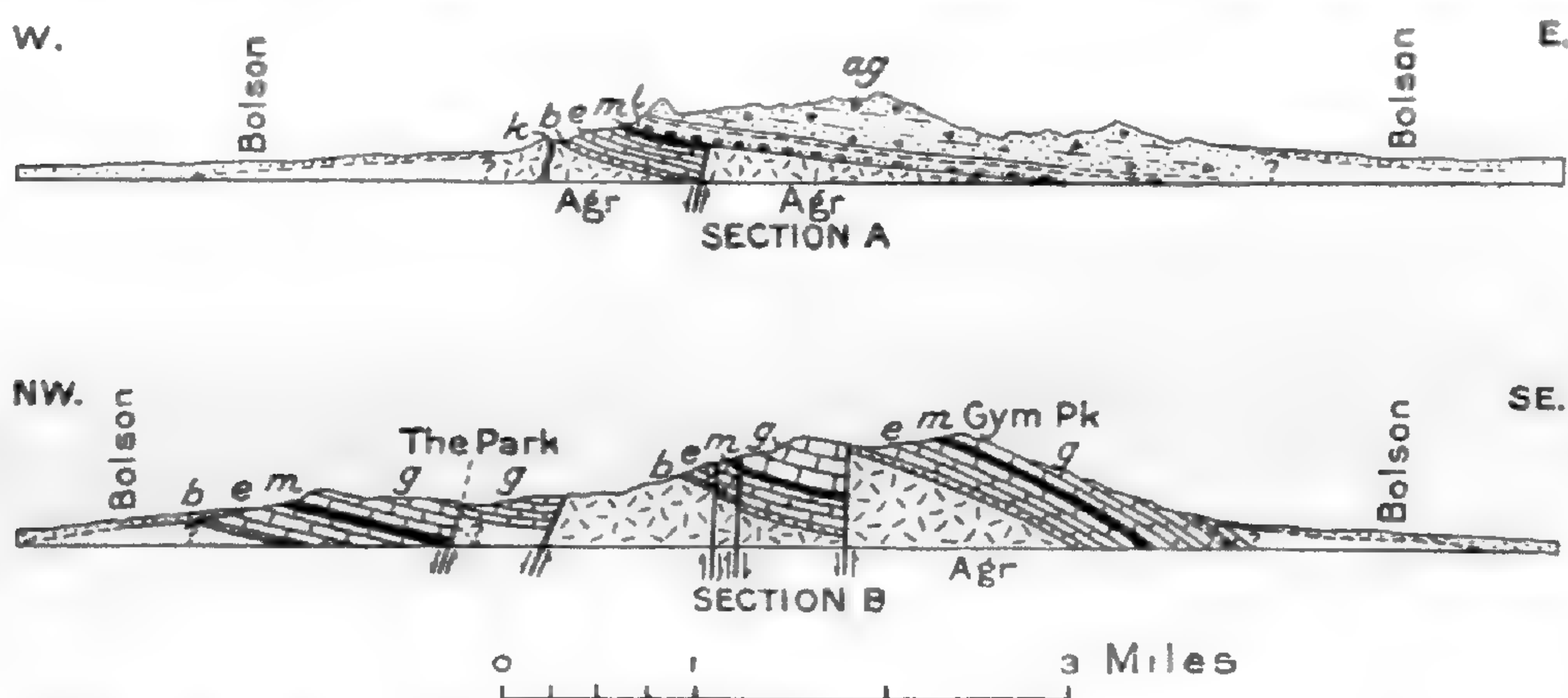
FIGURE 30.—Sections across Florida Mountains, Luna County, N. Mex. A, Through Capitol Dome, near the north end; B, through Gym Peak. b , Bliss sandstone; e , El Paso limestone; m , Montoya and Fusselman limestones; l , Lobo formation; g , Gym limestone; k , keratophyre dikes; Agr , granite; ag , volcanic agglomerate
