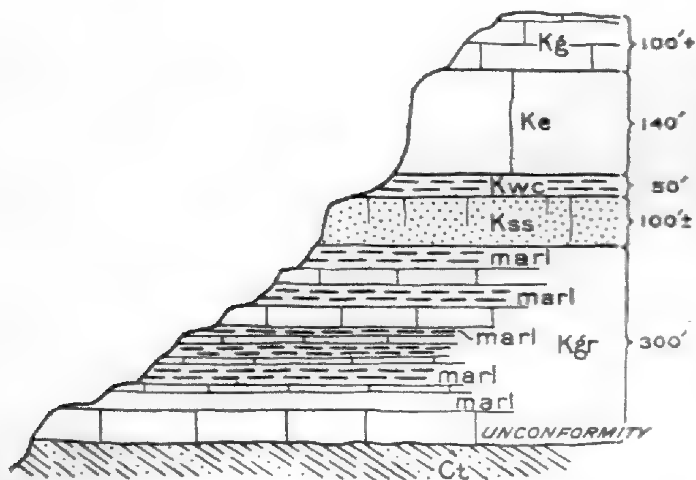
FIGURE 9.—Section near Maxon, Tex. Cretaceous: Kg, Georgetown limestone; Ke, Edwards limestone; Kwc, Walnut and Comanche Peak limestones; Kss, sandstone; Kgr, Glen Rose formation. Pennsylvanian: Ct, Tesnus formation
