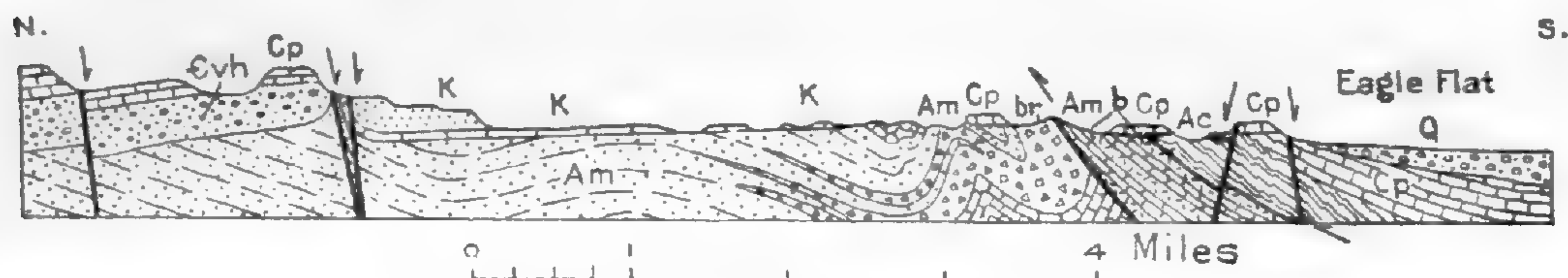
FIGURE 22. Section from the southern edge of the Diablo Plateau to Eagle Flat, east of the Sierra Blanca, Tex. By P. B. King. K, Sandstone and limestone (Cretaceous); Cp, limestone (Permian); Evh, Van Horn sandstone (Cambrian); Am, Millican formation (Algonkian), including breccia (br) and diabase (b); Ac, Carrizo Mountain schist; Q, Quaternary sand and gravel
