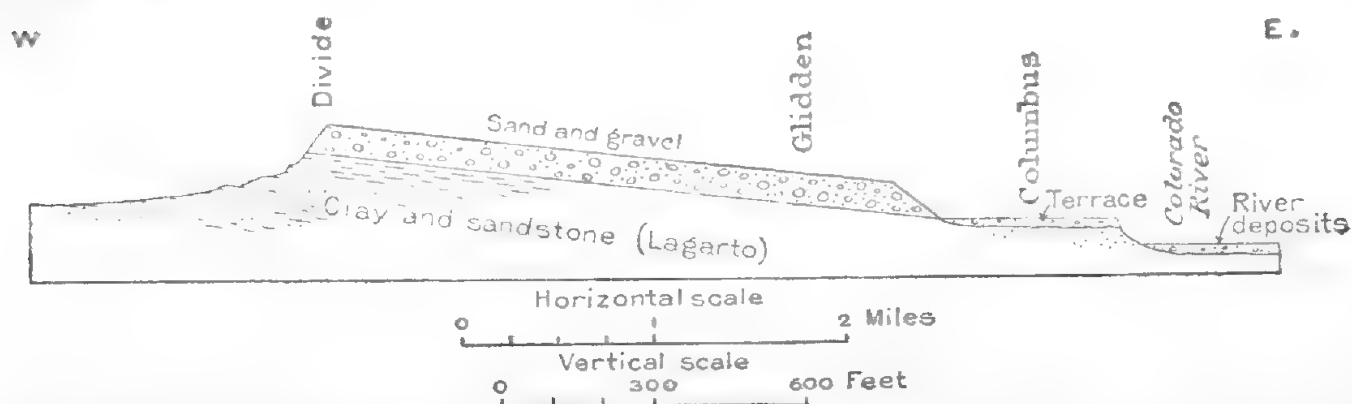
FIGURE 4.—Section along the Southern Pacific Railroad through Columbus and Glidden, Tex.
