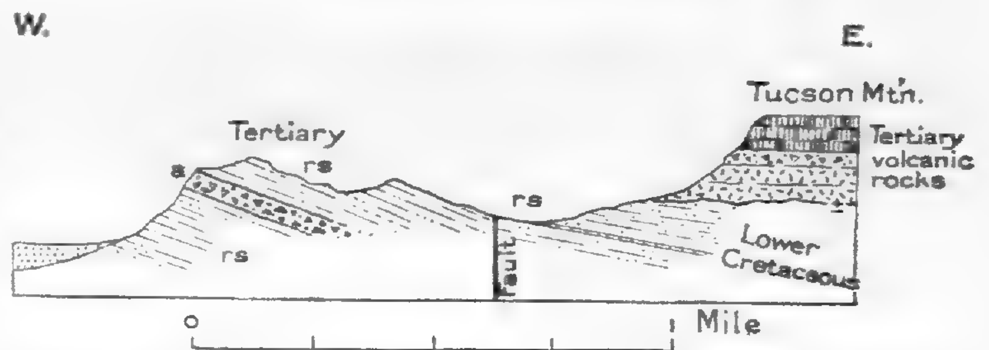
FIGURE 49. —Section of the west side of the Tucson Mountains, Ariz., about 3 miles south of the Ajo road, or 2 miles south of Amole Peak. a, Agglomerate; rs, red sandy shale
