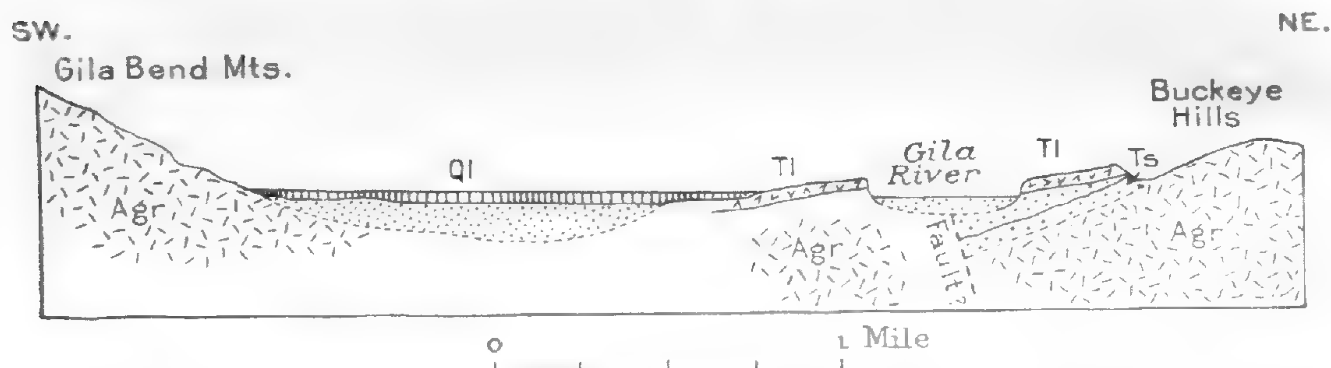
FIGURE 59.—Section across the valley of the Gila River at Gillespie Dam, Ariz. After C. P. Ross. Ql, Quaternary lava; Tl, Tertiary lava; Ts, Tertiary sandstone; Agr, granite
