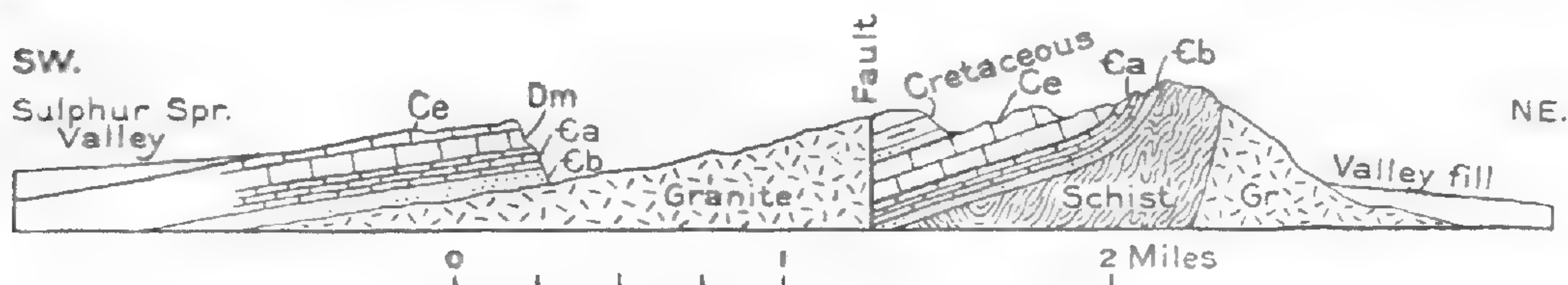
FIGURE 36.—Section of Dos Cabezas Mountains, Ariz. Ce, Escabrosa limestone; Dm, Martin limestone; Ca, Abrigo limestone; Cb, Bolsa sandstone; Gr, Granite
