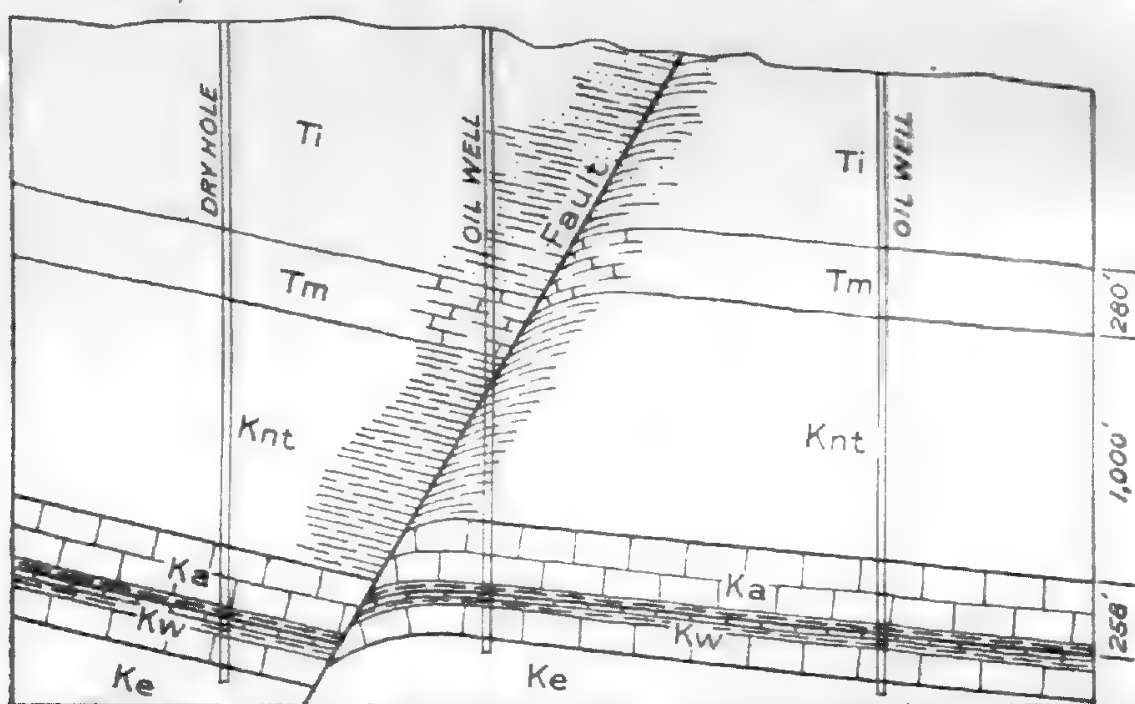
FIGURE 5.—Section across Salt Flat oil field, Caldwell County, Tex. Tertiary: Ti, Indio formation; Tm, Midway formation. Cretaceous: Knt, Navarro and Taylor clays; Ka, Austin chalk; Kw, Georgetown limestone overlain by Del Rio clay and Buda limestone; Ke, Edwards limestone
