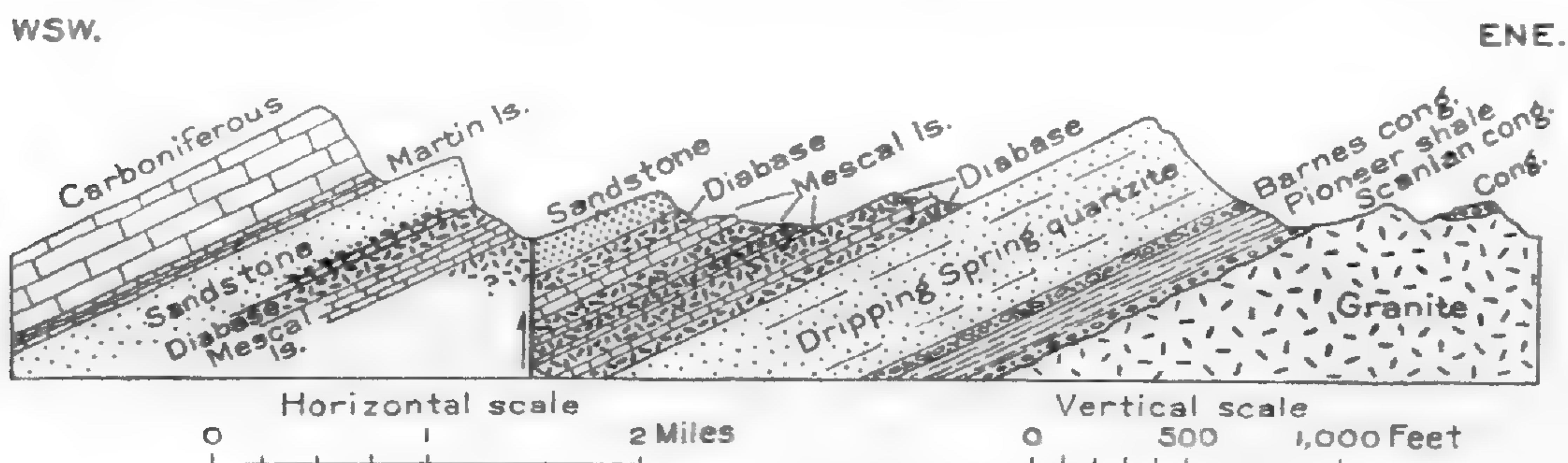
FIGURE 52.—Section across the center of Hayes Mountain, southwest of San Carlos, Ariz.
