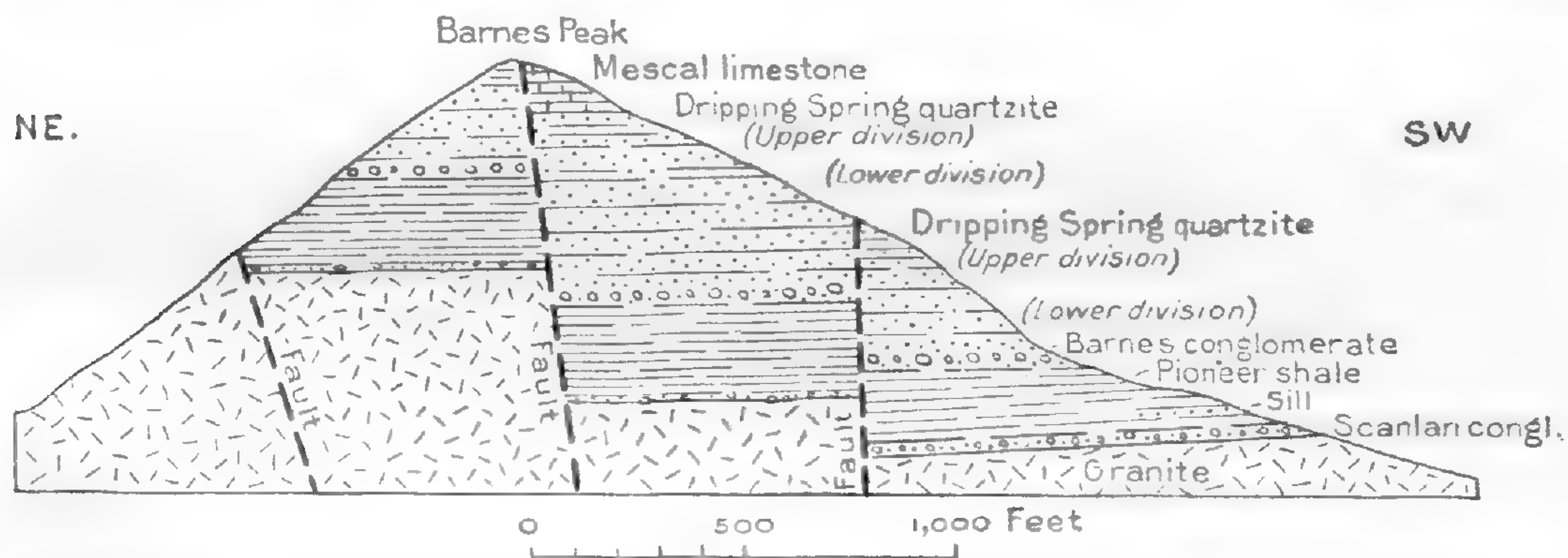
FIGURE 55.—Section showing relations of Apache strata 7 miles northwest of Miami, Ariz. By F. L. Ransome
