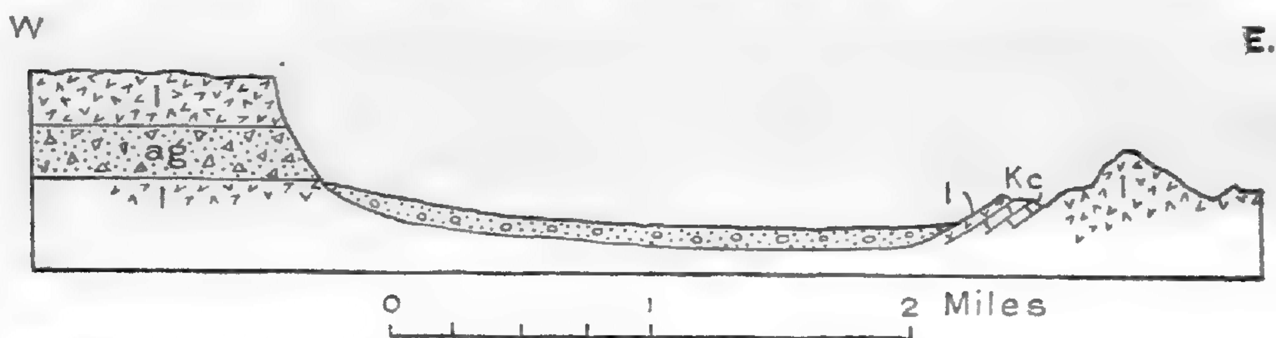
FIGURE 14.—Section across the Alpine Basin just north of Alpine, Tex. l, Lava (Tertiary); ag, agglomerate; Kc, limestone (Comanche).
