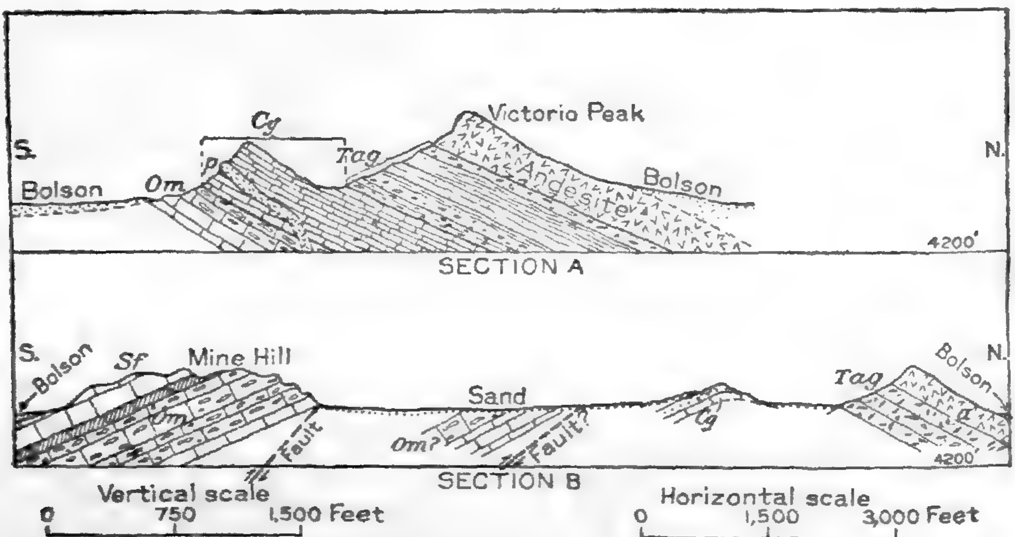
FIGURE 34.—Sections across Victorio Mountains, south of Gage, Luna County, N. Mex. a, Andesite; Tag, agglomerate, shale, and sandstone; Cg, Gym limestone (Permian); Sf, Fusselman limestone; Om, Montoya limestone; p, porphyry dike
