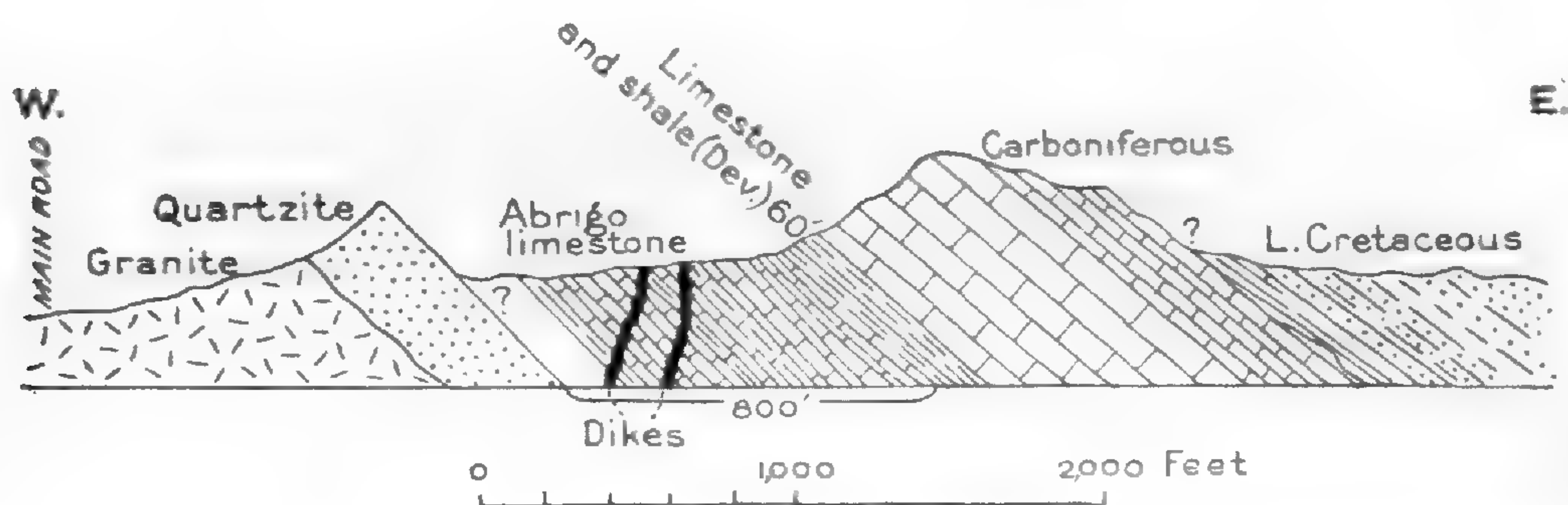
FIGURE 46.—Section 1 mile north of Helvetia mining camp, Ariz.
