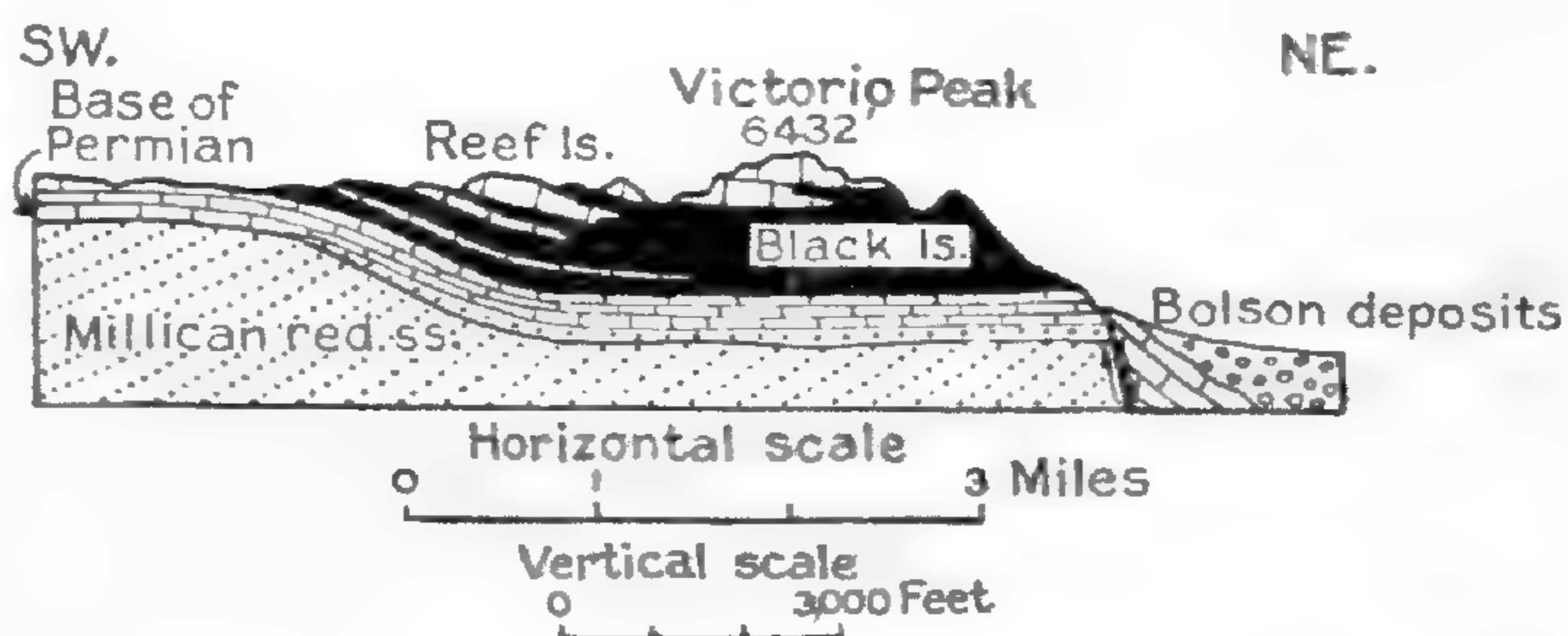
FIGURE 18.—Section of east front of Sierra Diablo at Victorio Peak, 18 miles north of Van Horn, Tex. By P. B. King
