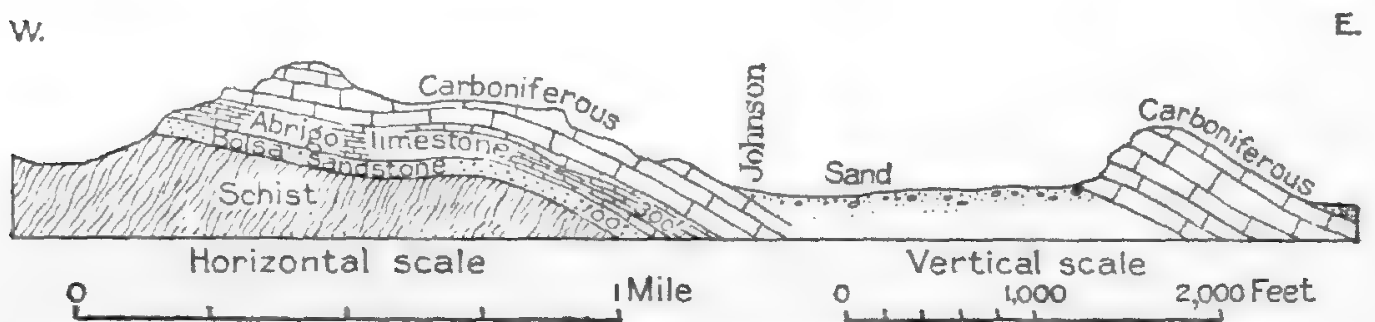
FIGURE 38.—Sketch section through the Johnson mining district, north of Dragoon station, Ariz.
