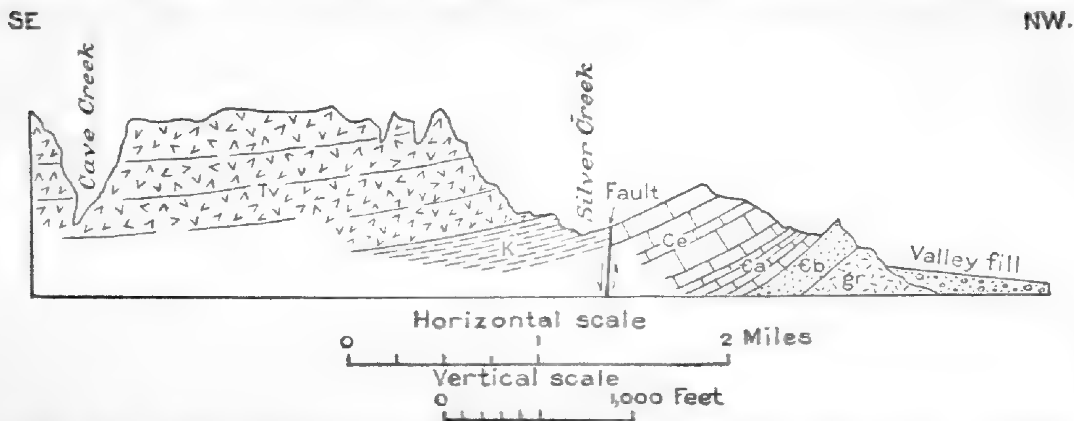
FIGURE 43.—Section of northeastern foothills of Chiricahua Mountains near Portal, Ariz. Cb, quartzite with sills of rhyolite (Cambrian); Ca, thin-bedded limestone and shale (Abrigo); Ce, limestone (Devonian and Carboniferous); K, sandstone, limestone, and shale (Comanche, Lower Cretaceous); Tv, lava (latite, Tertiary), dipping south at a low angle; gr, granite
