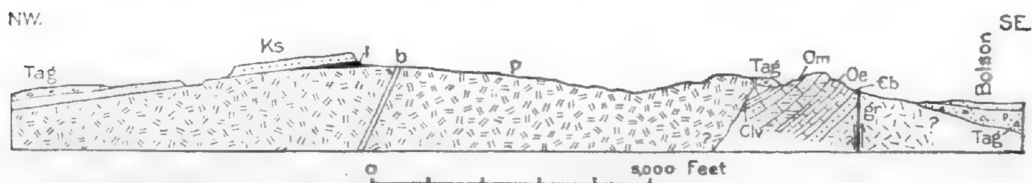
FIGURE 32.—Section across Fluorite Ridge, N. Mex. Tag, Agglomerate; Ks, Sarten sandstone; l, Lobo formation; Clv, Lake Valley limestone; Om, Montoya limestone overlain in part by limestone of undetermined age; Oe, El Paso limestone; cb, Bliss sandstone, gr, granite and diorite; p, porphyry; b, diabase dike
