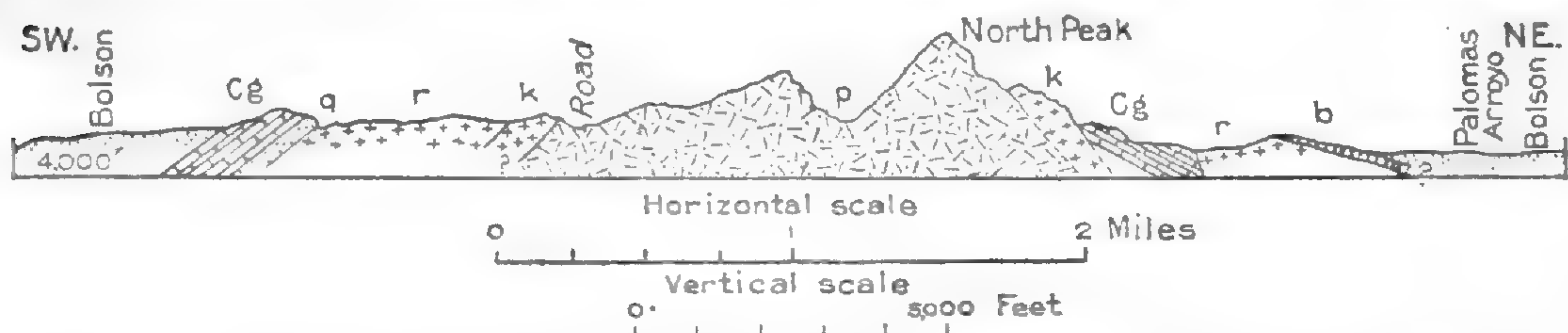
FIGURE 41.—Section across Tres Hermanas Mountains, Luna County, N. Mex. Cg, Gym limestone (Permian); p, porphyry; r, rhyolite; b, basalt; q, quartzite; k, keratophyre
