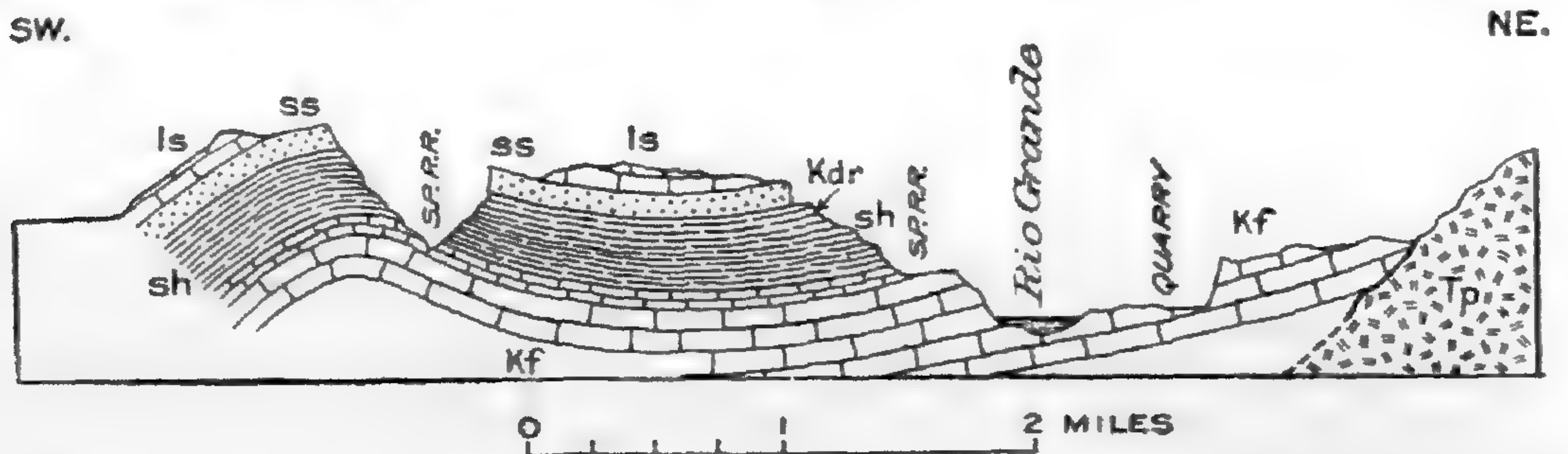
FIGURE 27.—Section southwest from cement quarry 2 miles west of El Paso, Tex. ls, Limestone, and ss, sandstone, of Upper Cretaceous age; Kdr, Del Rio horizon; sh, dark shale; Kf, Fredericksburg group; Tp, intrusive porphyry
