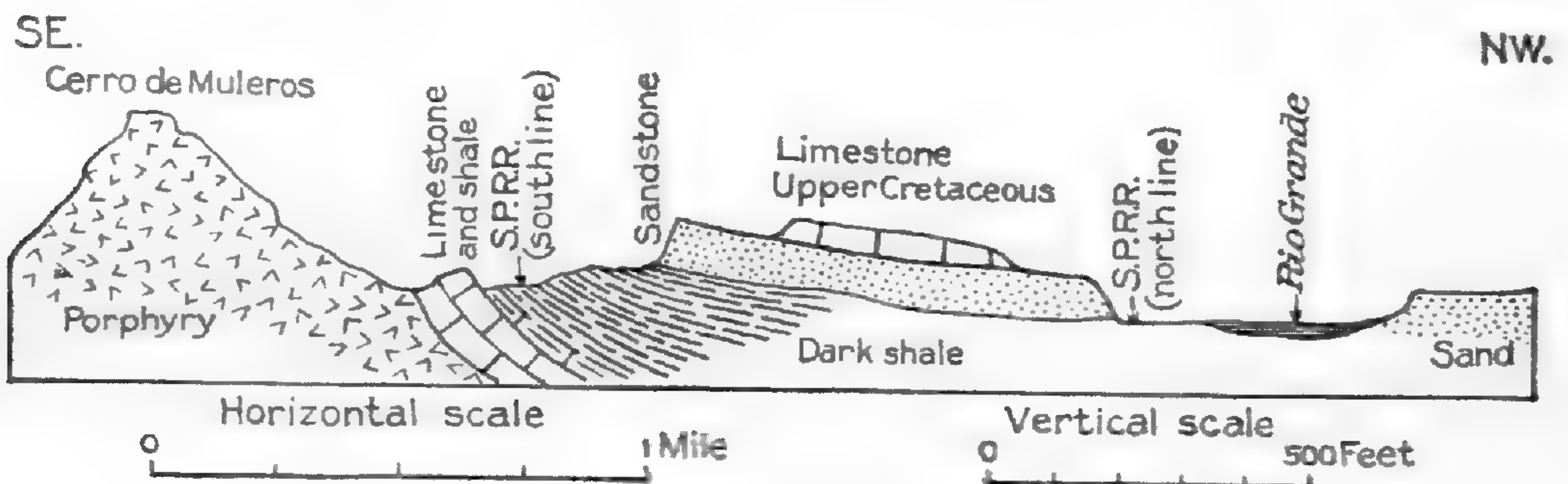
FIGURE 40.—Section through Bowen siding, New Mexico
