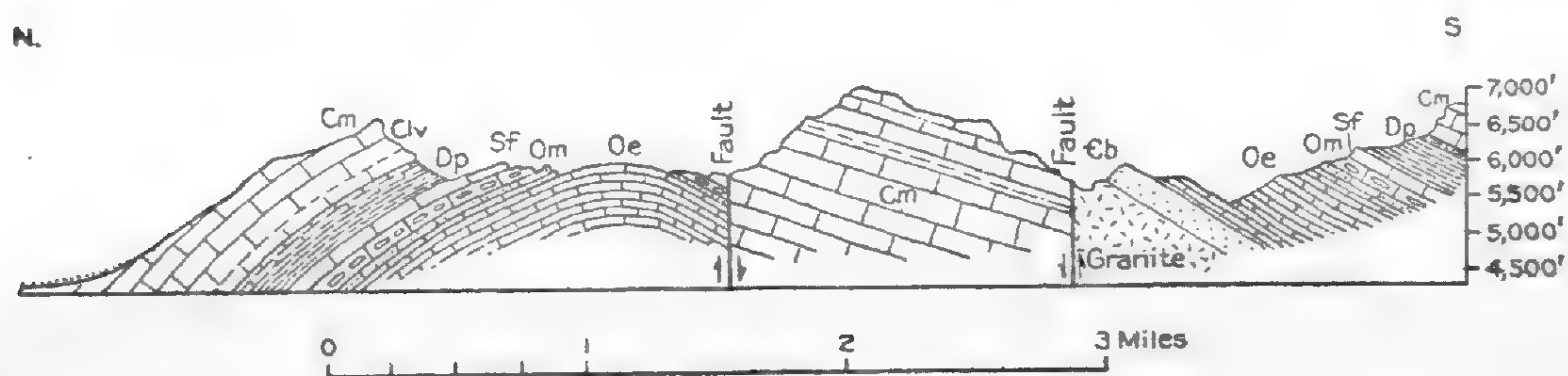
FIGURE 42.—Section across the north end of the Hatchet Mountains 20 miles south of Hachita, N. Mex. Cb, Bliss sandstone (Cambrian); Oe, El Paso limestone (Ordovician); Om, Montoya limestone (Ordovician); Sf, Fusselman limestone (Silurian); Dp, Percha shale (Devonian); Clv, Lake Valley limestone? (probably Mississippian); Cm, limestones of Magdalena group (Pennsylvanian)
