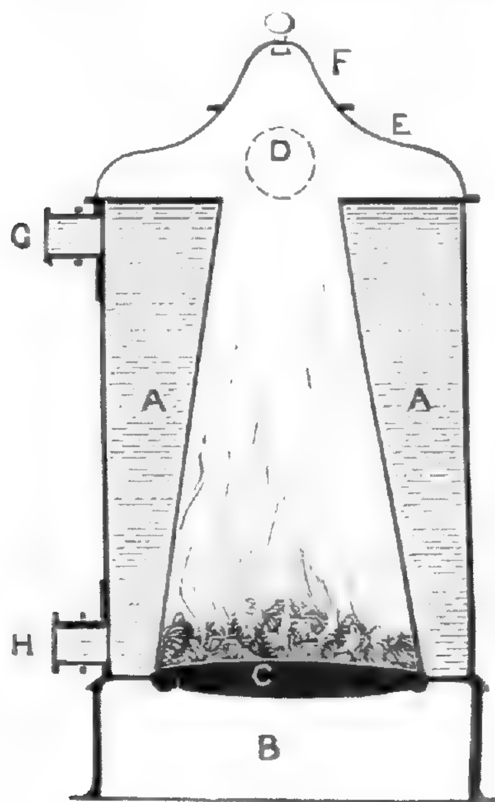
FIG. 260. VERTICAL SECTION OF CYLINDER BOILER.
