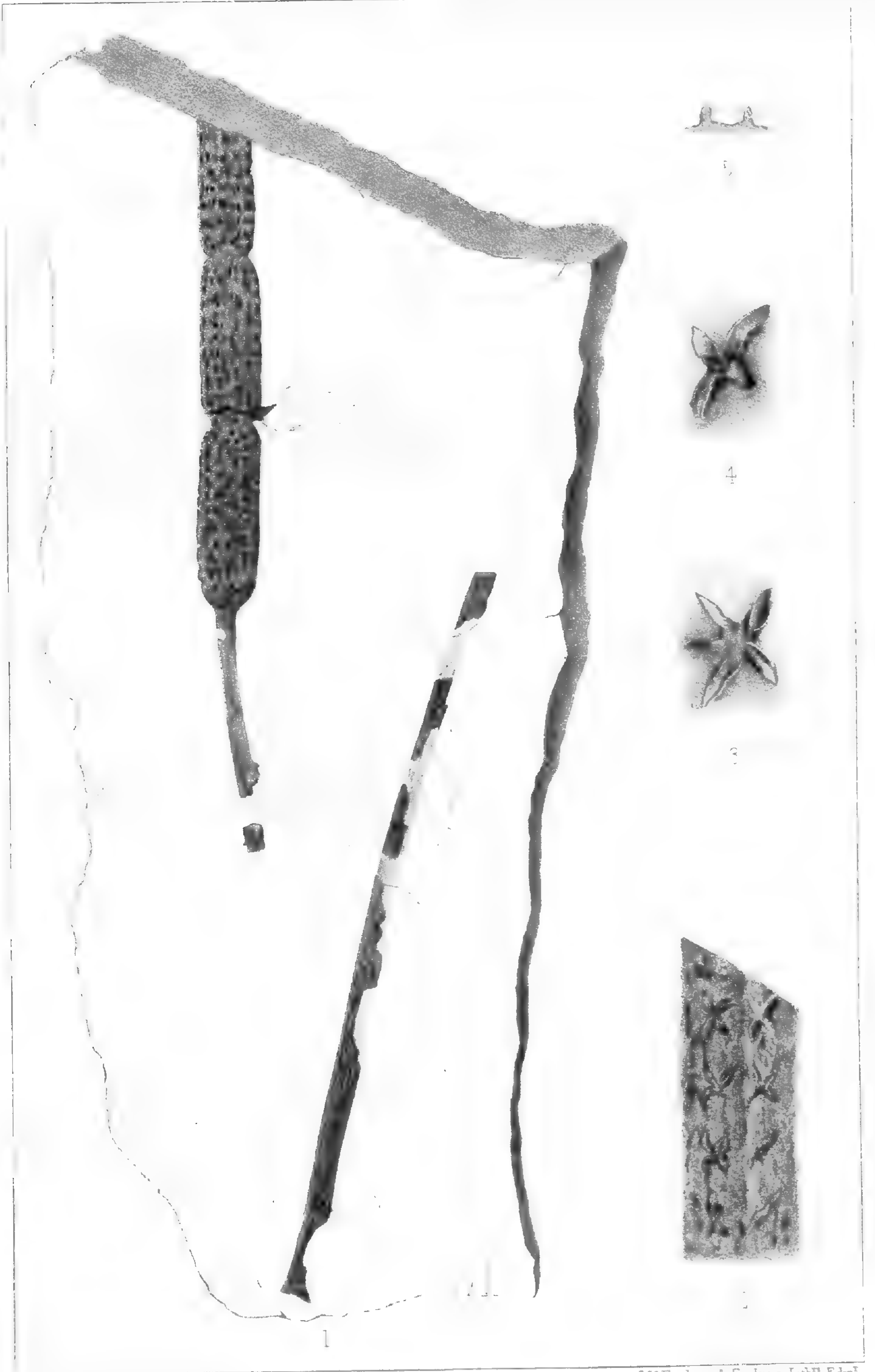
FRUIT OF BORNIA. Roem.
