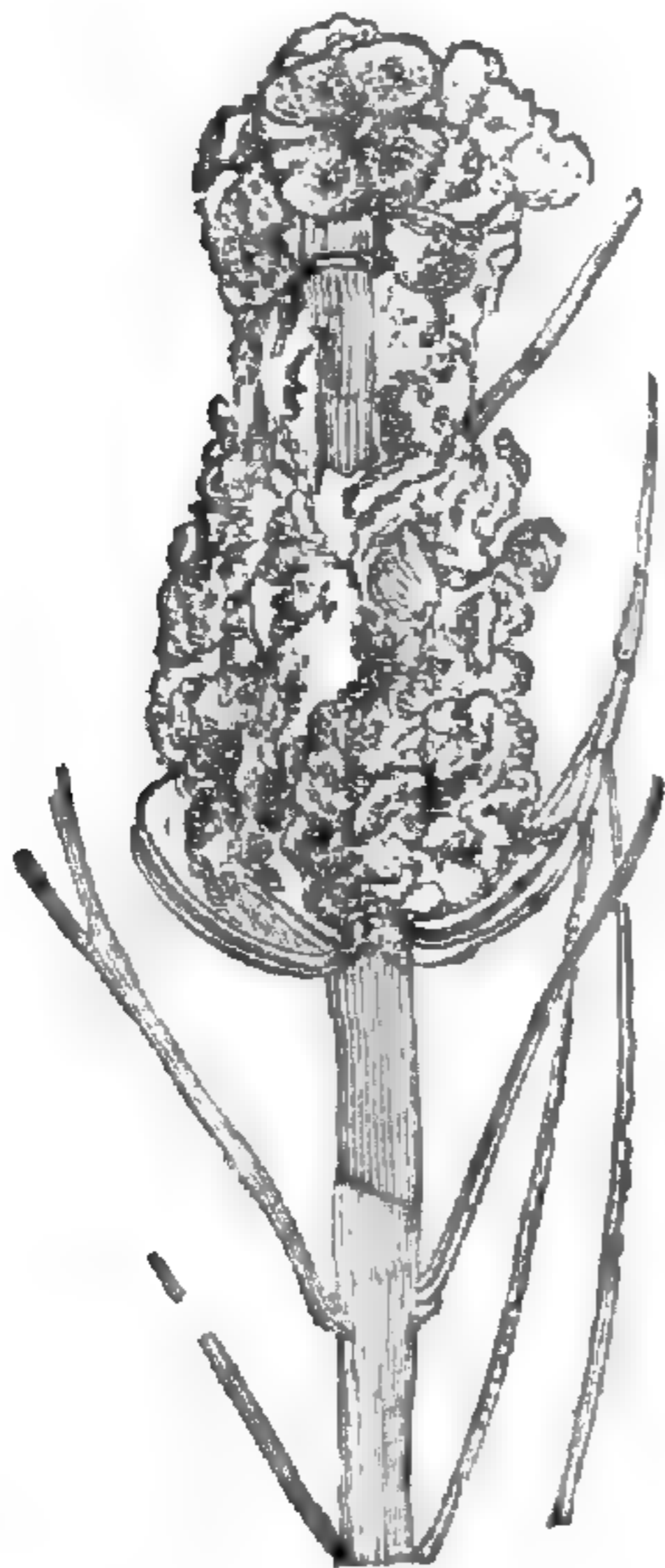
Fruit of Bornia ( Archæocalamites ) radiata , Brongn. (From Stur's 'Culm-Flora,' p. 129.)
