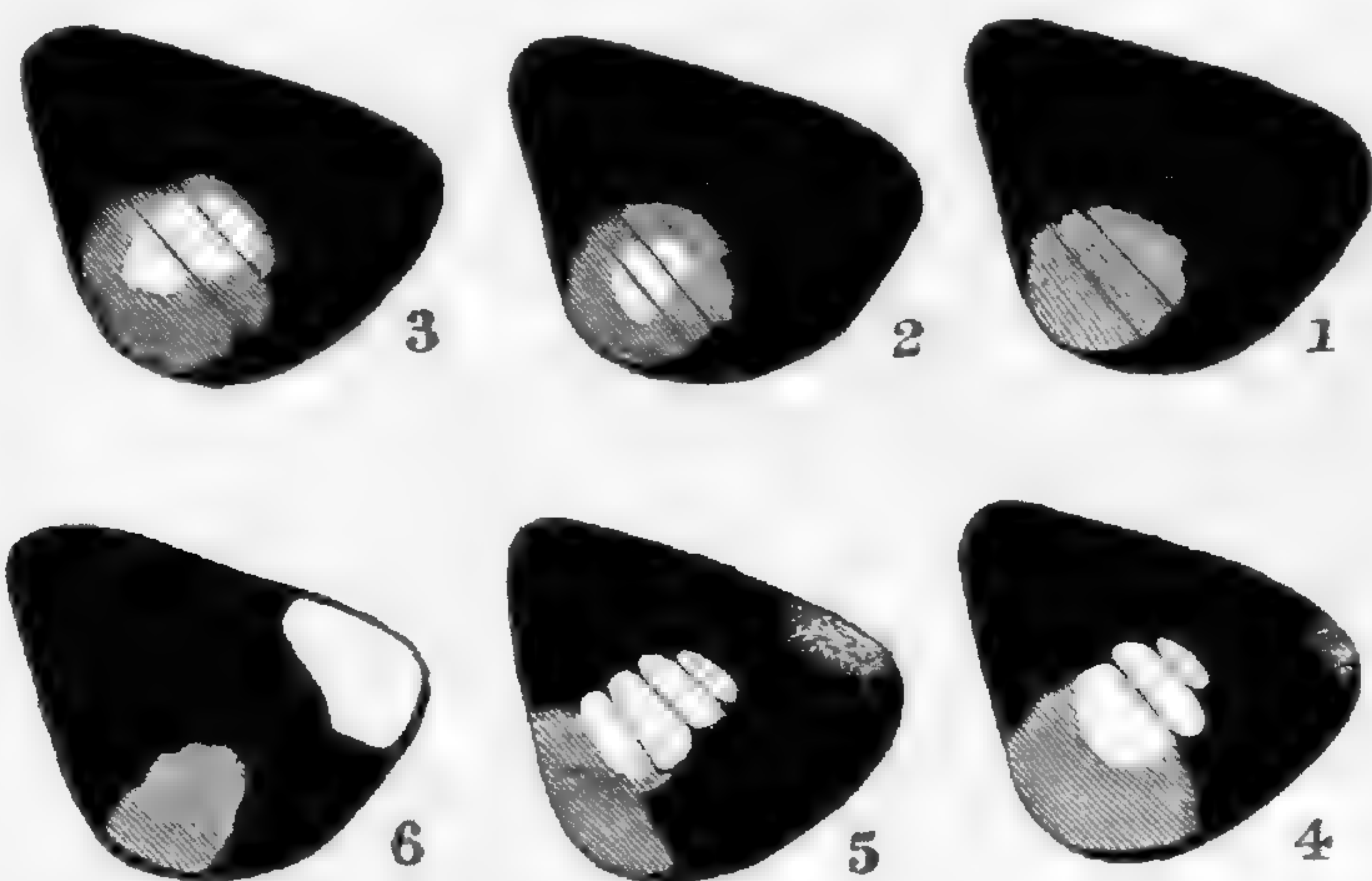
Hind wings of Phyllodes (reduced).
