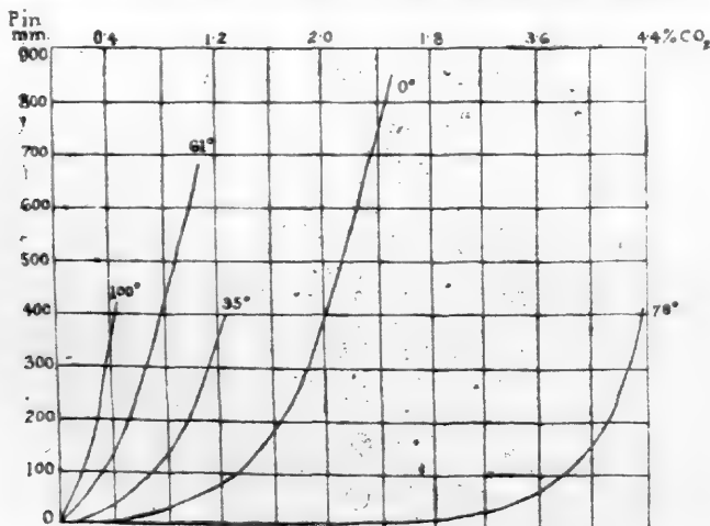
FIG. 1.—Absorption of carbon dioxide by charcoal.
