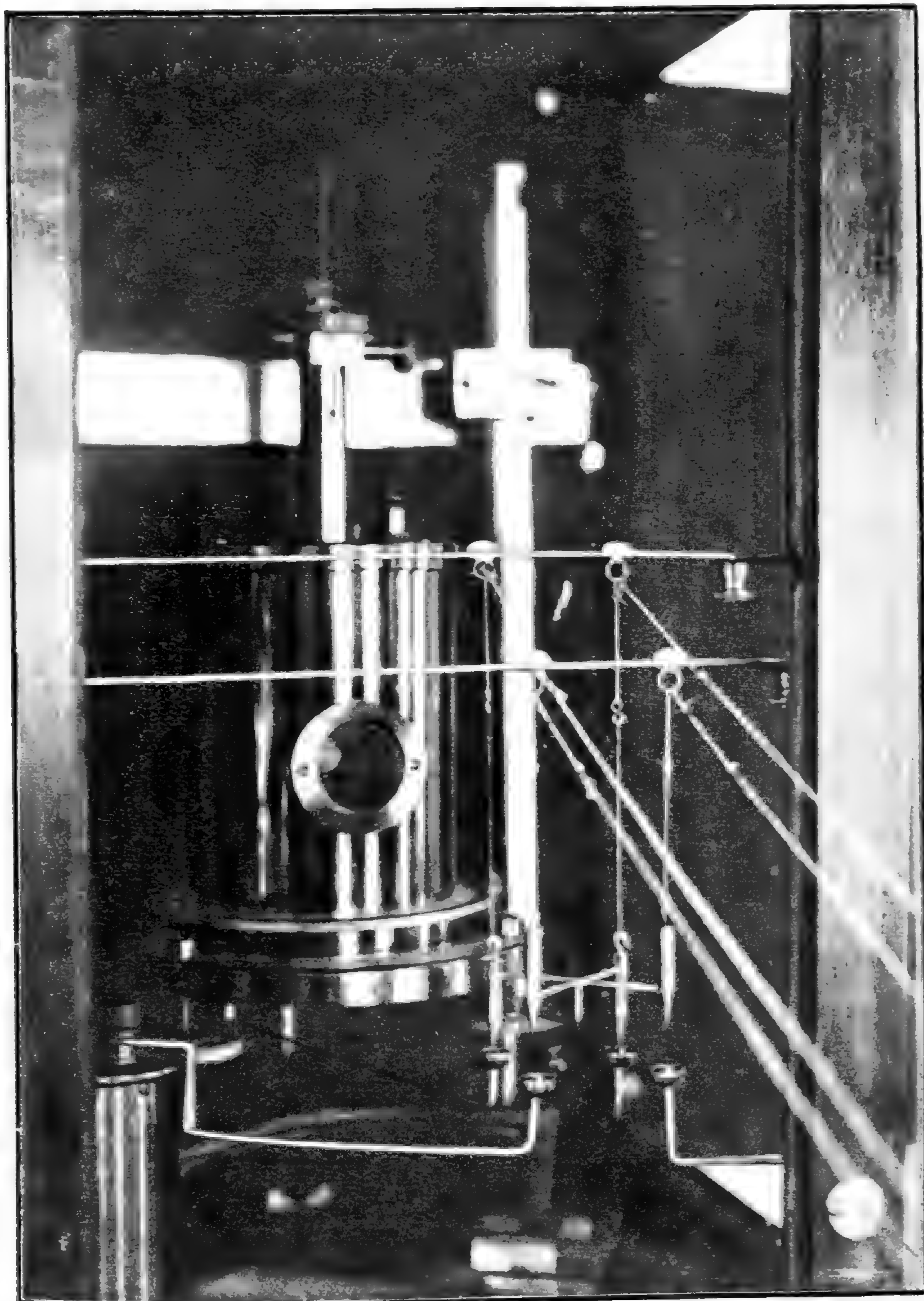
ARRANGEMENTS INSIDE CASE OF ELECTROMETER.
