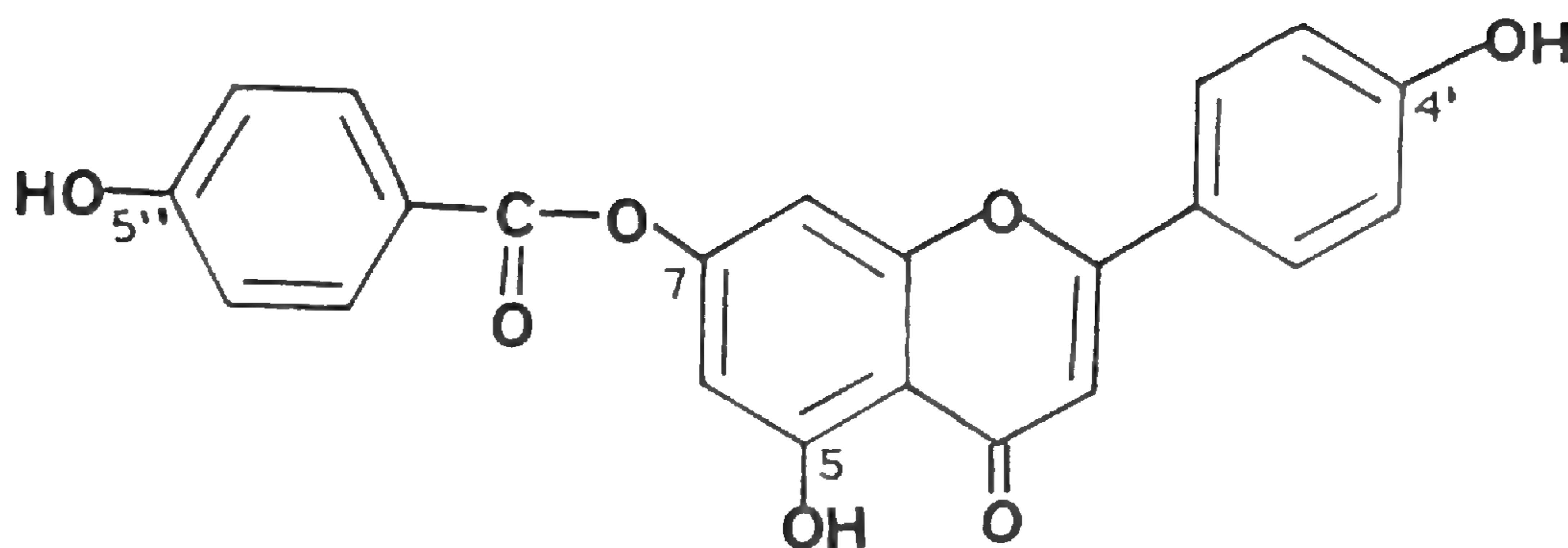
FIG. 1. Structure of Flavonoid I.
