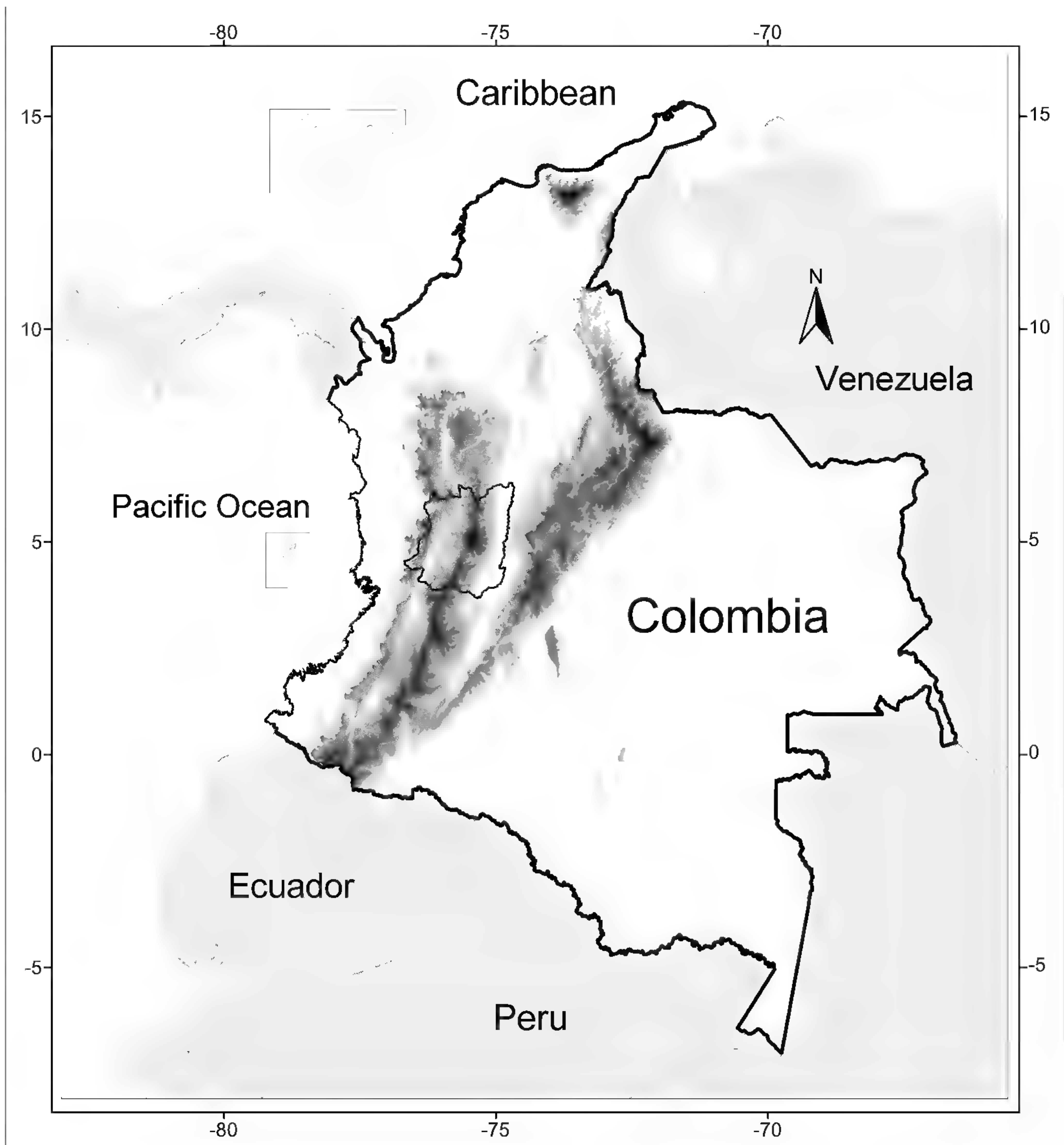
Figure 2. Topographic map of Colombia showing the location of the SIRAP Eje Cafetero (dark line).
