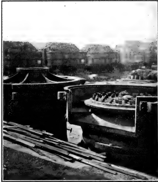
Paris—Machinery for Grinding Refuse and Railway Cars for transporting it to rural districts to be used as fertilizer for sugar-beets.
