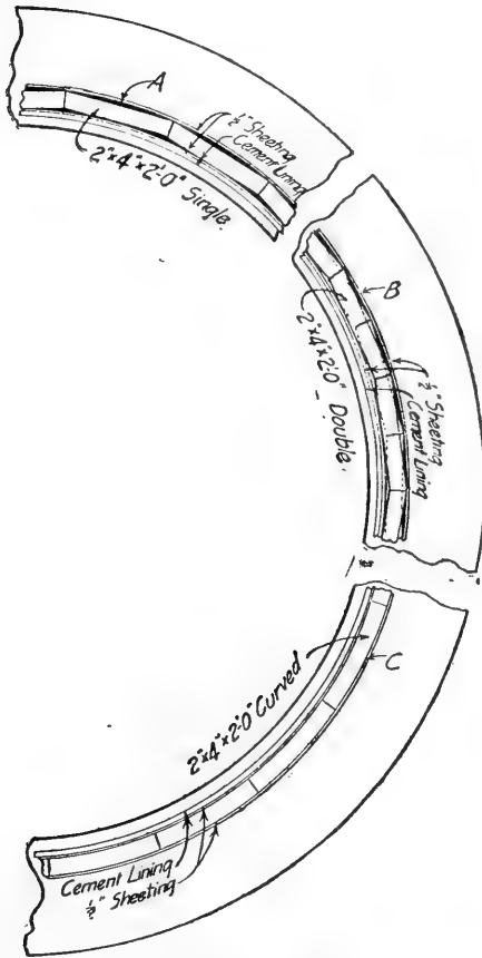
Fig. 2. —Showing three methods of making a sill or plate for Gurler or King Silo. A shows sill made of a single thickness of 2x4's cut in two-foot lengths; B shows sill made of two thicknesses of 2x4's laid to break joints; C shows 2x4 sawed out of 2x6 plank. C is the best method, since the sheathing then fits the sill making a tight joint, whereas in A and B a tight joint between sheathing and sill or plate cannot be secured. Observe that the sill is placed near the inner edge of the foundation.
