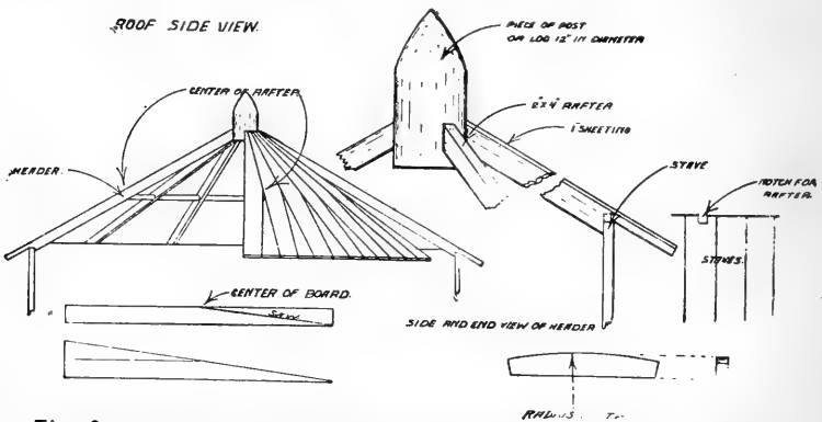
Fig. 9.—Showing construction and details of one style of roof. (From Nebr. Bul. No. 138.)
