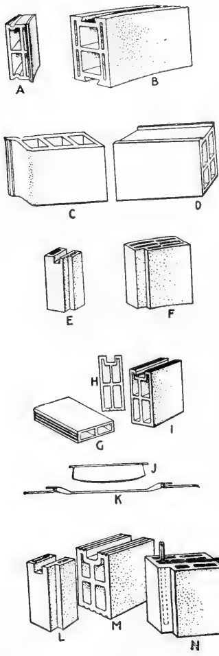
Fig. 43.—Group of Patented Clay Blocks of various manufacturers.
