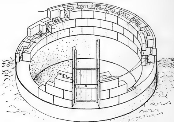
Fig. 36.—Showing how the two-piece cement block is laid in the wall and the door frame.
