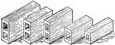
Fig. 47. —Five types of clay blocks which can be used for silo construction. "A" is 5"x8"x24"; "B" is 5"x8"x16"; "C" is 4"x8"x16"; "D" is 5"x5"x16"; and "E" is 4"x5"x16". (Cuts from Nebraska Bulletin No. 158.)
