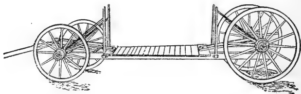
Fig. 52.—Low-down rack for hauling fodder corn.
