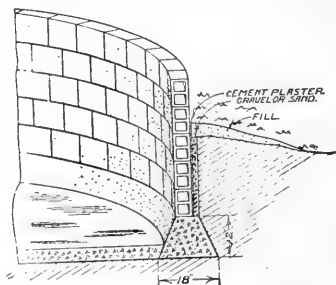
Fig. 46.—Clay block silo foundation. — (Nebraska Bulletin No. 138.)
