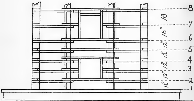
Fig. 22.—Skeleton showing method of framing.
