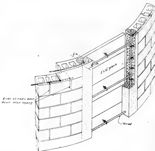
Fig. 59.—Continuous door opening for concrete block silo. View shows the manner of fastening reinforcing rods to the door frames, also of anchoring rods around a block instead of lapping.
