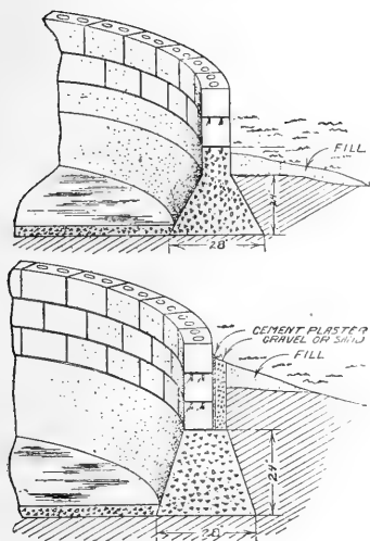
Fig. 40.—Two types of foundation for cement block silos.—Courtesy Nebraska Station.
