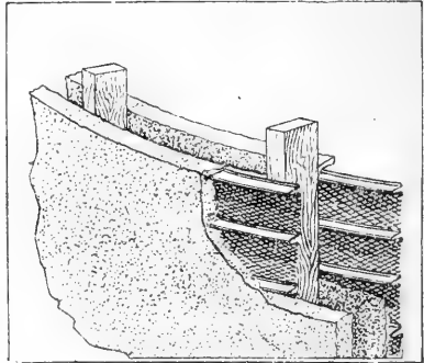
Fig. 54.—Showing double wall metal-lath silo.—Courtesy General Fireproofing Co., Youngstown.
