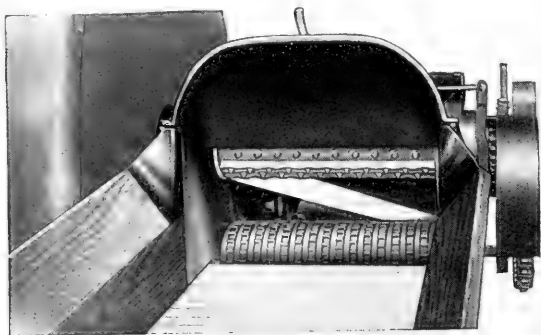
The sure, positive "bull-dog grip" of "Ohio" Feed Rollers is famous. The single lever gives absolute control of rolls and table, stopping, starting or reversing the feed at a touch.
