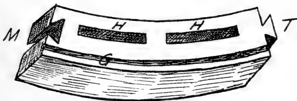
Fig. 37.—Illustrates a type of concrete block used in silo construction. H H are holes left in blocks. T and M are dove-tailed tenon and mortise so made that blocks interlock when laid on the wall. G is a groove made in block to imbed iron rod for reinforcing the wall.
