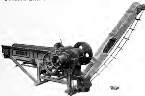
Metal Bucket Carrier, Straight or Swivel Delivery, for "Ohio" Monarch Silo Fillers Nos. 12, 15 and 17.
