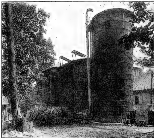
Fig. 53. —Shows Silver's No. 19 "Ohio" Monarch Self Feeder Blower Silage Cutter filling a group of five silos, owned by S. M. Shoemaker, Burnside, P. O., Eccleston, Md. The machine had just completed storing 1700 tons of silage.
