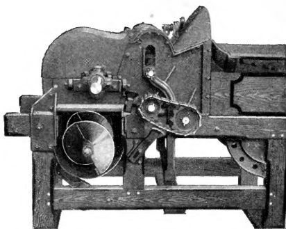
Auger side of machine with fan case removed. The auger prevents feed from entering blower in bulky, irregular quantities.
