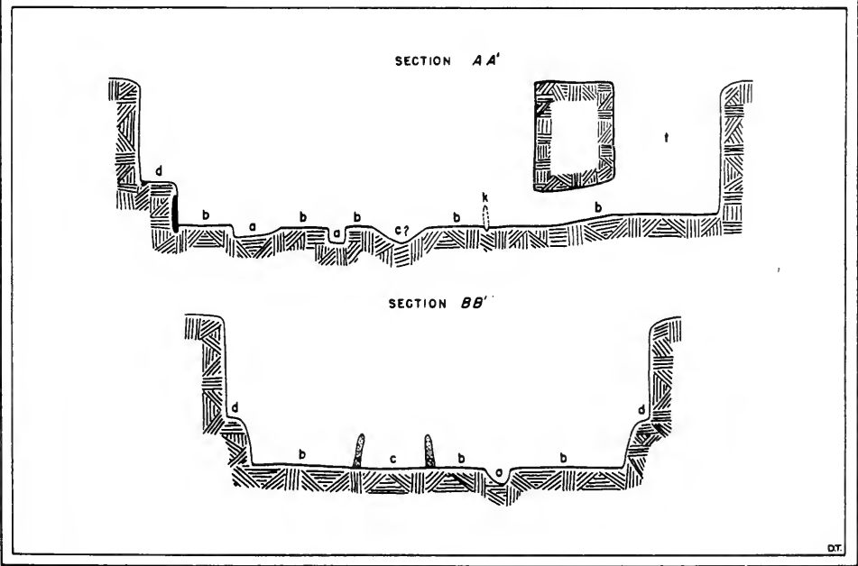
MAP 25. GROUND PLAN AND SECTIONS OF PIT HOUSE G, SITE 2
