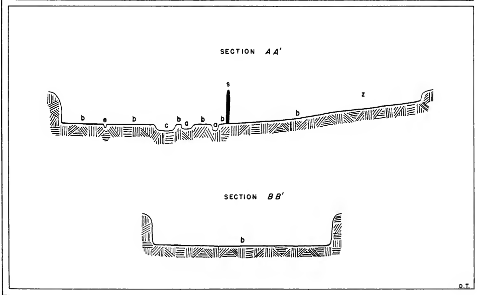
MAP 23. GROUND PLAN AND SECTIONS OF PIT HOUSE C, SITE 2
