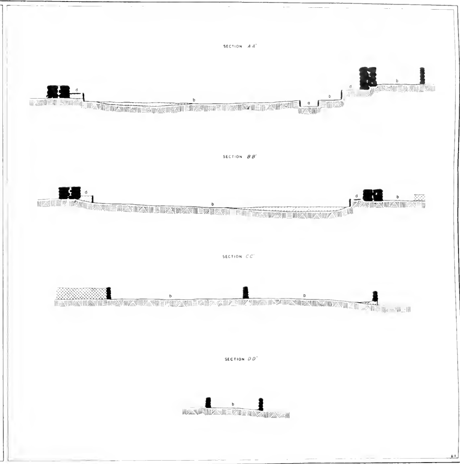
MAP 17. GROUND PLAN AND SECTIONS OF GREAT KIVA I AND PERIPHERAL ROOMS, SITE 1
