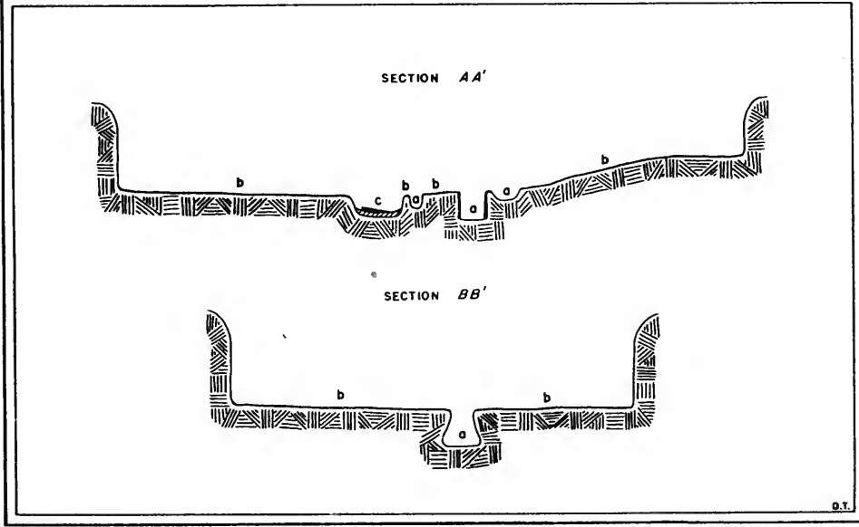
MAP 22. GROUND PLAN AND SECTIONS OF PIT HOUSE B, SITE 2
