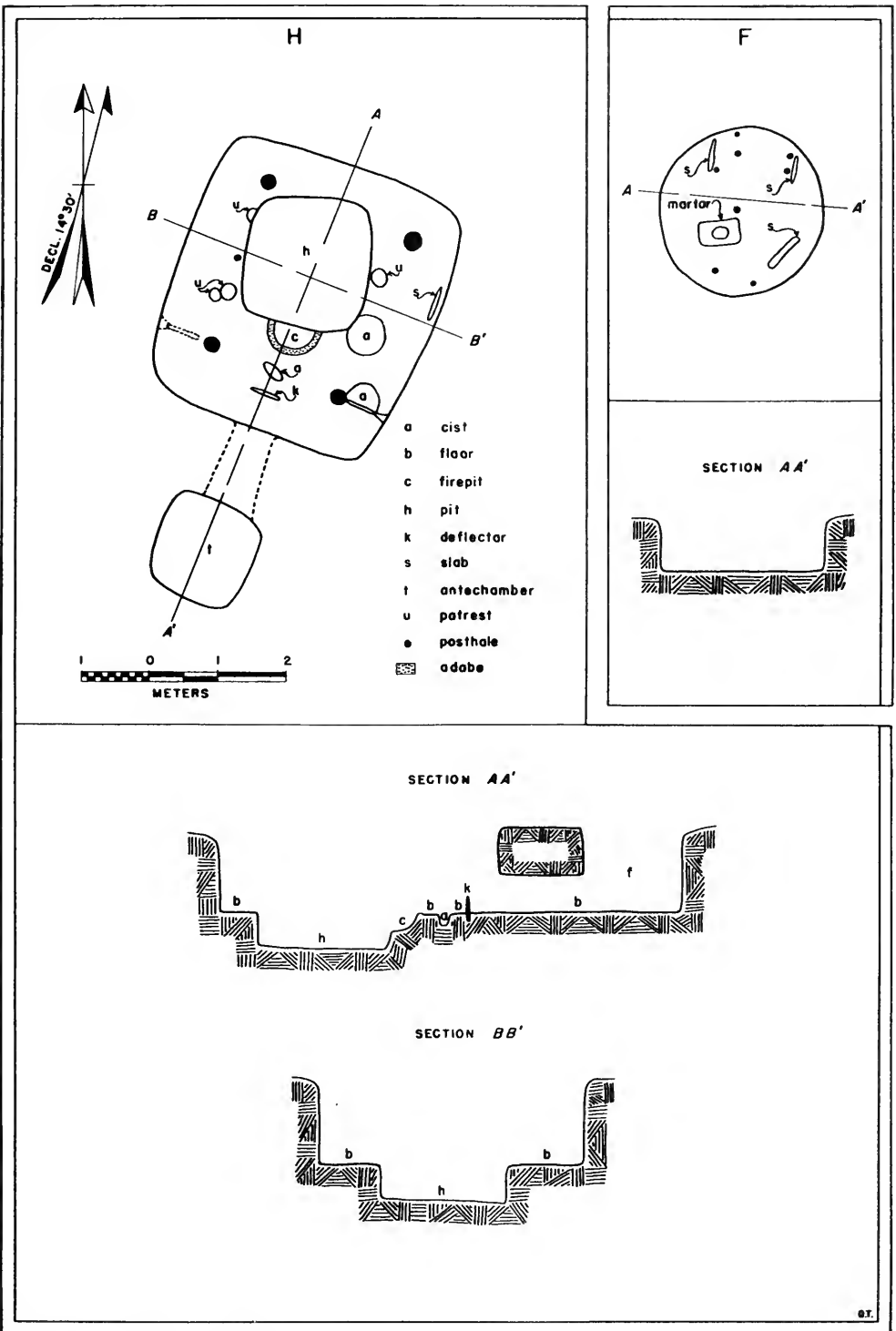
MAP 26. GROUND PLAN AND SECTIONS OF PIT HOUSE H AND CIRCULAR, SUBTERRANEAN PIT F, SITE 2
