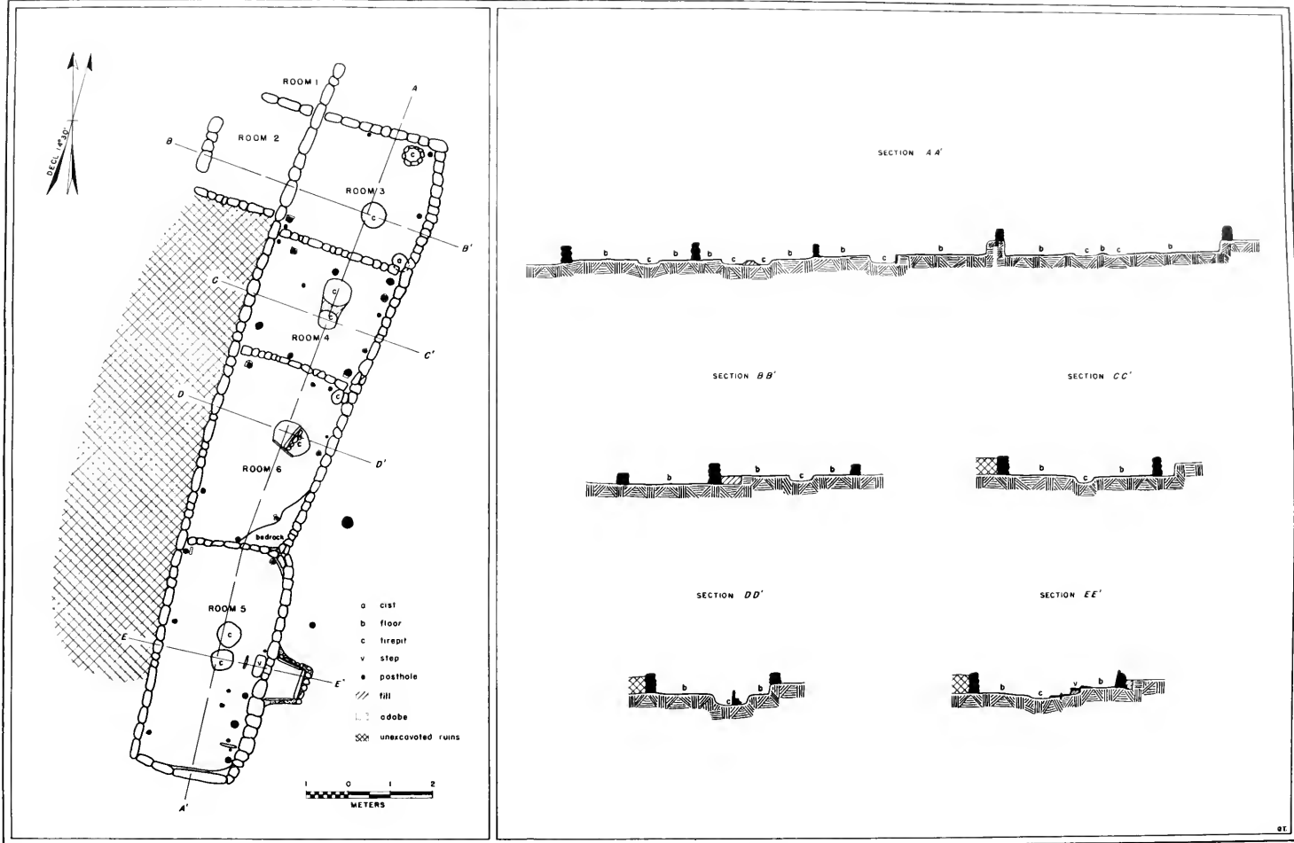
MAP 12. GROUND PLAN AND SECTIONS OF HOUSE GROUP I, SITE 1
