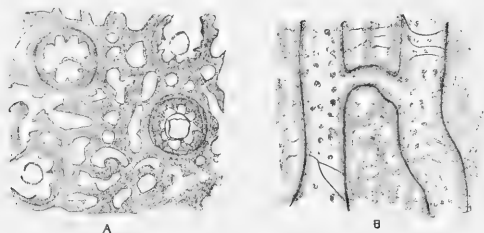
FIG. 17.—Sections of a species of Stromatopora , from the Devonian Limestone of Gerolstein, enlarged twelve times, showing " Caunopora -tubes" with septal spines. A. Tangential section. B. Vertical section
