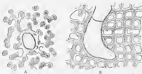
FIG. 16.—A. Tangential section of Hermatostroma Schlüterii , n. sp., enlarged twelve times. B. Vertical section of the same, similarly enlarged. Both sections intersect one of the large thin-walled tubes which are found at intervals in this species.
