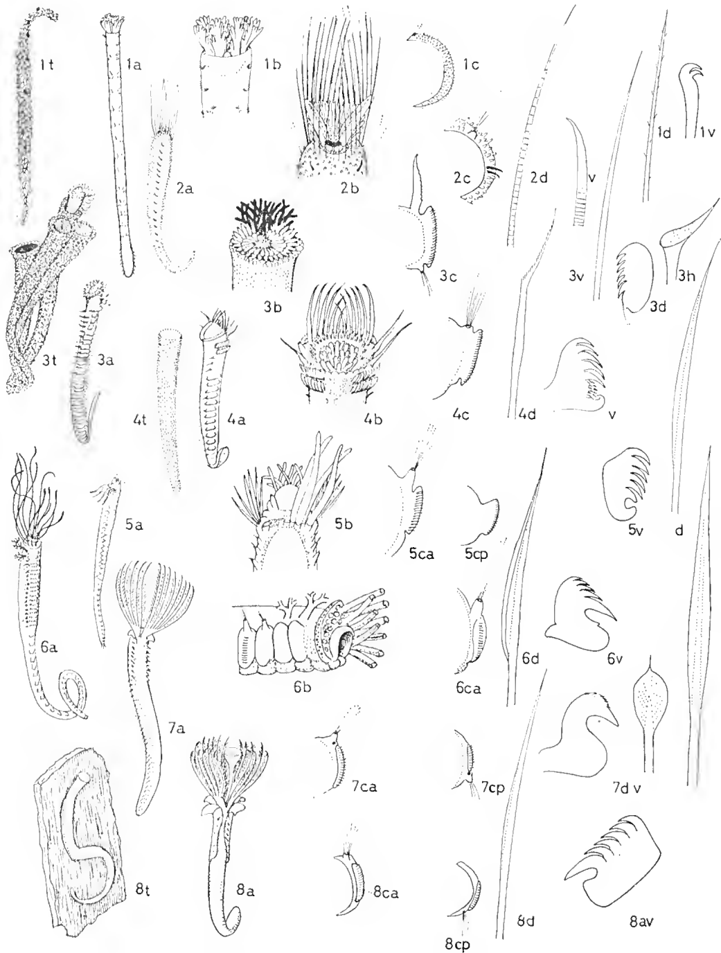
FIG. 0.6. Illustrations of Family Characters. 1, Oweniidae. 2, Flabelligeridae. 3, Sabellariidae. 4, Pectinariidae. 5, Ampharetidae. 6, Terebellidae. 7, Sabellidae. 8, Serpulidae. (A) Entire worm. (B) Head. (CA) Anterior foot. (CP) Posterior foot. (D) Notoseta. (H) Palea from operculum. (T) Tubc. (V) Neuroseta.
