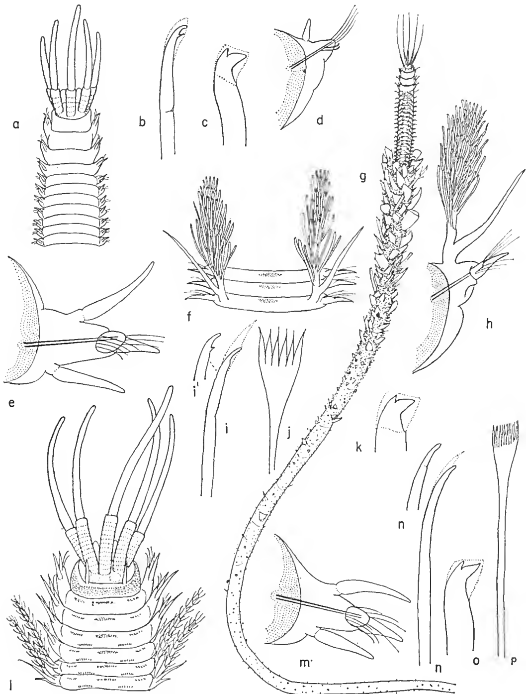
FIG. 17.10. Paronuphis antarctica . (A) Head. (B) Pseudocompound seta. (C) Acicular seta. (D) Middle foot. Diopatra neapolitana . (E) Anterior view of second foot. (F) Branchiferous region showing pigment pattern. (G) Tube (half natural size). (H) Seventh foot. (I) Pseudocompound seta. (J) Comb seta. (K) Acicular seta. Diopatra neapolitana capensis . (L) Head. (M) Anterior view of second foot. (N) Pseudocompound seta. (O) Acicular seta. (P) Comb seta.
