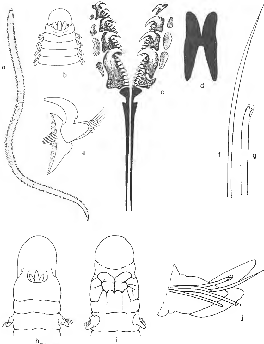
FIG. 17.14. Aglaurides fulgida . (A) Entire worm (half natural size). (B) Head. (C) Maxillae. (D) Mandibles. (E) Foot. (F) Capillary seta. (G) Acicular seta. Augneria tentaculata (after Monro 1930). (H) Dorsal view of head. (I) Ventral view of head. Ninoe lagosiana (after Augener). (J) Posterior foot with postsetal lobe and gill.
