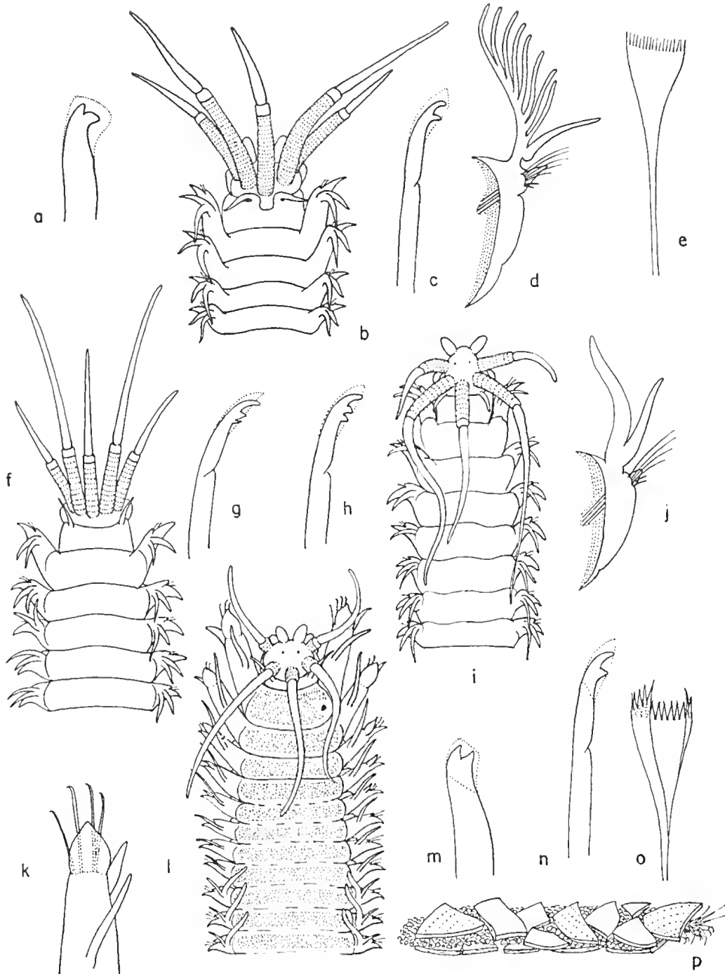
FIG. 17.13. Onuphis quinquedens . (A) Acicular seta. (B) Head. (C) Pseudocompound hook. (D) Middle foot. (E) Comb seta. Onuphis holobranchiata . (F) Anterior end. (G) Pseudocompound hook. Onuphis geophiliformis . (H) Pseudocompound hook. (I) Anterior end. (J) Twelfth foot. Onuphis conchylega . (K) Dorsal view of first foot. (L) Anterior end. (M) Acicular seta. (N) Pseudocompound hook. (O) Comb seta. (P) Tube.
