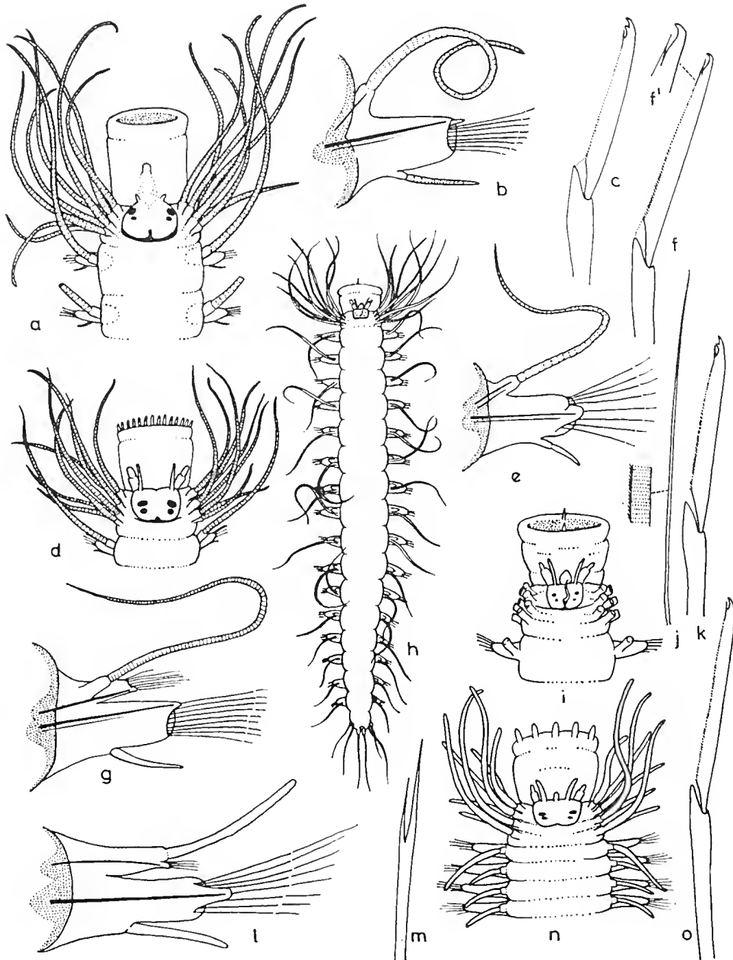
FIG. 11.2. Hesione splendida . (A) Head. (B) Foot. (C) Seta. Kefersteinia cirrata . (D) Head. (E) Foot. (F) Seta. Leocrates clapedii . (G) Tenth foot. (H) Entire worm (twice natural size). (I) Head. (J) Notoseta. (K) Neuroseta. Gyptis capensis . (L) Tenth foot. (M) Forked type of notoseta. (N) Head. (O) Neuroseta.
