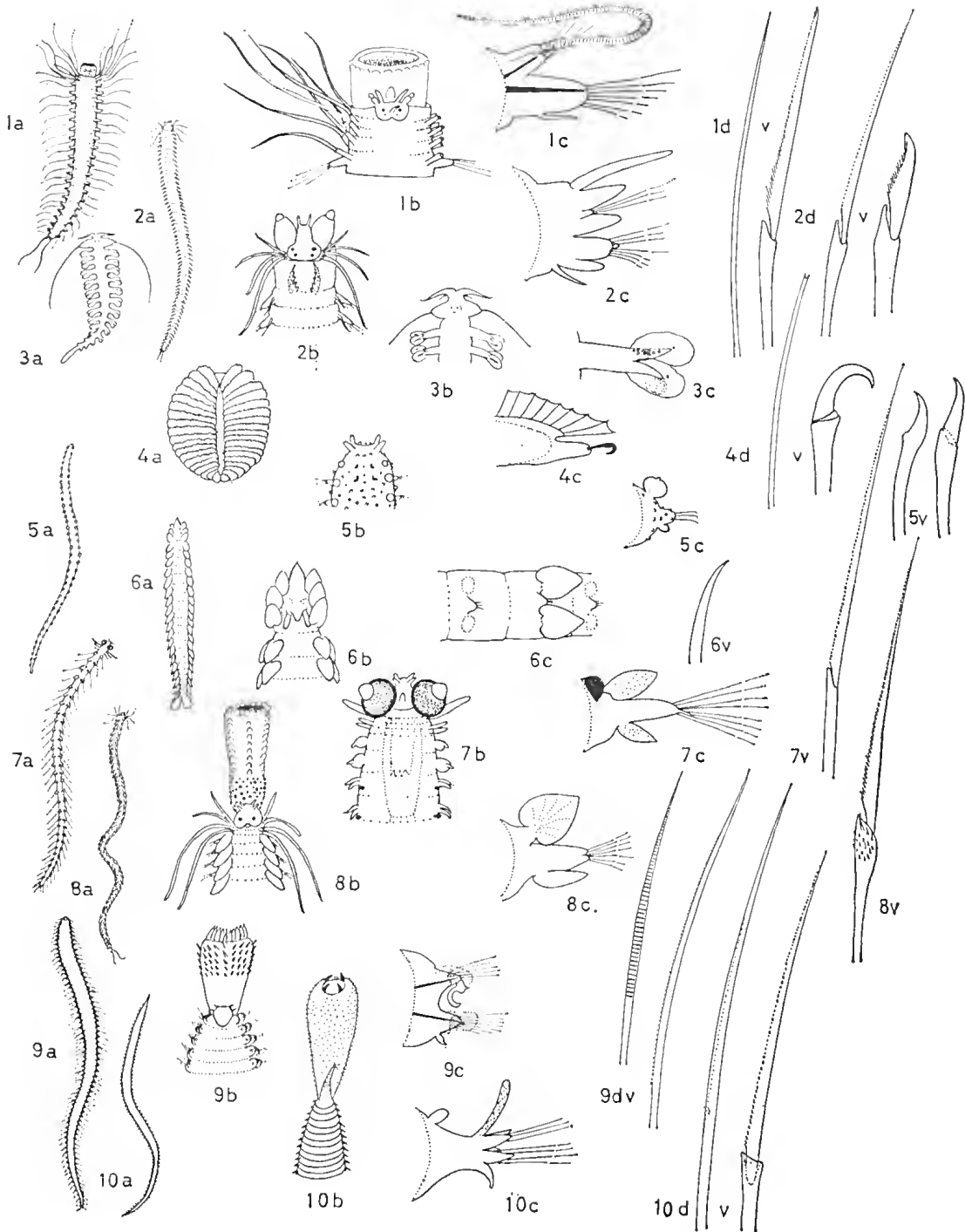
FIG. 0.3. Illustrations of Family Characters. 1, Hesionidae. 2, Nereidae. 3, Tomopteridae. 4, Sphinteridae. 5, Sphaerodoridae. 6, Typhloscolecidae. 7, Alciopidae. 8, Phyllococidae. 9, Nephtyidae. 10, Glyceridae. (A) Entire worm. (B) Head. (C) Foot. (D) Notoseta. (v) Neuroseta or seta of uniramous parapodium.
