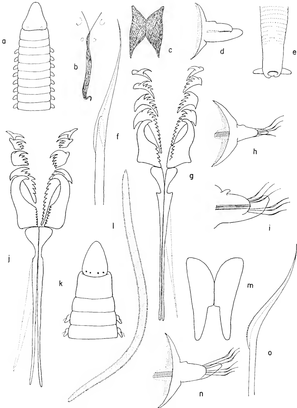
FIG. 17.18. Drilognathus capensis . (A) Head. (B) Vestiges of maxillae. (C) Mandibles. (D) Foot. (E) Posterior end. Arabella mutans . (F) Hooded acicular seta. (G) Maxillae. (H) Foot. Arabella iricolor . (I) Foot with dorsal cirrus. (J) Maxillae. (K) Head. (L) Entire worm (natural size). (M) Mandibles. Arabella iricolor caerulea . (N) Foot. (O) Winged capillary.
