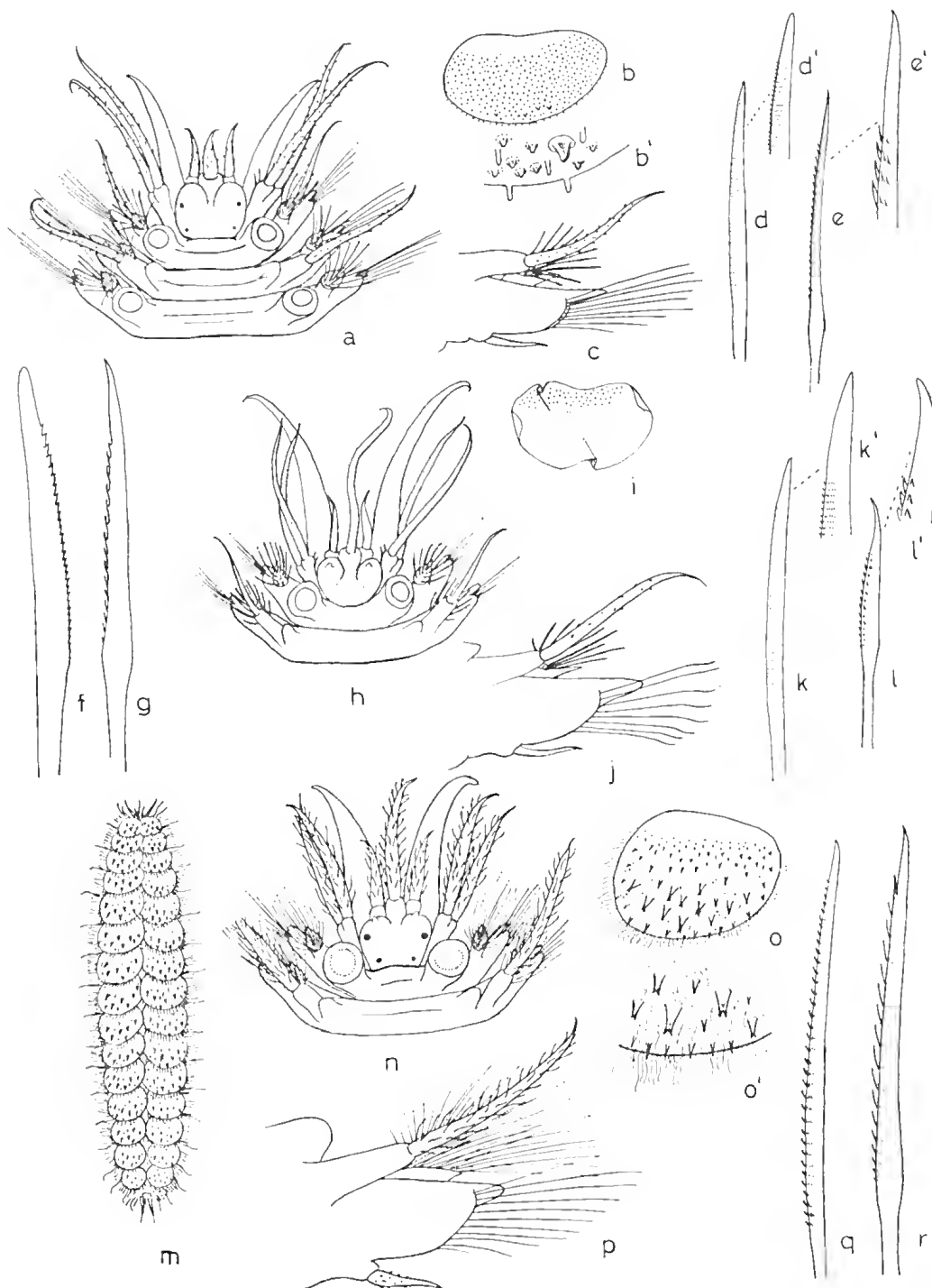
FIG. 1.8. Eunoe nodulosa . (A) Head. (B, B 1 ) Elytron and details of margin. (C) Foot. (D) Notoseta. (E) Neuroseta. Eunoe macrophthalmma (after McIntosh, 1925). (F) Notoseta. (G) Neuroseta. Eunoe assimilis . (H) Head. (I) Elytron. (J) Foot. (K) Notoseta. (L) Neuroseta. Harmothoe dictyophora . (M) Entire worm (twice life size). (N) Head. (O, O 1 ) Elytron and details of tubercles. (P) Foot. (Q) Notoseta. (R) Neuroseta.
