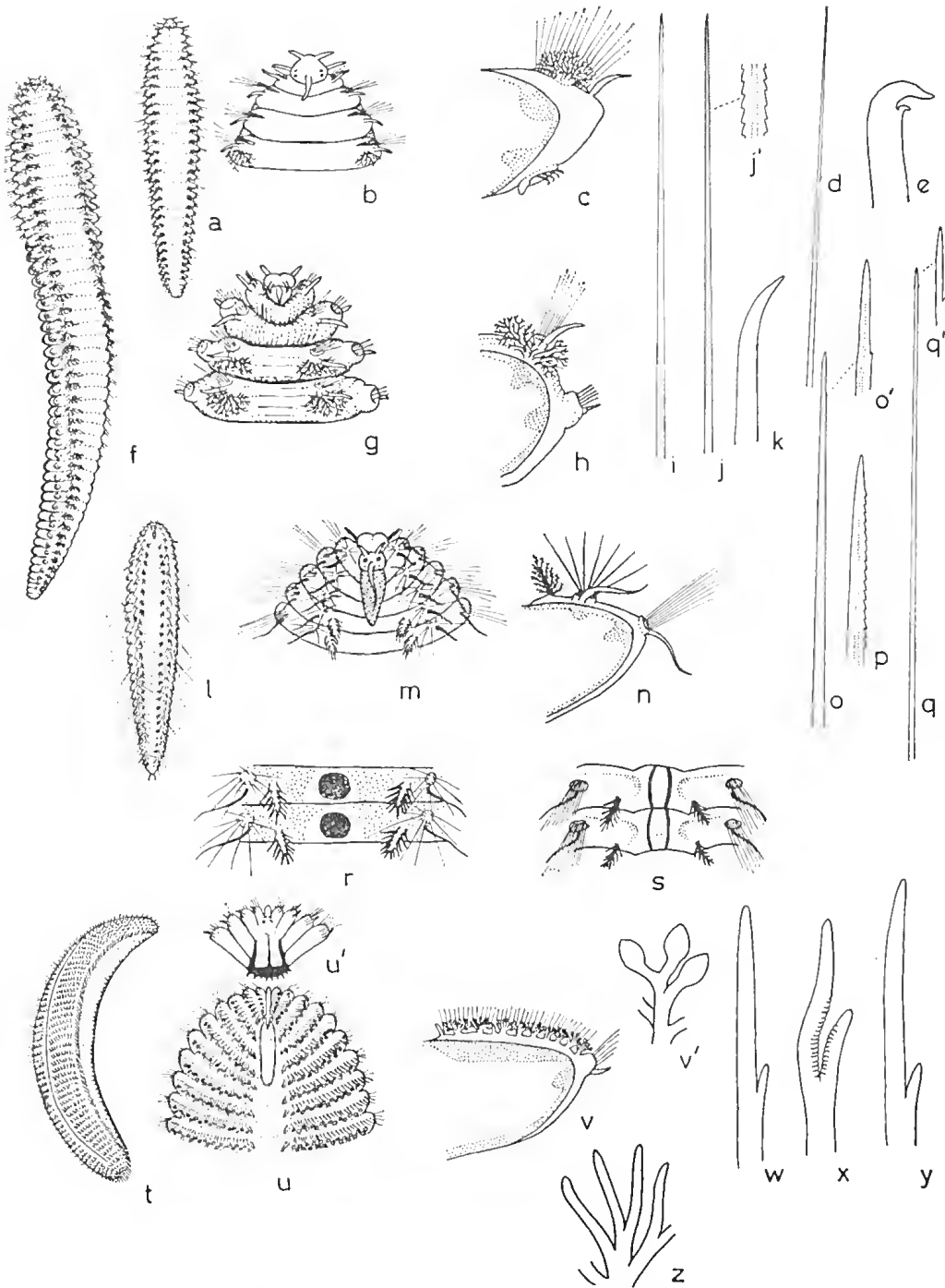
FIG. 3.1. Hippoona gaudichaudi agulhana . (A) Entire worm (twice natural size). (B) Head. (C) Posterior view of foot. (D) Notoseta. (E) Neuropodial hook. Amphinome rostrata . (F) Entire worm (half natural size). (G) Head. (H) Posterior view of foot. (I) Notopodial capillary. (J) Harpoonseta. (K) Neuroseta. Chloecia inermis . (L) Entire worm (natural size). (M) Head. (N) Foot. (O) Notoseta. (P) Tip of harpoon seta. (Q) Neuroseta. Chloecia flava . (R) Dorsal view of two segments showing pigment pattern (after Horst). Chloecia fusca . (S) Dorsal view of two segments showing pigment pattern (after Horst). Euphrosine capensis . (T) Lateral view of entire worm (1.5 times natural size). (U) Head. (U 1 ) Ventral view of head. (V) Foot. (V 1 ) Enlarged view of tips of gill filaments. (W) Spurred notoseta. (X) Ringent notoseta. (Y) Neuroseta. Euphrosine myrtilosa . (Z) Enlarged view of tips of gill filaments.
