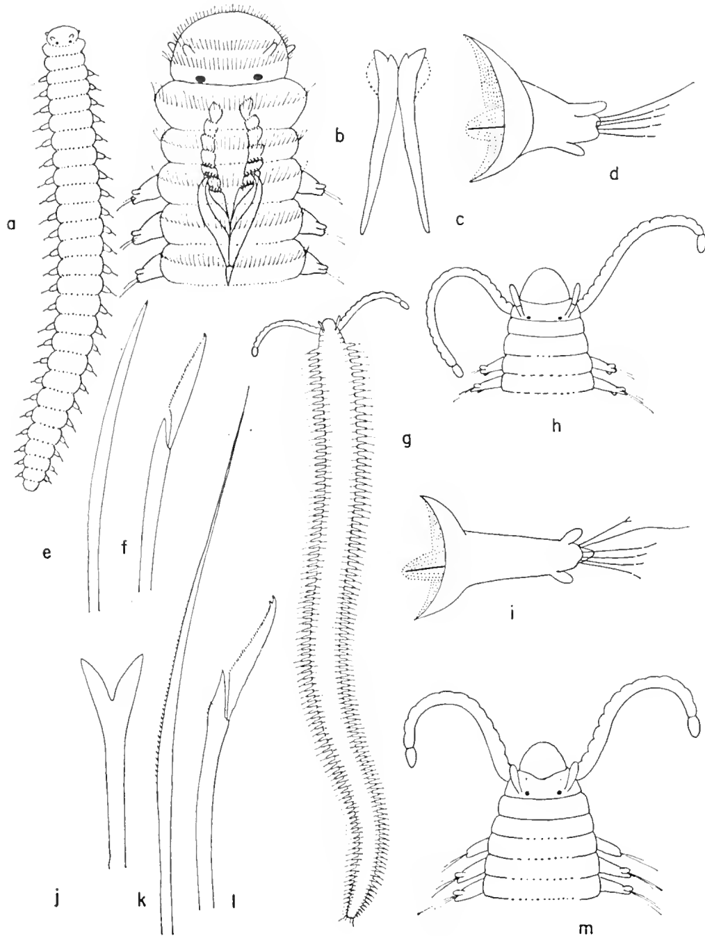
FIG. 17.20. Ophryotrocha puerilis . (A) Entire worm (16 times life size). (B) Head. (C) Mandibles. (D) Foot. (E) Superior simple seta. (F) Inferior compound seta. Protodorvillea biarticulata . (G) Entire worm (16 times life size). (H) Head. (I) Foot. (J) Forked seta. (K) Superior capillary seta. (L) Falcigerous seta. Protodorvillea egena . (M) Head.
