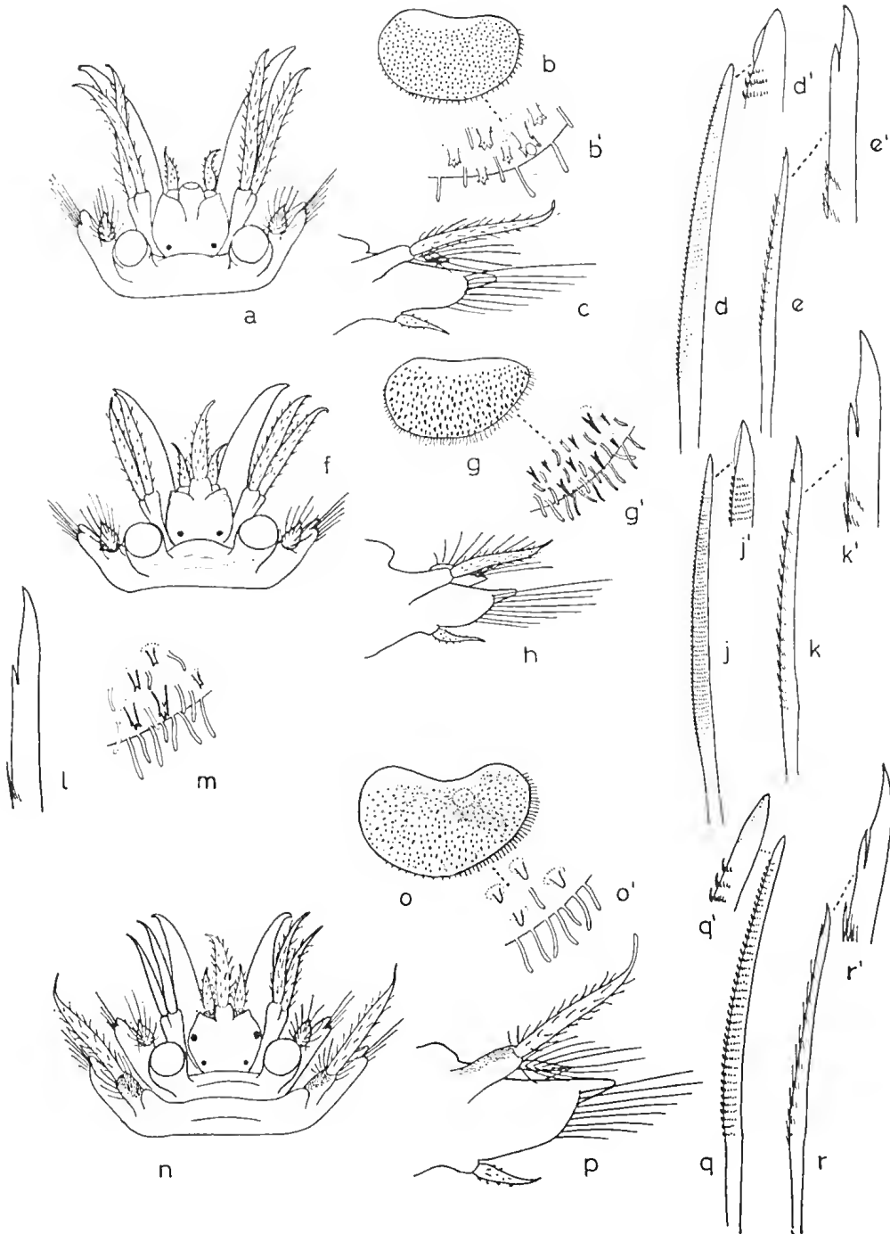
FIG. 1.9. Harmothoe antilopis . (A) Head. (B, B 1 ) Elytron and details of tubercles. (C) Foot. (D, D 1 ) Notoseta. (E, E 1 ) Neuroseta. Harmothoe aquiseta . (F) Head. (G, G 1 ) Elytron and details of tubercles. (H) Foot. (J, J 1 ) Notoseta. (K, K 1 ) Neuroseta. Harmothoe aquiseta africana . (L) Tip of neuroseta. (M) Details of tubercles on elytron. Harmothoe gorceensis . (N) Head. (O, O 1 ) Elytron and details of tubercles. (P) Foot. (Q, Q 1 ) Notoseta. (R, R 1 ) Neuroseta.
