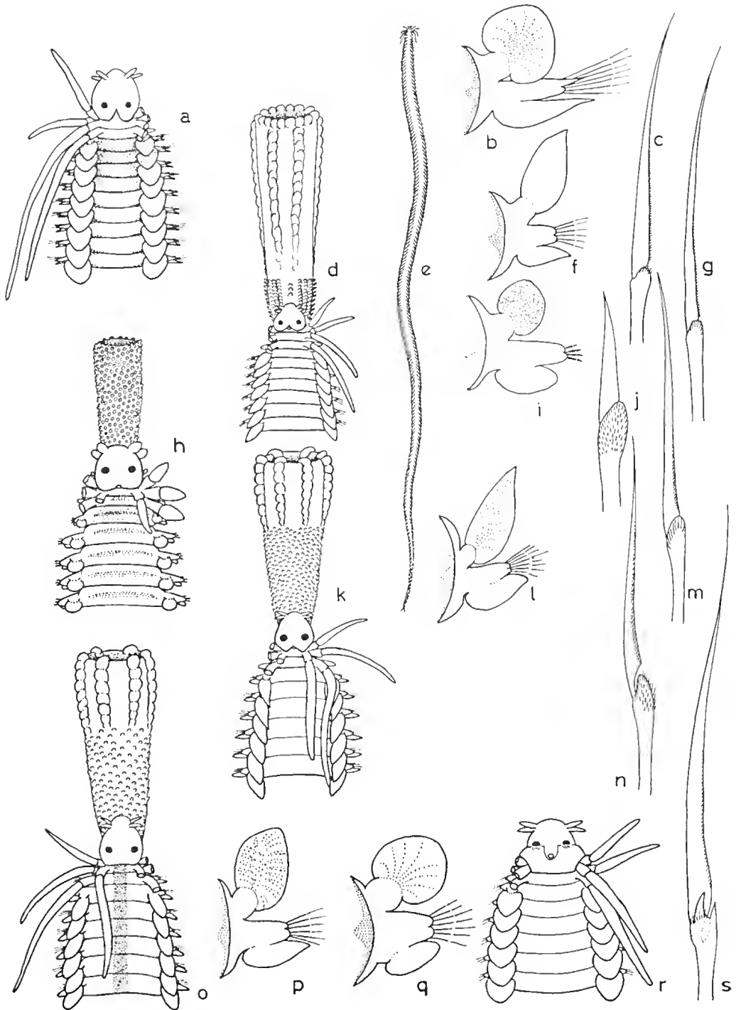
FIG. 5.2. Phyllodoce longipes . (A) Head. (B) Foot. (C) Seta. Phyllodoce madeirensis . (D) Head and everted proboscis. (E) Entire worm (natural size). (F) Foot. (G) Seta. Phyllodoce quadraticeps . (H) Head with proboscis partly everted. (I) Foot. (J) Seta. Phyllodoce fristedti . (K) Head with proboscis partly everted. (L) Anterior foot. (M) Seta. Phyllodoce malmgreni . (N) Seta. (O) Head with proboscis partly everted. (P) Foot. Phyllodoce capensis . (Q) Foot. (R) Head. (S) Seta.
