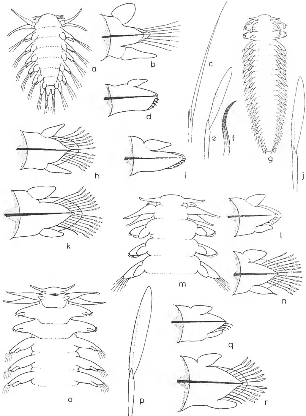
FIG. 5.6. Pedinosoma curtum . (A) Entire worm (20 times natural size). (B) Posterior view of foot. (C) Seta. Lopadorhynchus uncinatus (modified from Fauvel, 1915). (D) Second foot. (E) Compound seta. (F) Simple hook from second foot. (G) Entire worm (dorsal view, three times natural size). (H) Tenth foot. Lopadorhynchus krohni . (I) Second foot. (J) Compound seta. (K) Seventh foot. Lopadorhynchus appendiculatus . (L) Second foot. (M) Dorsal view of anterior end. (N) Tenth foot. Lopadorhynchus henseni . (O) Ventral view of anterior end. (P) Compound seta. (Q) Second foot. (R) Seventh foot.
