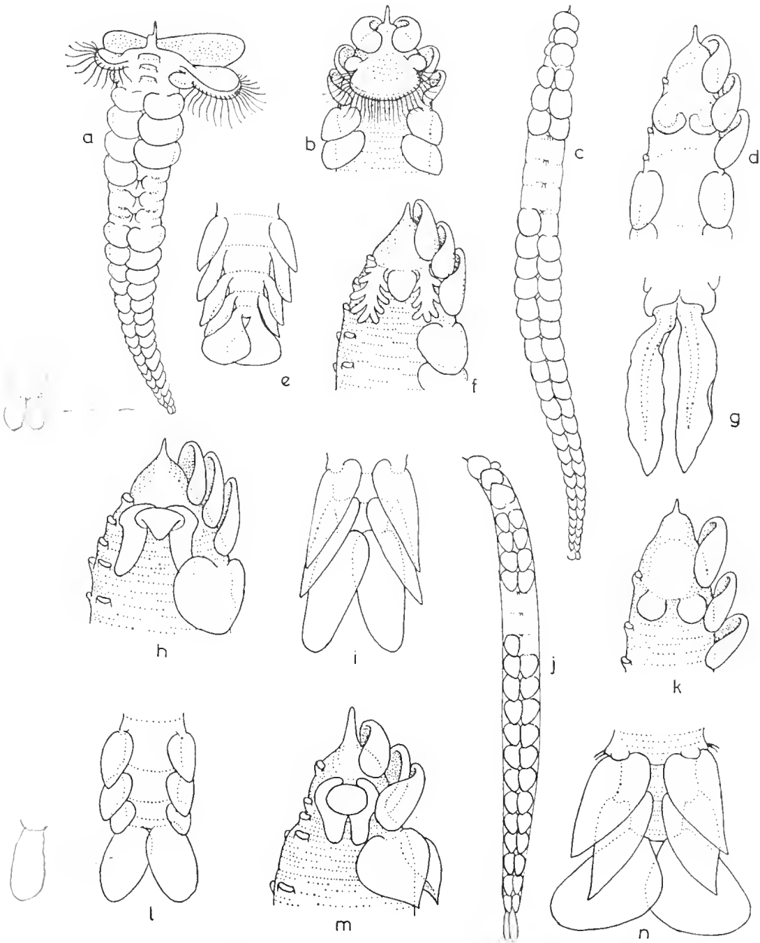
FIG. 9.1. Typhloscolex muelleri . (A) Lateral view of entire worm (25 times life size). (B) Dorsal view of head. Sagitella kowalevskii . (C) Lateral view of entire worm (eight times life size). (D) Dorsal view of head. (E) Tail end. Travisioopsis coniceps (after Monro, 1936, fig. 16.B). (F) Dorsal view of head. (G) Tail end. Travisioopsis lanceolata . (H) Dorsal view of head. (I) Tail end. Travisioopsis dubia . (J) Lateral view of entire worm (14 times life size). (K) Dorsal view of head. (L) Tail end. Travisioopsis lobifera . (M) Dorsal view of head. (N) Tail end.
