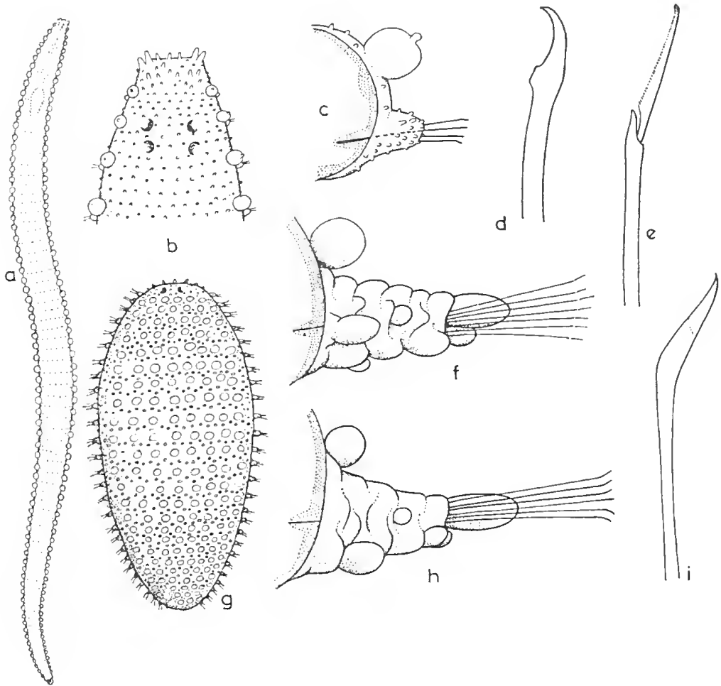
FIG. 13.1. Sphaerodorum gracile . (A) Entire worm (five times life size). (B) Head (after Fauvel). (C) Parapodium. (D) Seta. Sphaerodoridium benguelarum . (E) Seta. (F) Parapodium. (G) Entire worm (25 times life size). Sphaerodoridium capense . (H) Parapodium. (I) Seta.
