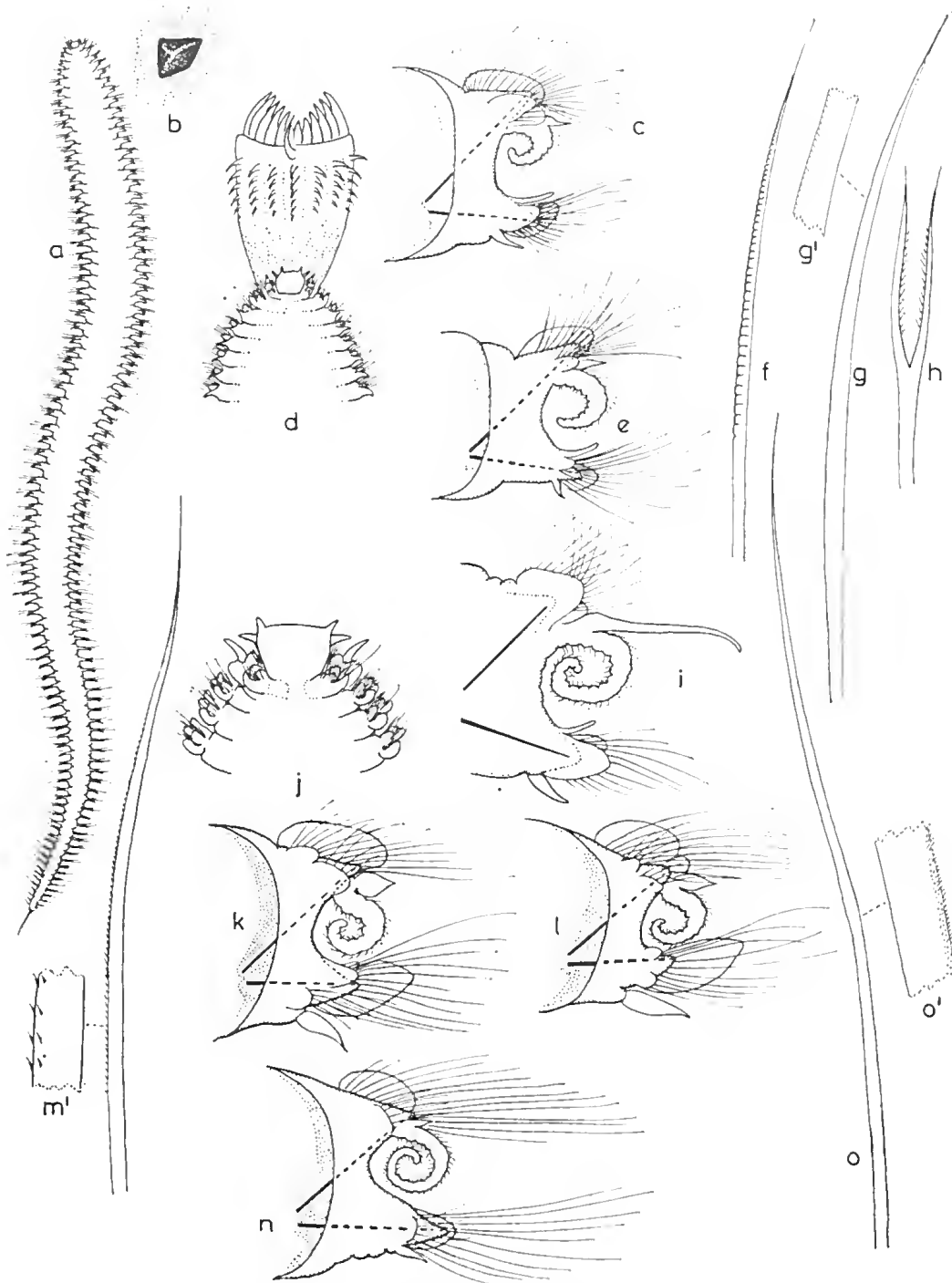
FIG. 15.1. Nephtys dibranthis . (A) Entire worm (five times life size). (B) Chitinous jaw. (C) Twelfth foot. (D) Head with proboscis extruded. (E) Middle foot. (F) Laddered pre-acicular seta. (G) Post-acicular seta. (H) Forked seta. Nephtys lyrochaeta . (I) Thirty-fifth foot (from Monro, 1936). Nephtys macroua . (J) Head. (K) Anterior foot. (L) Middle foot. (M) Post-acicular seta. Nephtys malmgreni . (N) Middle foot. (O) Post-acicular seta.
