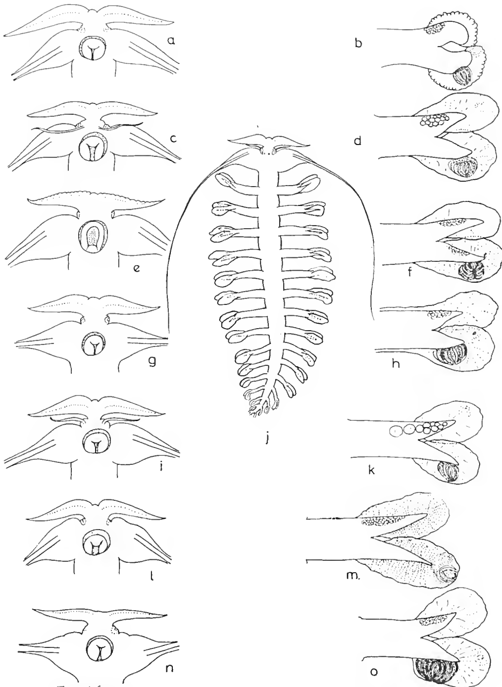
FIG. 8.2. Euahteris Tomopteris euchaeta . (A) Head. (B) Fifth foot. Tomopteris krampi . (C) Head. (D) Fifth foot. Tomopteris carpenteri . (E) Head. (F) Fifth foot. Tomopteris ligulata . (G) Head. (H) Fifth foot. Tomopteris elegans . (I) Head. (J) Entire worm (six times life size). (K) Fourth foot. Tomopteris septentrionalis . (L) Head. (M) Fifth foot. Tomopteris planktonis . (N) Head. (O) Fifth foot.
