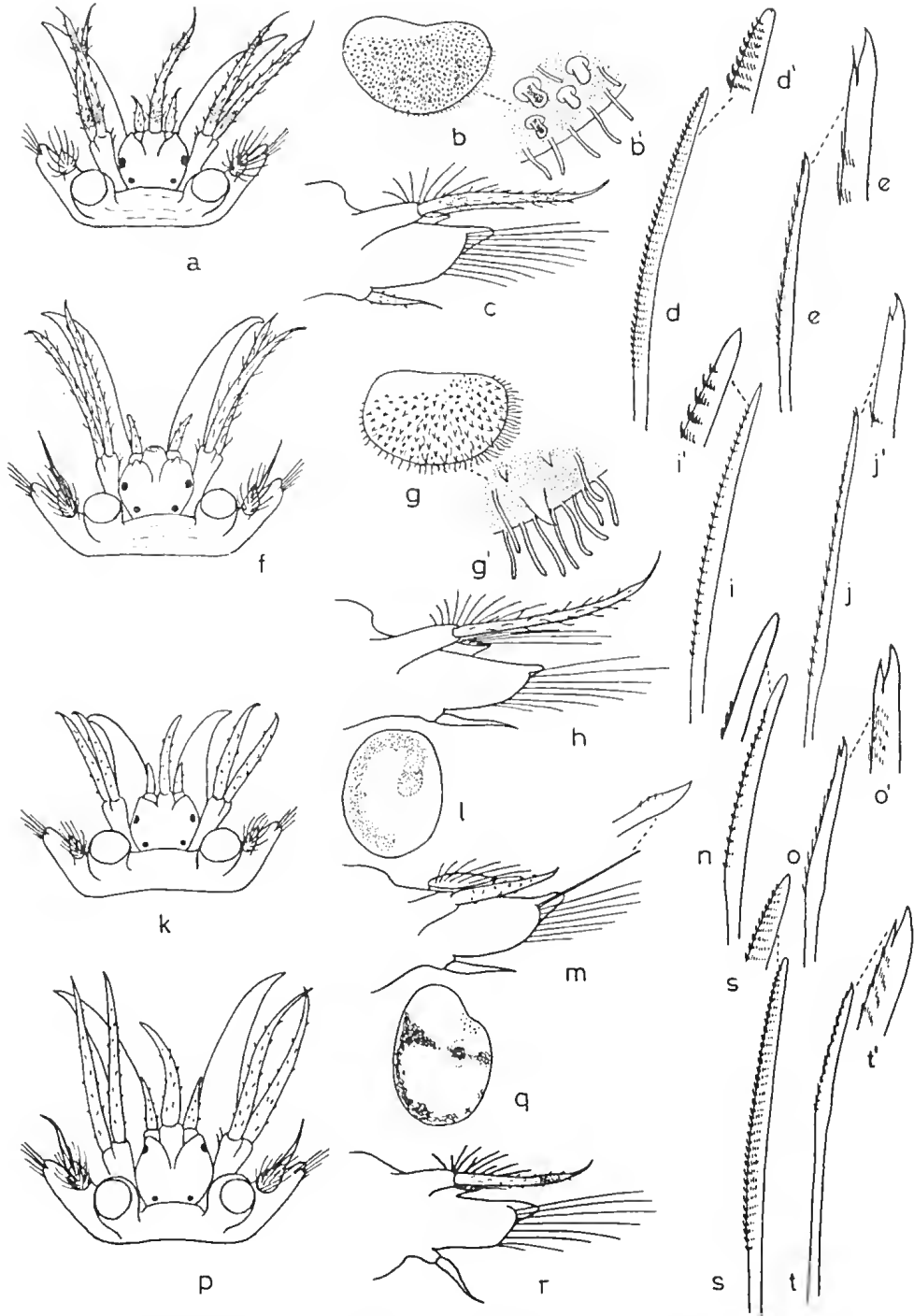
FIG. 1.10. Harmothoe gilchristi . (A) Head. (B, B 1 ) Elytron and details of tubercles. (C) Foot. (D) Notoseta. (E) Neuroseta. Harmothoe lagiscoides serrata . (F) Head. (G, G 1 ) Elytron and details of tubercles. (H) Foot. (I) Notoseta. (J) Neuroseta. Harmothoe saldanha . (K) Head. (L) Elytron. (M) Foot. (N) Notoseta. (O) Neuroseta. Harmothoe lunulata . (P) head. (Q) Elytron. (R) Foot. (S) Notoseta. (T) Neuroseta.
