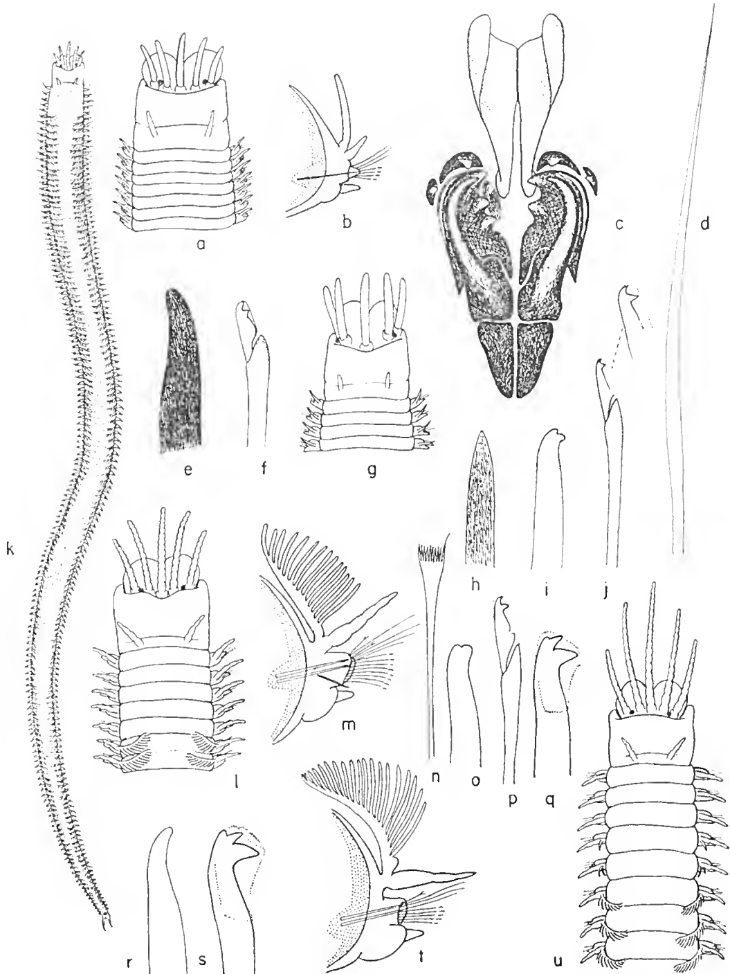
FIG. 17.2. Eunice siciliensis . (A) Head. (B) Eightieth foot. (C) Jaws. (D) Simple capillary seta. (E) End of aciculum. (F) Compound seta. Eunice cincta . (G) Head. (H) End of aciculum. (I) Acicular seta. (J) Compound seta. Eunice antennata . (K) Entire worm (1.5 times life size). (L) Anterior end. (M) Thirty-fifth foot. (N) Comb seta. (O) Tip of aciculum. (P) Compound seta. (Q) Acicular seta. Eunice australis . (R) Tip of aciculum. (S) Acicular seta. (T) Twenty-fifth foot. (U) Anterior end.
