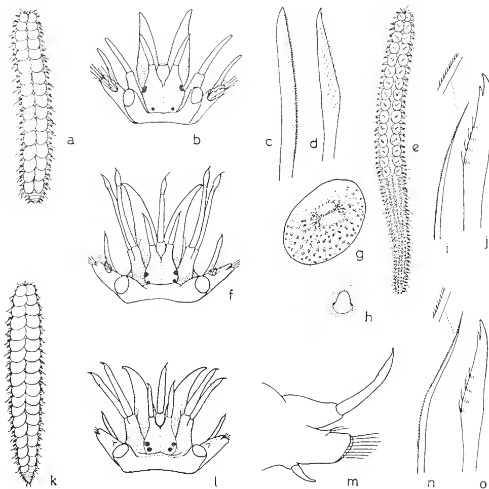
FIG. 1.15. Parahalosydna capensis . (A) Entire worm (twice natural size). (B) Head. (C) Noto-seta. (D) Neuroseta (after McIntosh). Pseudopolynoe inhaca . (E) Entire worm (1.5 times natural size). (F) Head. (G) Elytron. (H) Elytrous tubercle. (I) Noto-seta. (J) Neuroseta. Halosydna alleni . (K) Entire worm (twice natural size). (L) Head. (M) Anterior view of foot. (N) Noto-seta. (O) Neuroseta.
