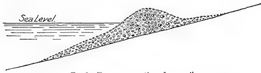
FIG. 5.—Transverse section of sea wall.
