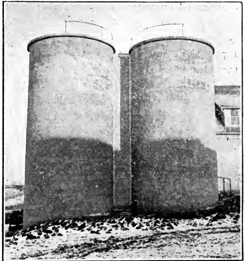
Twin Concrete Silos on farm of Frank White, La Fox, Ill., each 18x45 feet. Built by Polk System. W. H. Warford, Geneva, Ill., Contractor.
