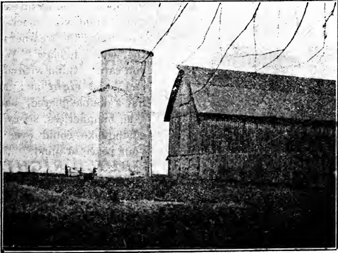
Silo of Mr. C. W. Broughton, McGirr, Ill., diameter 16 feet, height 45 feet. Built by Polk System.
