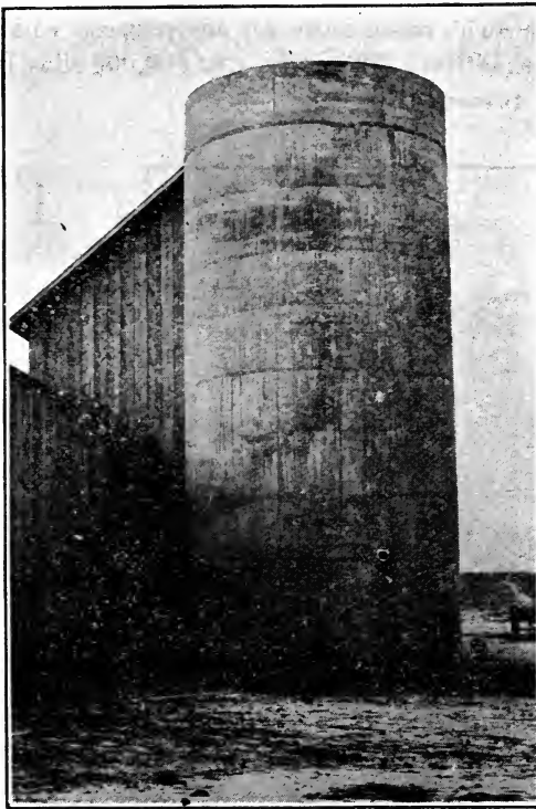
Silo of George Dick, Sycamore, Ill., Size: Diameter 16 feet, Height 40 feet. Polk System
