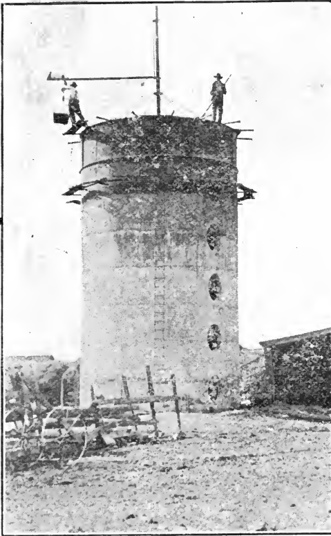
18 x 45 feet Silo under construction. P. A. Qvanstrong, Genoa, Illinois, Contractor. Polk System.
