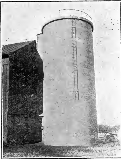
C. A. Baber's Monolithic Silo, LaFox, Illinois. Diameter 18 feet, height 45 feet. Polk System. W. H. Warford, Geneva, Illinois, Contractor.
