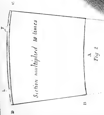
Diagram for the Essay on the Crust of the Earth.
