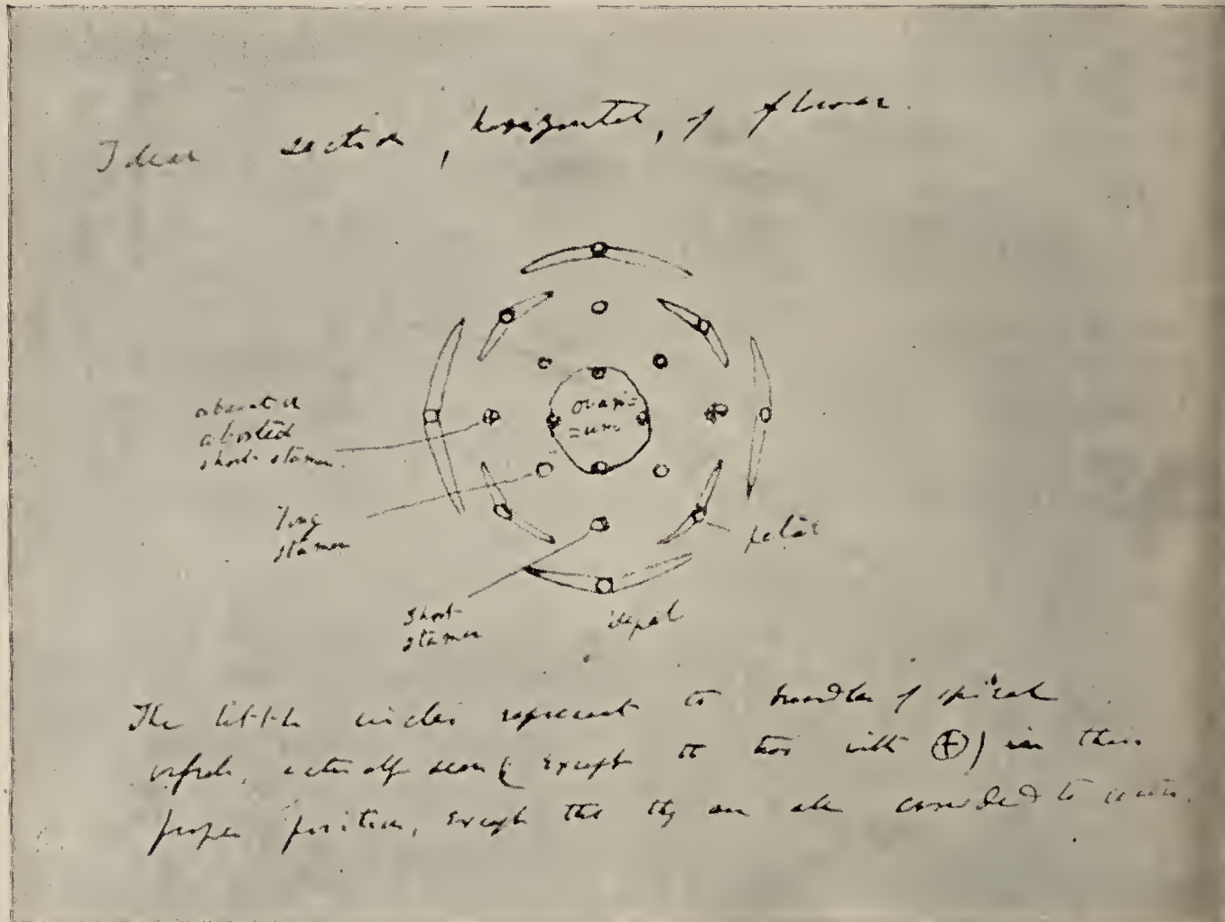
Fig. 10.—DIAGRAM OF CRUCIFEROUS FLOWER.
