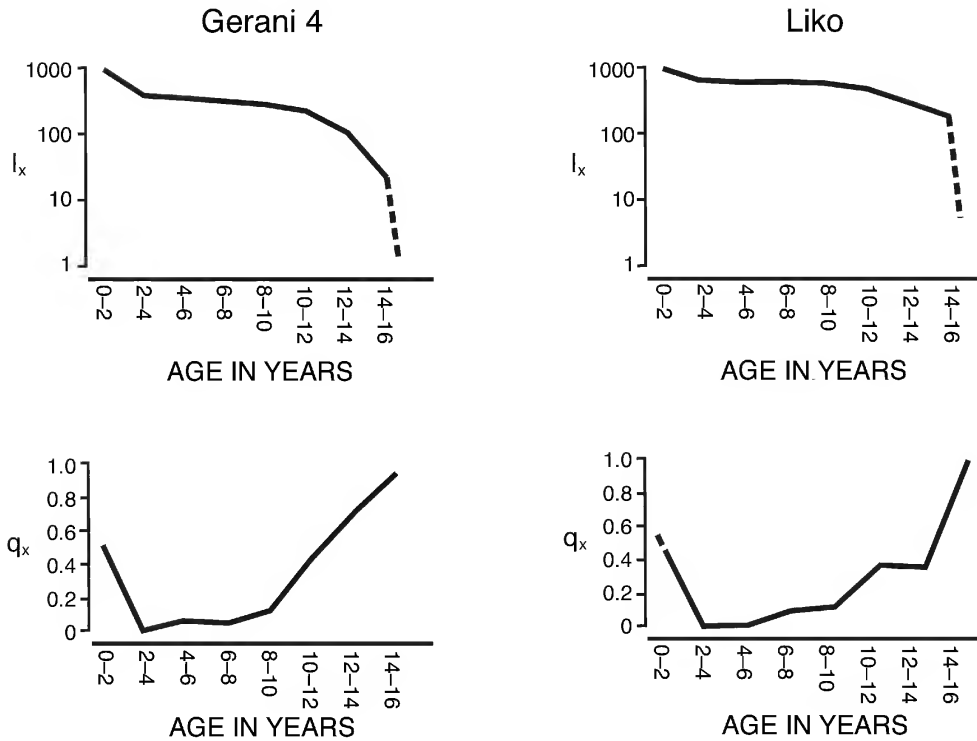
FIG. 7. Survivorship curves ( l_x ) and mortality rates ( q_x ) (top and bottom, respectively) for Candiaceervus ropalophorus (Gerani 4) and Candiaceervus sp. II (Liko).
