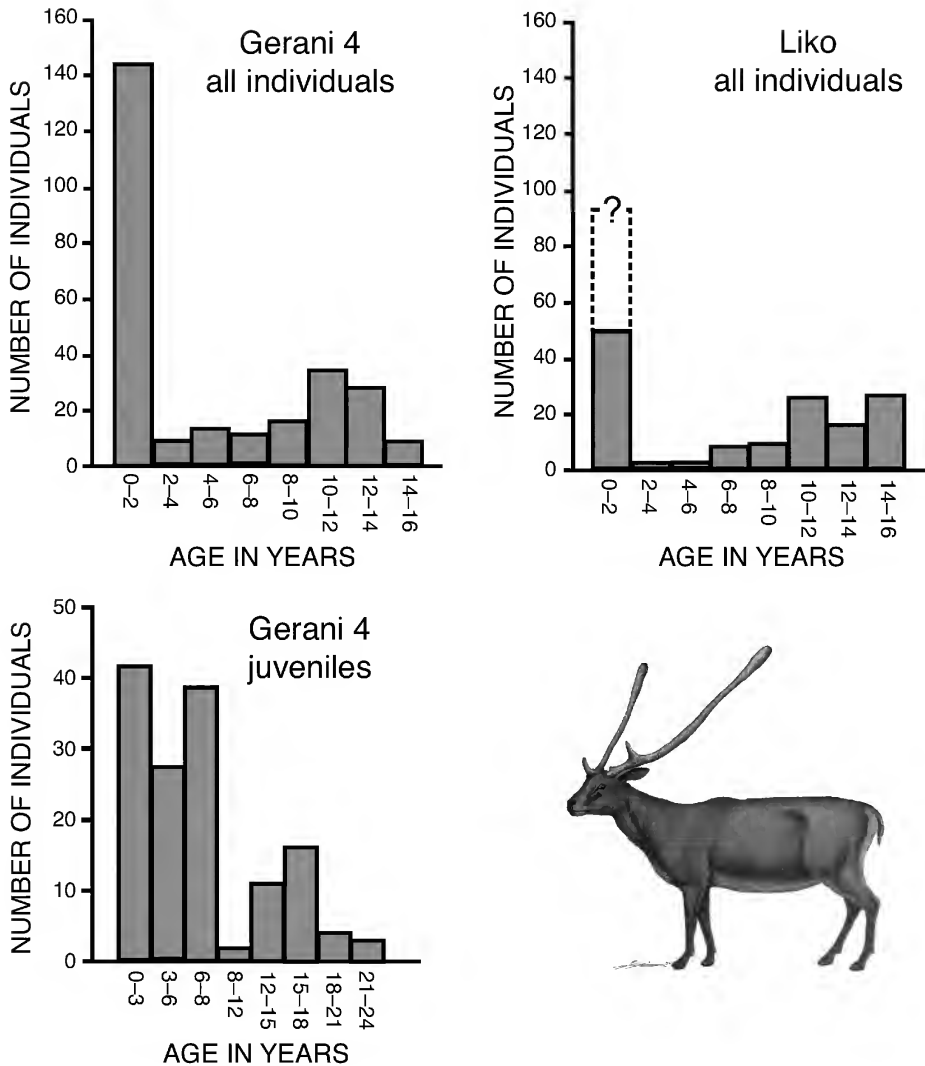
FIG. 6. Mortality profiles (dx) for Candiacevurus ropalophorus from Gerani 4 (top left, actual numbers for all ages; bottom left, juveniles only) and Candiacevurus sp. II from Liko (top right, all ages). Bottom right, reconstruction of Can. ropalophorus by Alexis Vlachos.
