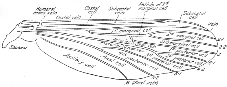
FIGURE 16.—Wing of mosquito (Howard, Dyar, and Knab). The corresponding symbols for the veins in the Comstock-Needham system are: 1, R ; 2.1 and 2.2, R 2 and R 3 ; 3, R 4+5 ; 4.1, M 1+2 ; 4.2, M 3 ; 5.1 and 5.2, Cu 1 and Cu 2 ; anterior cross vein, r-m ; posterior (basal) cross vein, m-cu .
