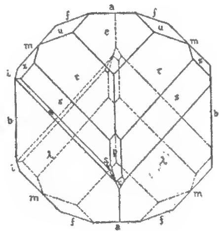
Figure 6. Diopside, colourless crystal from Montreal chrome pit; orthographic projection of one of the measured crystals, showing two of the new forms, s. (\bar{5}34) and r. (15\cdot4\cdot10) .
