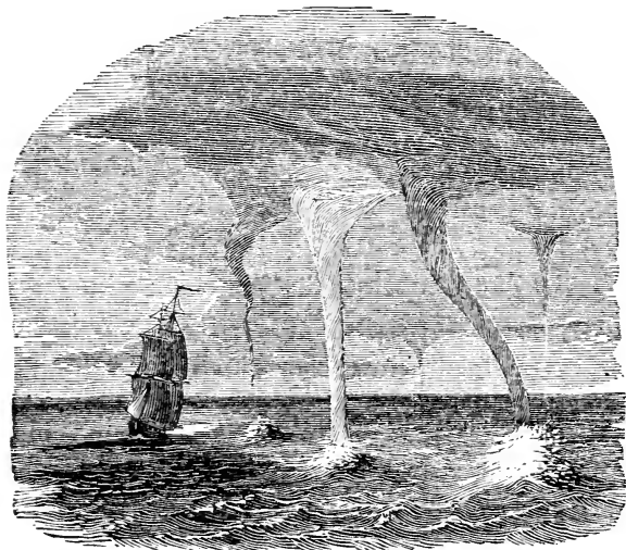
WATERSPOUTS.
