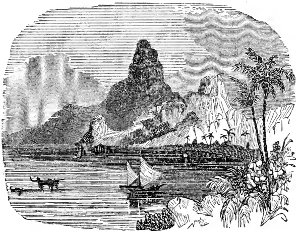
VOLCANIC ISLANDS.
