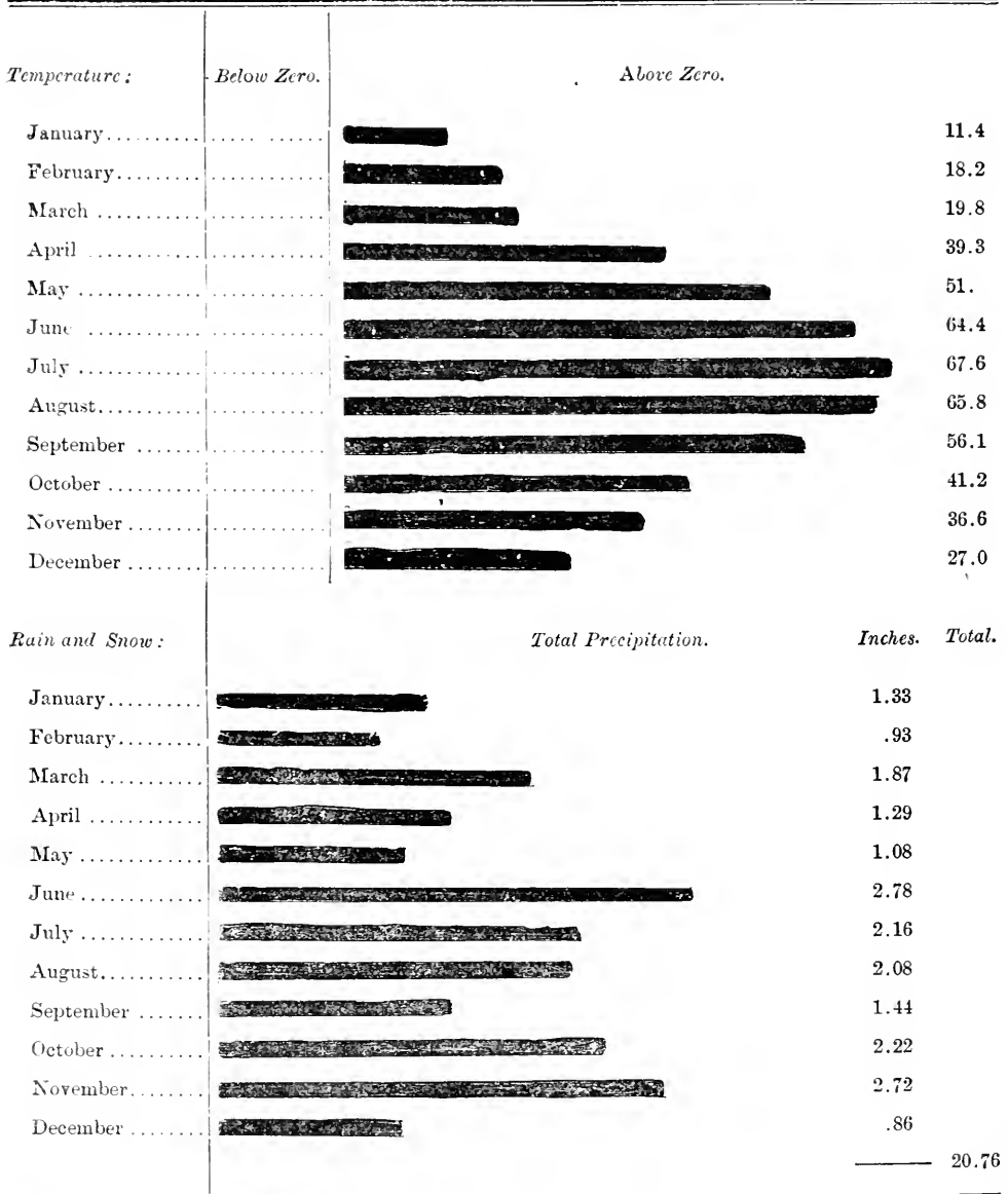
DIAGRAM ILLUSTRATING THE MEAN METEOROLOGICAL RESULTS FOR 1888.
