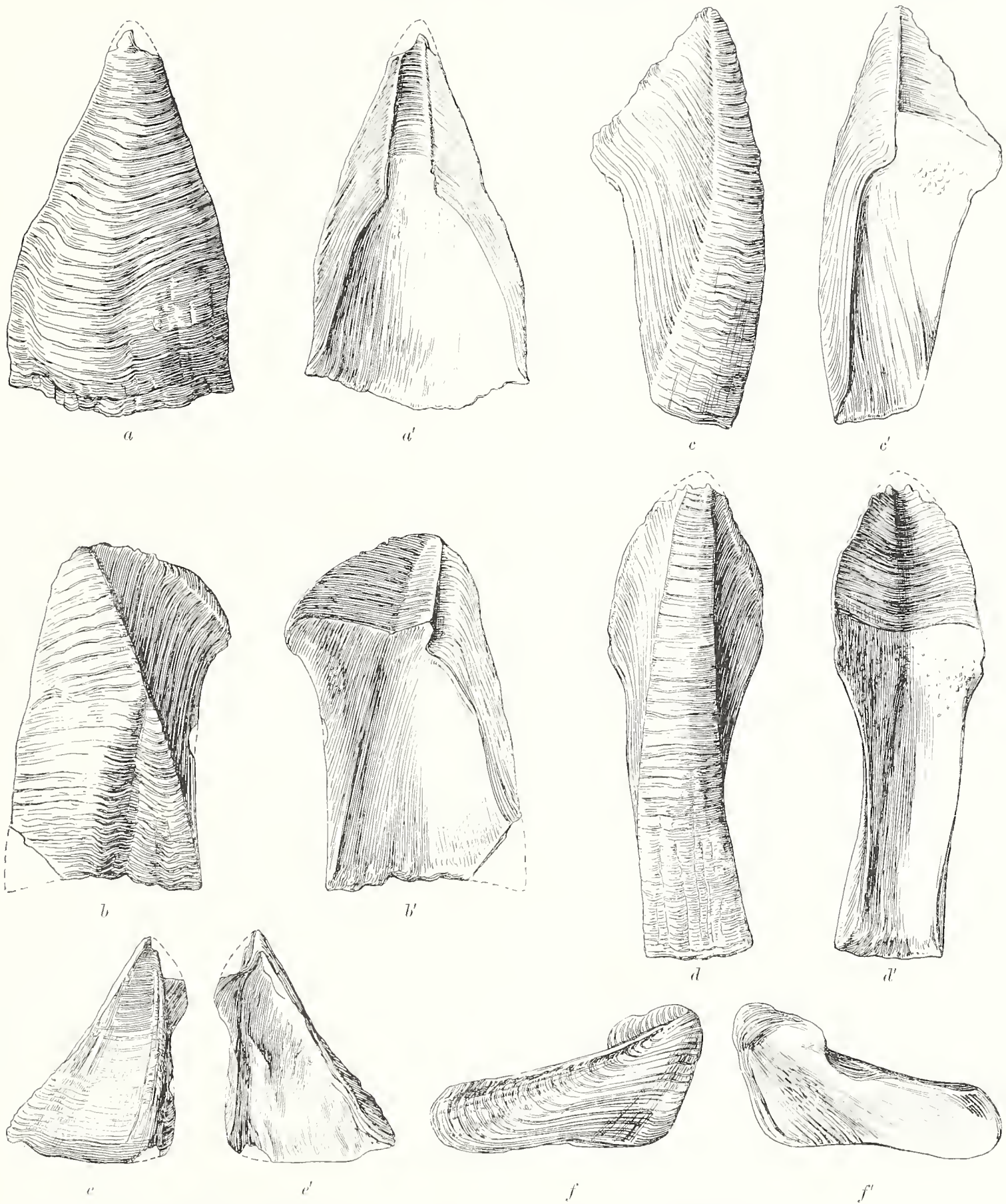
FIG. 7.— Hexclasma antarcticum , n. sp., nat. size. a, a' , external and internal views of rostrum; b, b' , the same of lateral; c, c' , the same of carino-lateral; d, d' , the same of carina; e, e' , the same of tergum; f, f' , the same of scutum. The valves figured are the most perfect specimens collected; they do not belong to the same individual.
