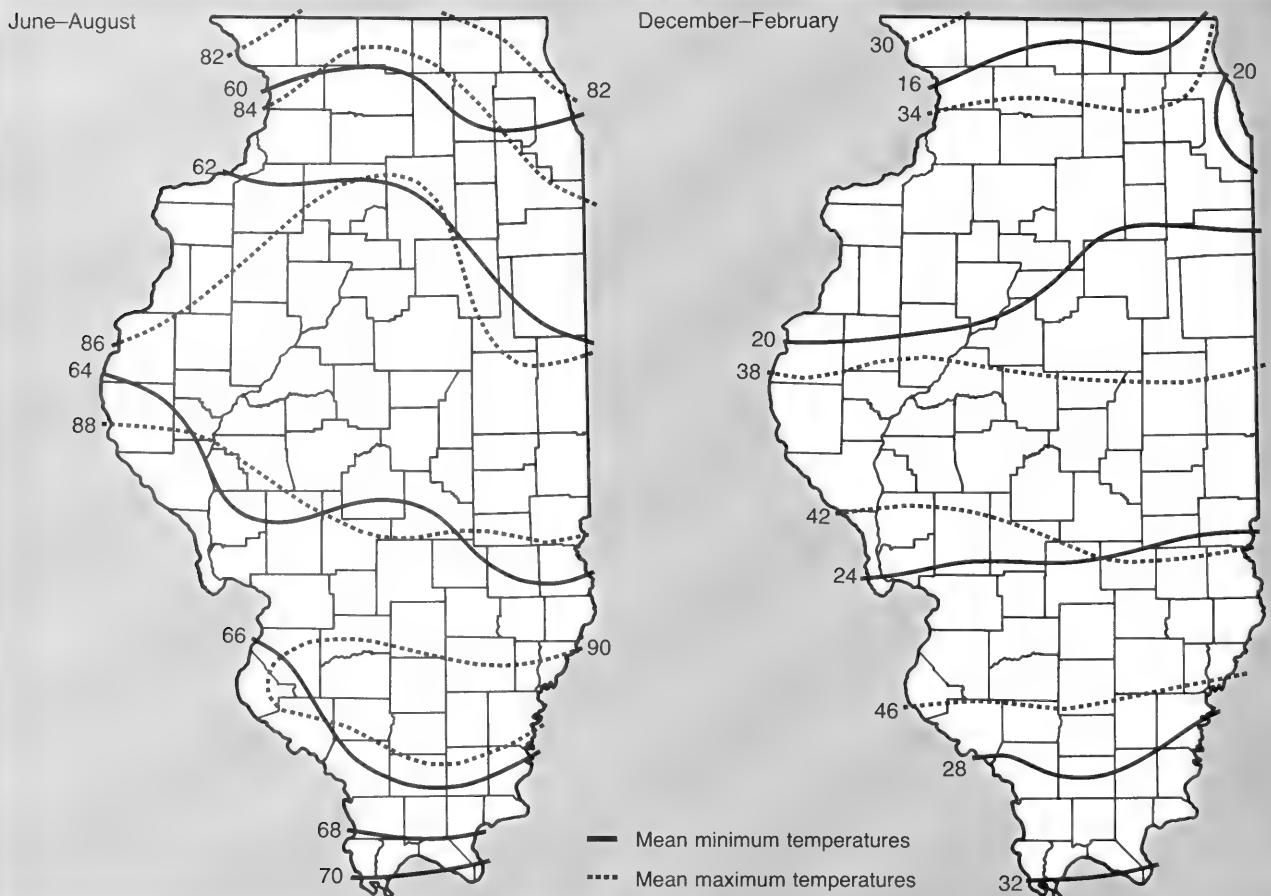
Figure 4. Mean maximum and minimum temperatures (in degrees Fahrenheit) in summer and winter. Source: Illinois Technical Advisory Committee on Water Resources 1967.
