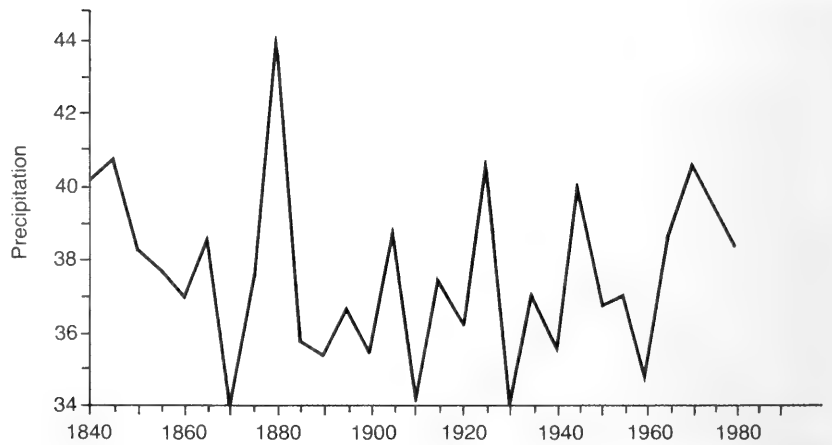
Figure 2. Five-year precipitation means (in inches) for Illinois. Source: Illinois State Water Survey.
