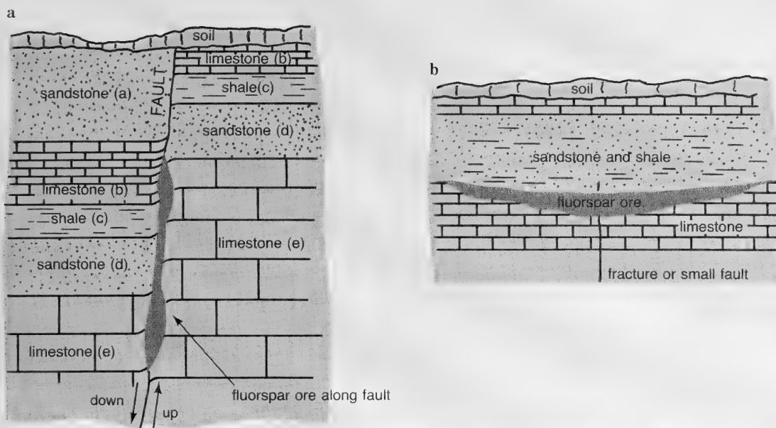
Figure 6. Cross sections showing the occurrence of fluorspar: a. vein deposit of fluorspar ore along a vertical fault and b. horizontal bedded-replacement of fluorspar ore. Source: Lamar 1965; Bradbury et al. 1968.
