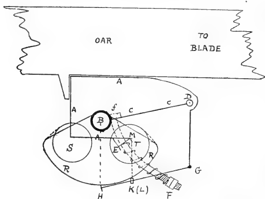
Fig. 1. Diagram illustrating action of Pencil and Spring.
