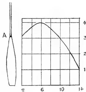
Fig. 9. Position of 'Turning Point' on Oar during the Stroke.
