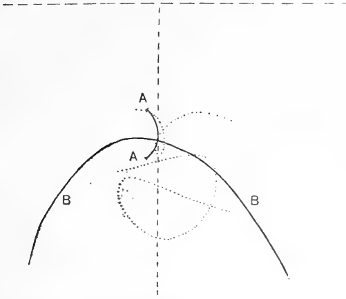
Fig. 8. Motion in space of Instantaneous Centre ( B ) and 'Turning Point' ( A ).
