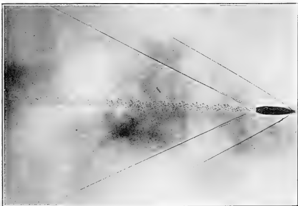
FIG. 4.—30 Calibre boat-tailed bullet, approximate speed 2500 feet per second.
