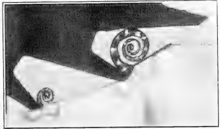
FIG. 4.—Steel milling cutter operating on a plate of nitro-cellulose.
