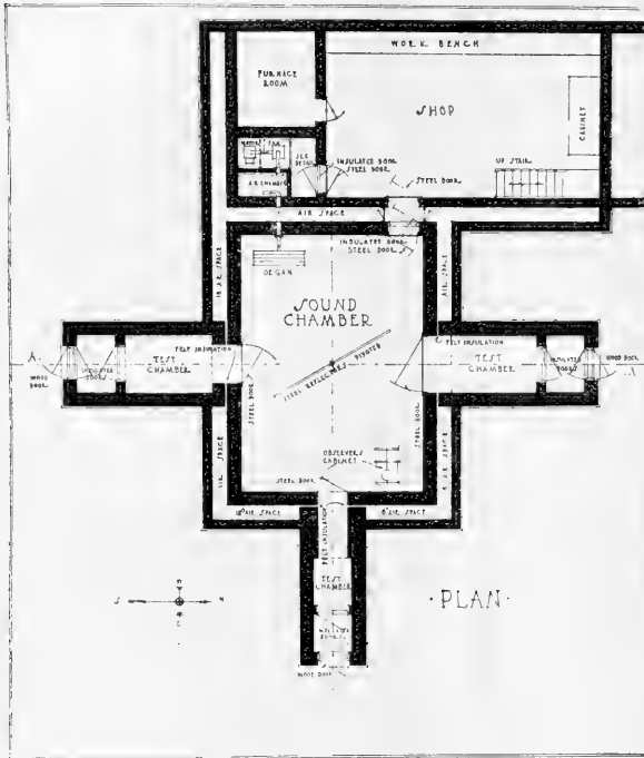
FIG. 1.—Plan of Acoustic Research Building.
