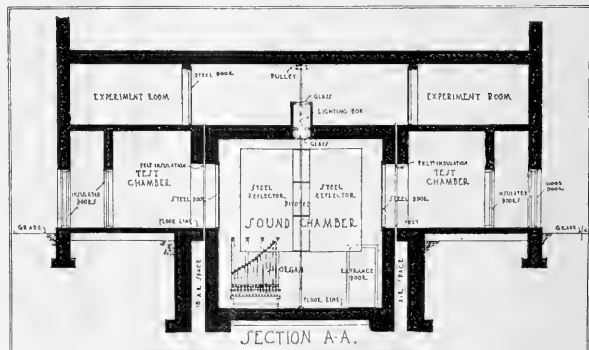
FIG. 2.—Section A-A of Acoustic Research Building.
